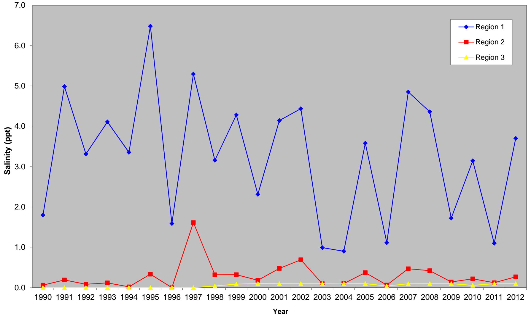
Delaware River Average Salinity
