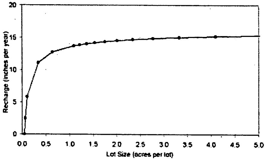
Figure 4. Graph relating to lot size. (Calculated using the recharge methodology of Charles and others, 1993. This example is for a Rockaway soil in Rockaway Township, Morris County.)
