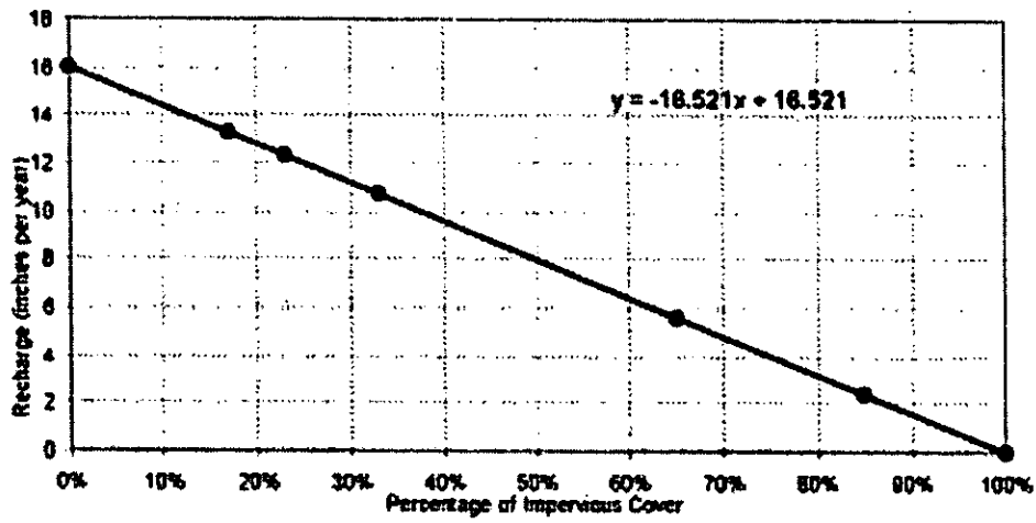
Figure 3. Example of recharge as a function of impervious cover. (Calculated using the recharge methodology of Charles and others, 1993)
