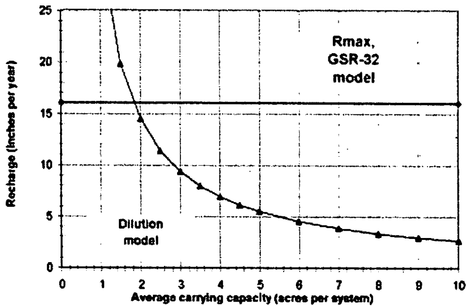
Figure 5. Recharge values estimated by the nitrate-dilution and recharge methodologies.
