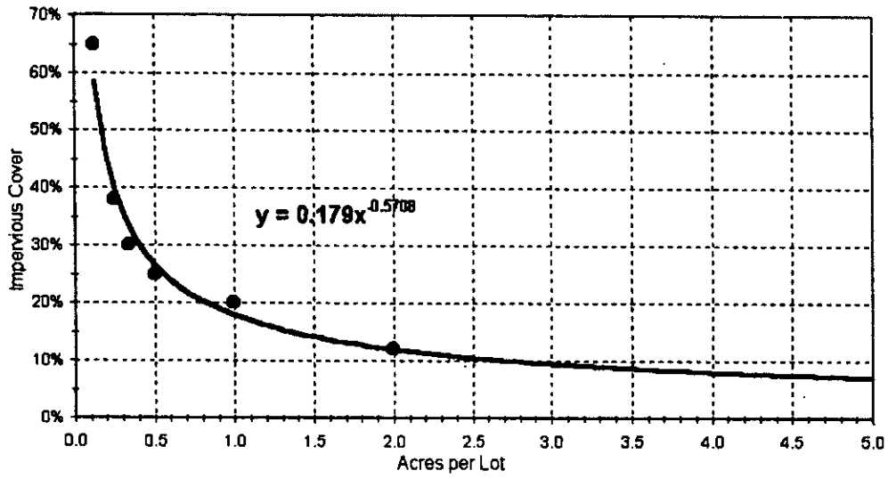
Figure 1. Relation between percentage of impervious land cover and housing density. Points depict U.S. Department of Agriculture (1986) data. Curve is best fit power series line for the data set.
