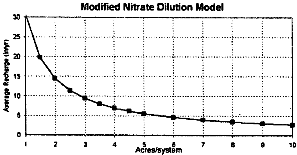
Figure 2. Example of modified Trela-Douglas nitrate-dilution model. Assumptions: 3 people per home, 10 pounds nitrate per person per year.
