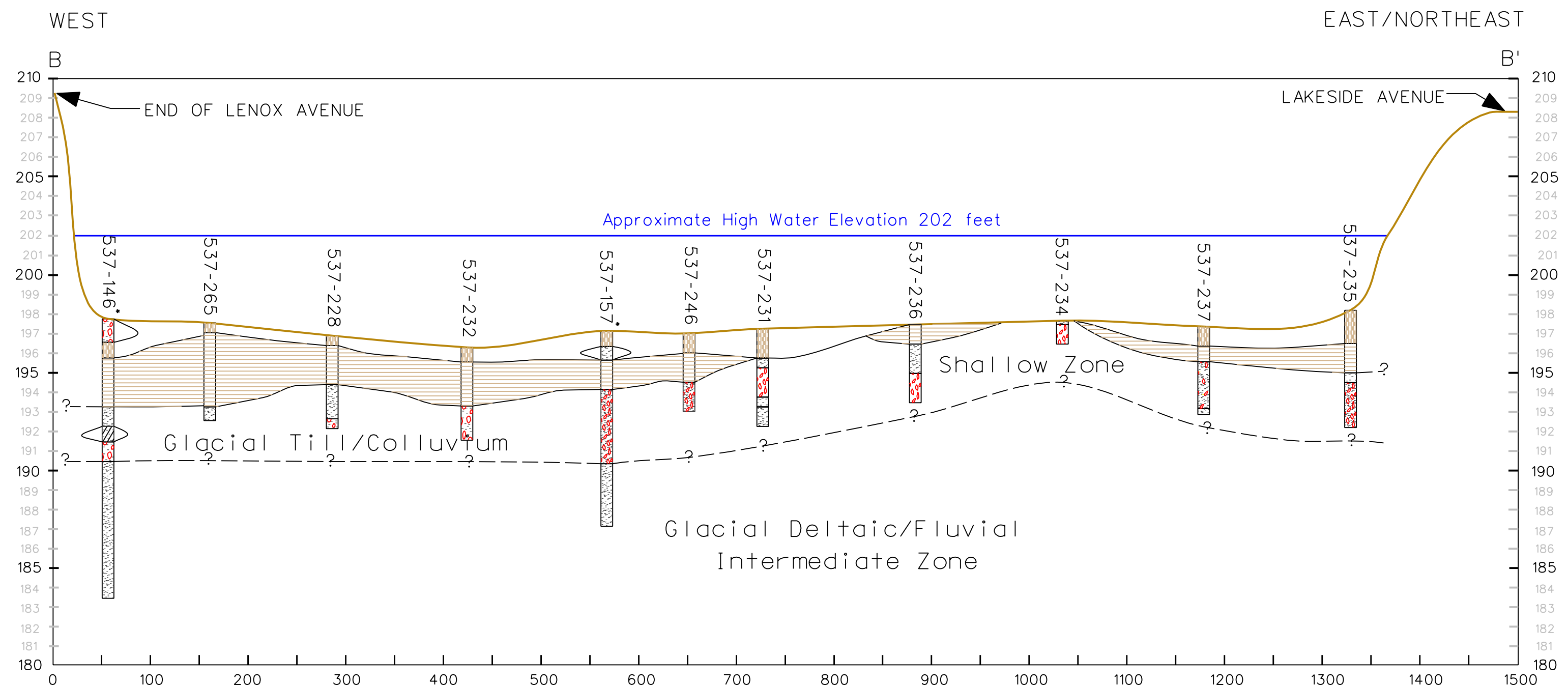
Cross-Section B-B' Acid Brook Delta DuPont Pompton Lakes Works Figure 4
