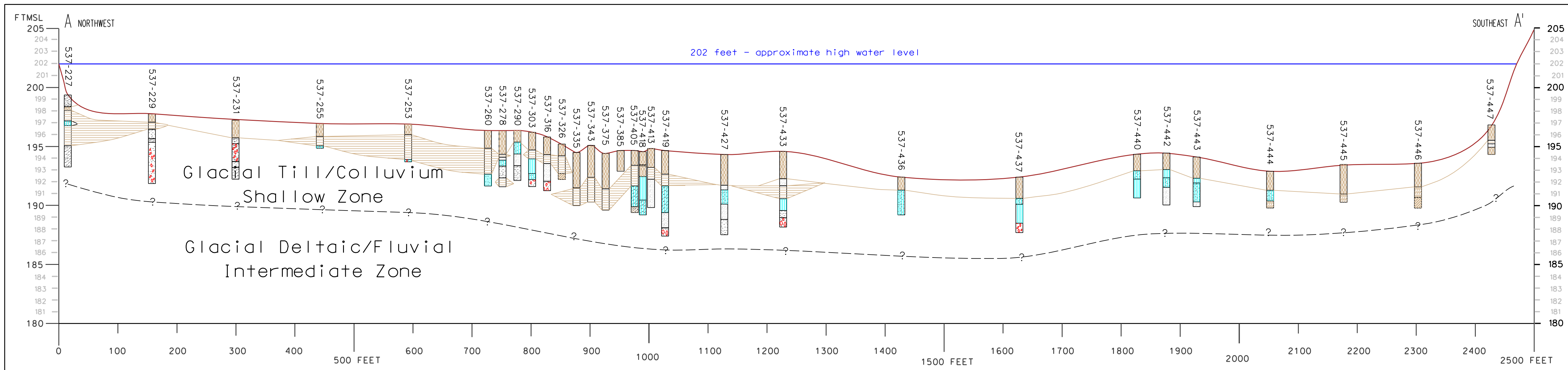
Cross-Section A-A' Acid Brook Delta DuPont Pompton Lakes Works Figure 3
