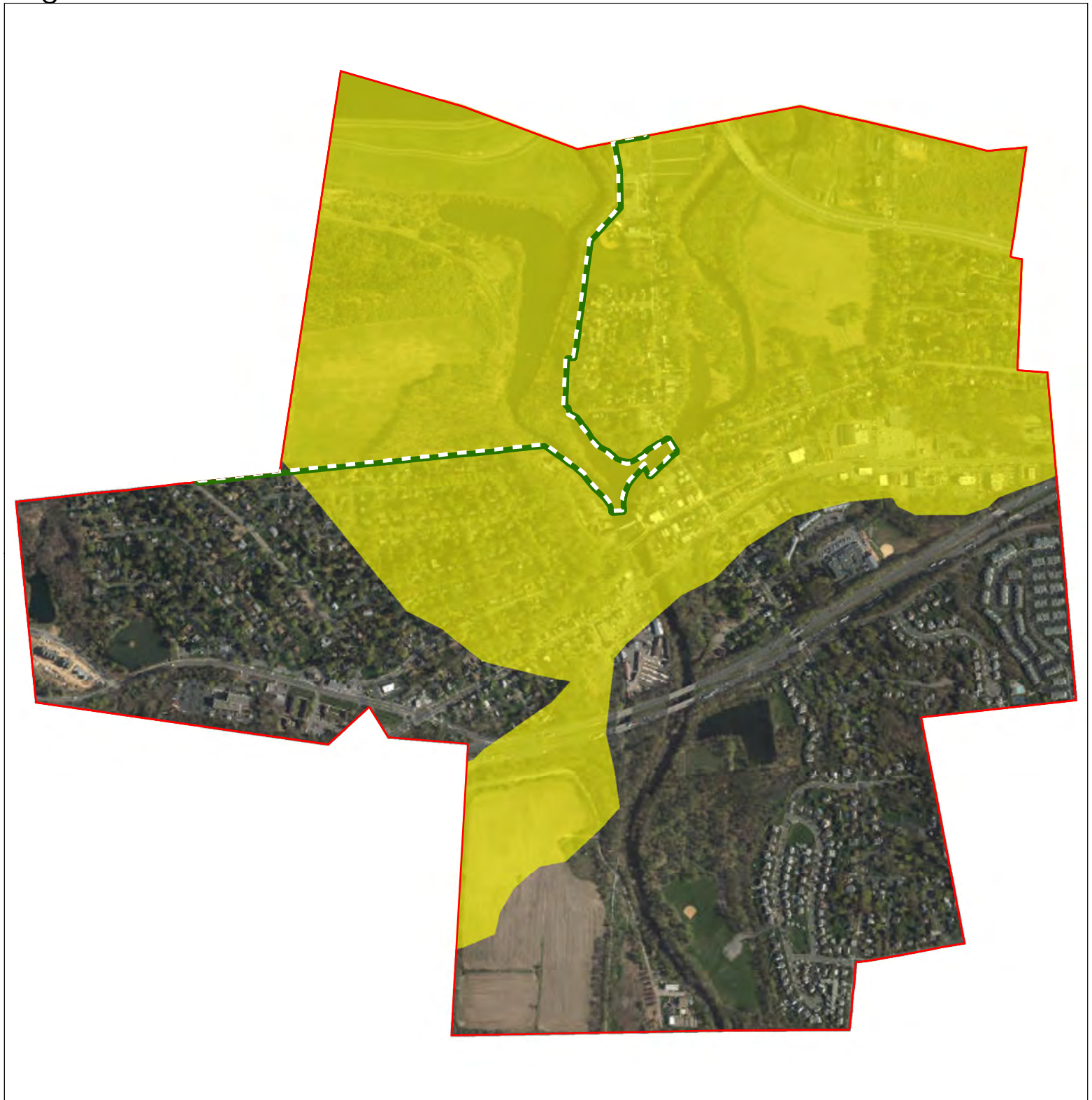
Figure 18: Carbonate Rock Areas
