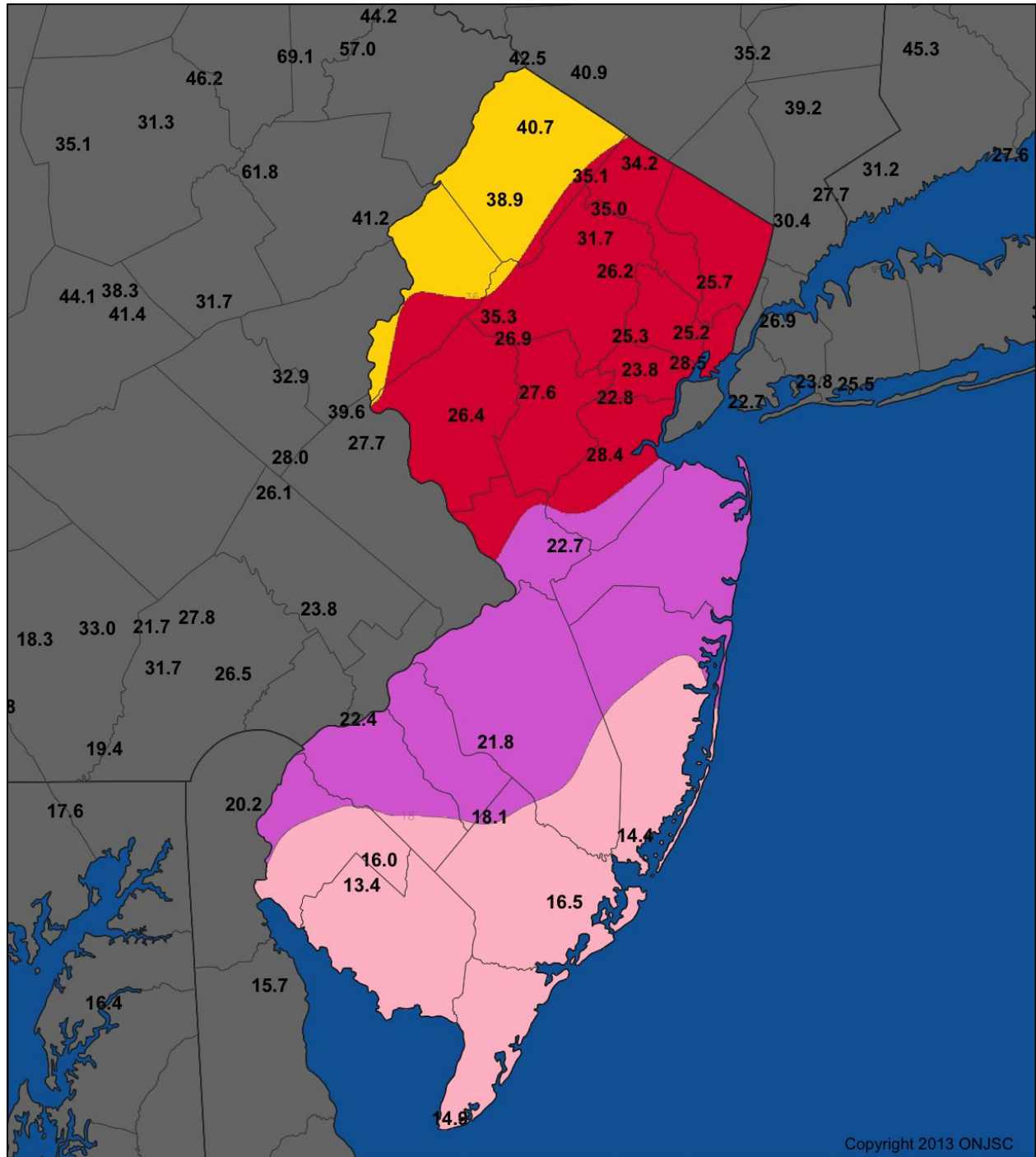
Figure 5.11-1. Normal Seasonal Snowfall, 1981-2010
