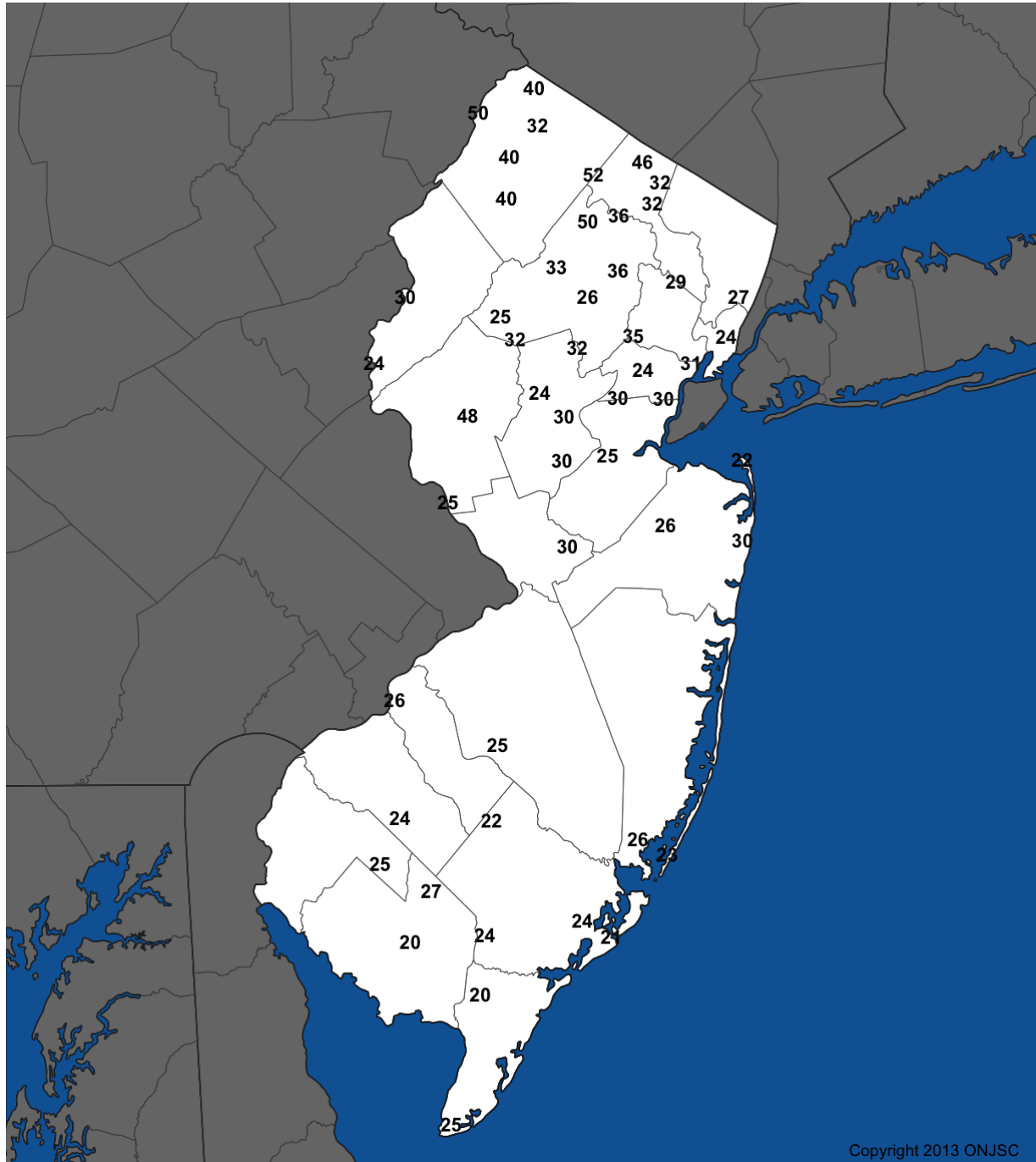
Figure 5.11-2. Extreme Depth of Snow on Ground
