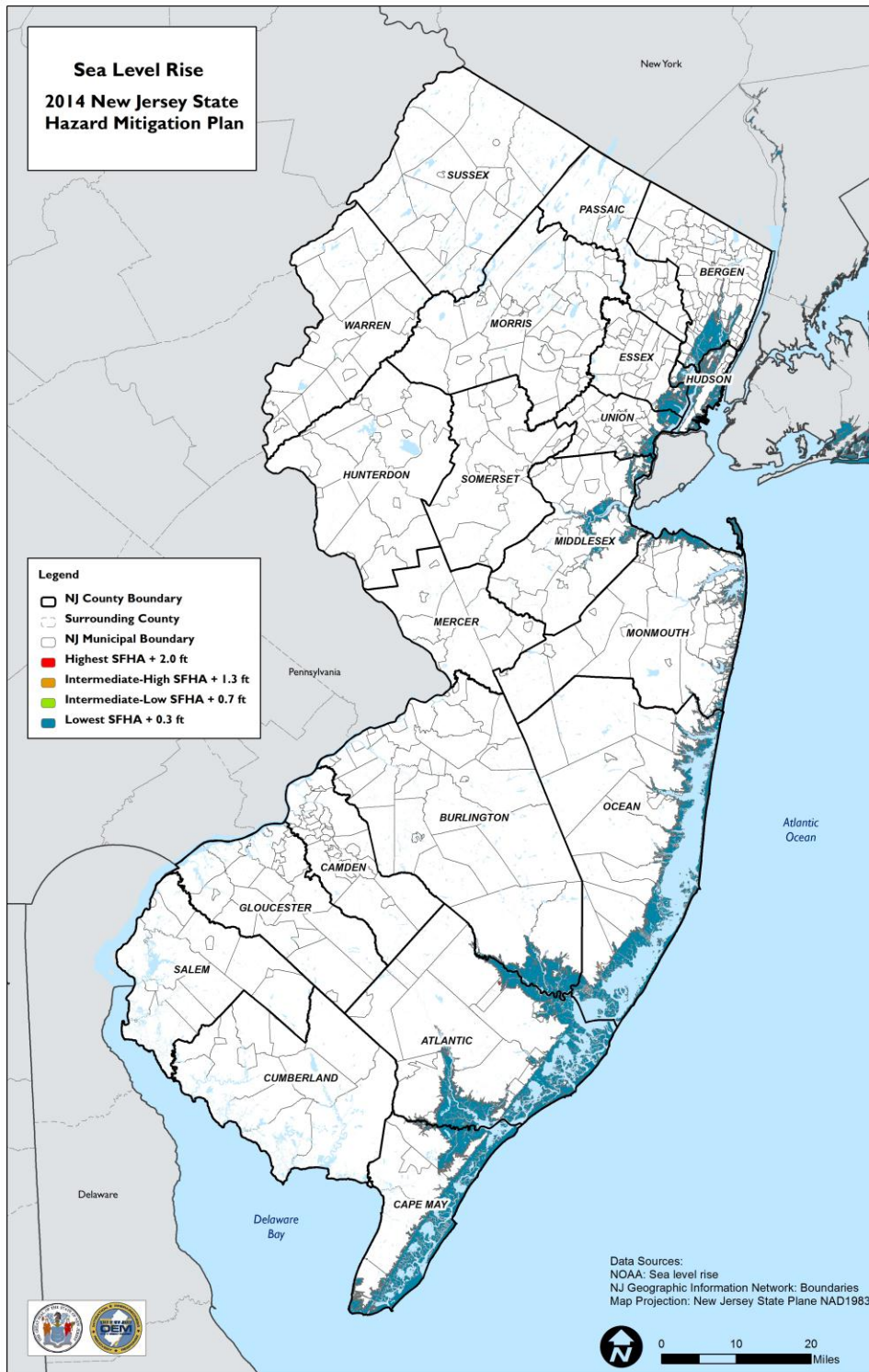
Figure 5.2-17. Global Mean Sea Level Rise Scenarios for New Jersey
