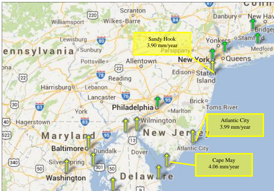
Figure 5.2-11. Sea Level Trends in New Jersey
