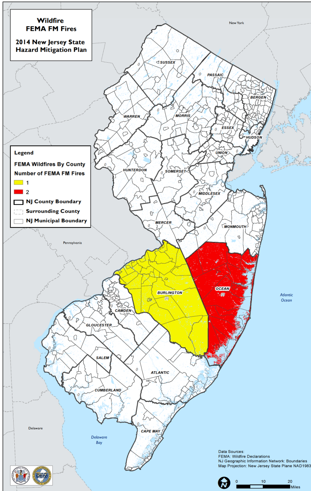
Figure 5.12-5. FEMA-Declared Wildfire Disasters by County
