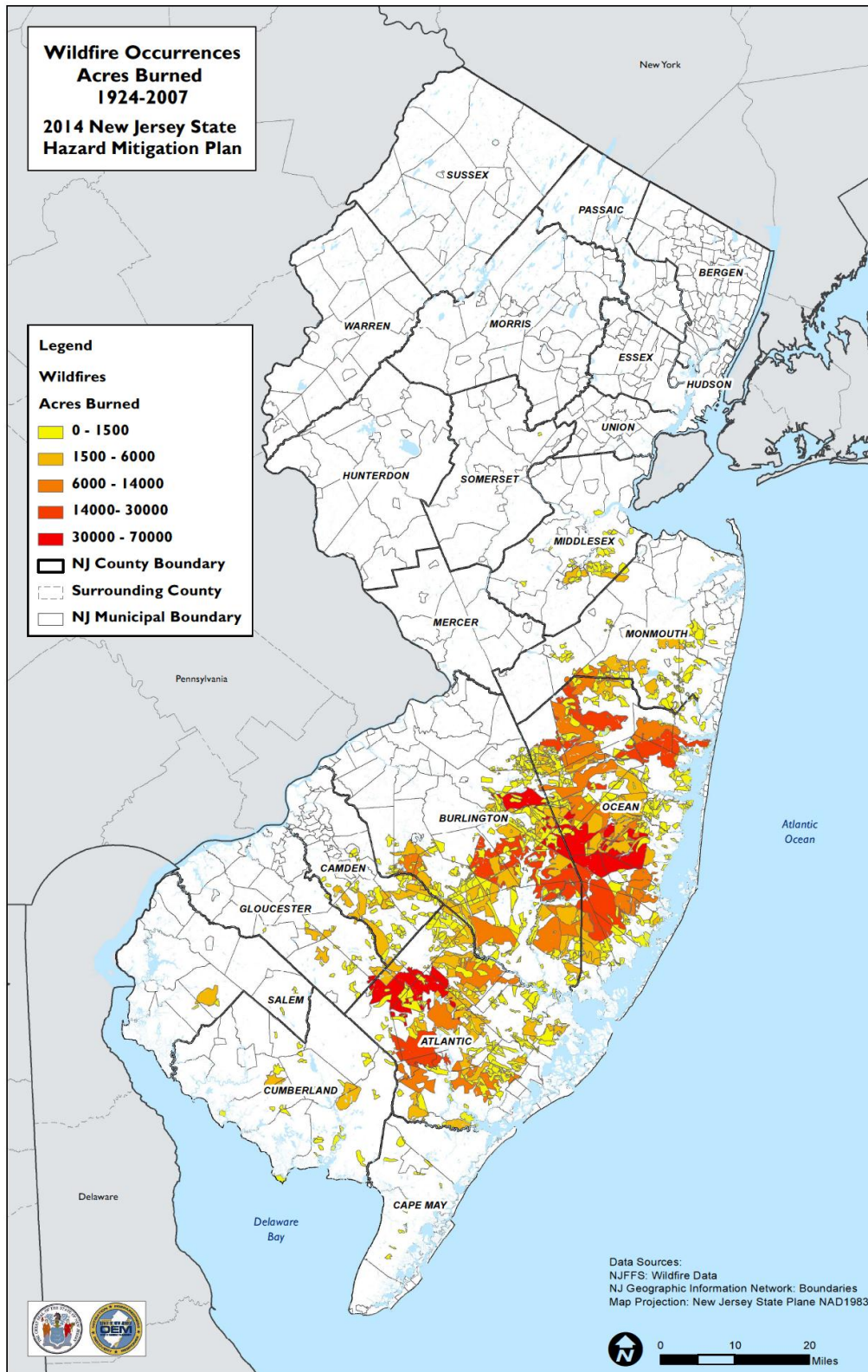
Figure 5.12-4. Past Occurrences of Wildland Fires in New Jersey
