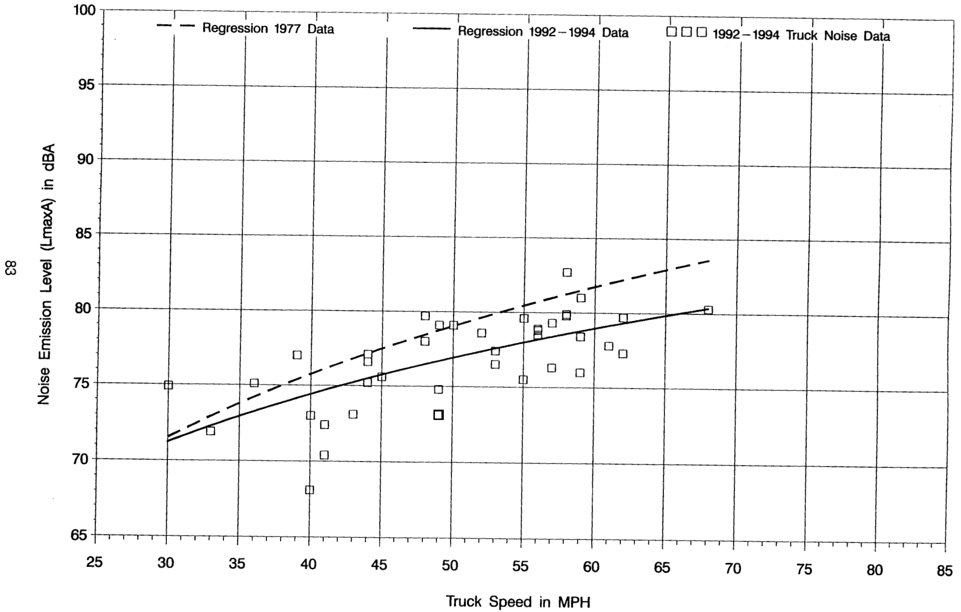
Figure B-6: Noise Emission Level (LmaxA) vs. Truck Speed ROADWAY TYPE 6 (Non-Controlled Access, Downgrade) – MEDIUM TRUCKS & BUSES
