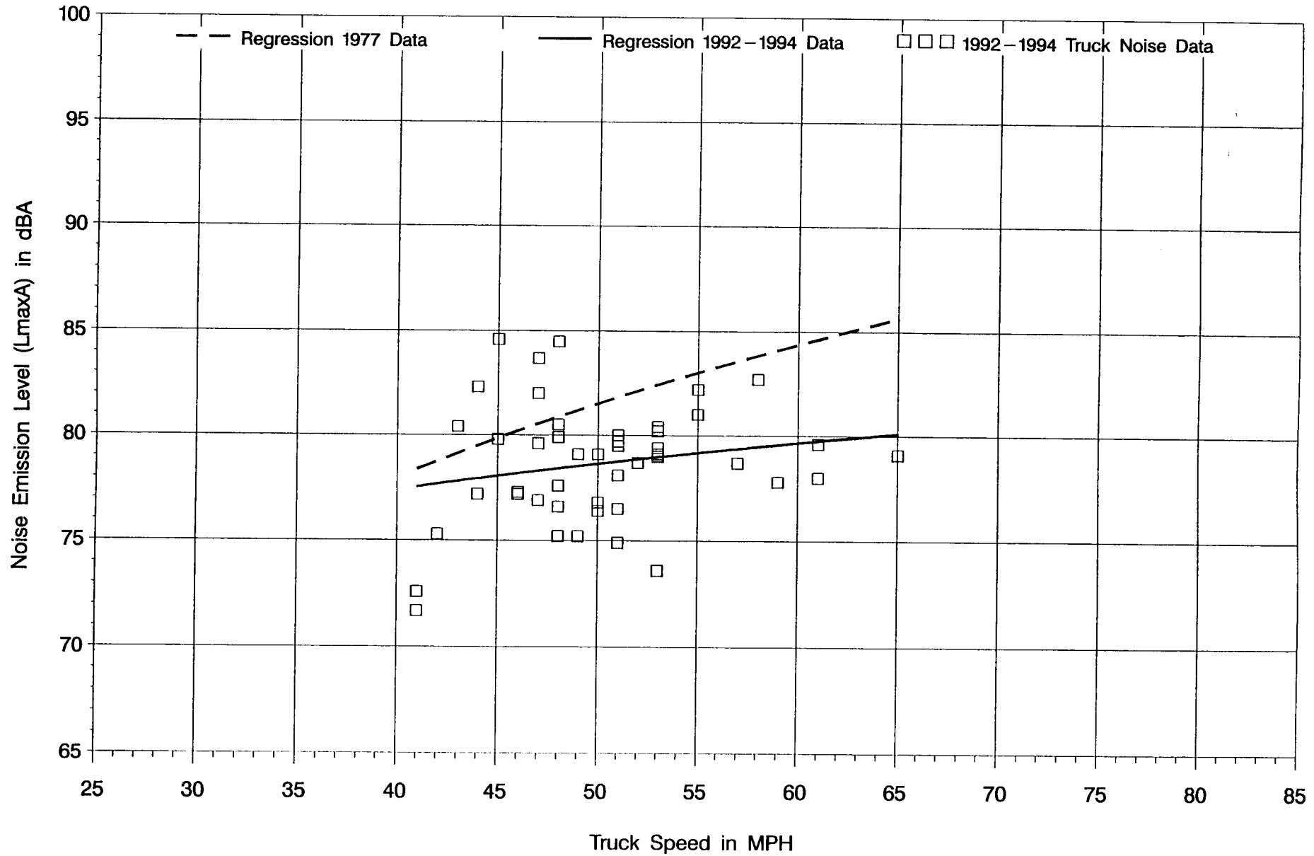
Figure B-1: Noise Emission Level (LmaxA) vs. Truck Speed ROADWAY TYPE 1 (Controlled Access, Level) – MEDIUM TRUCKS & BUSES
