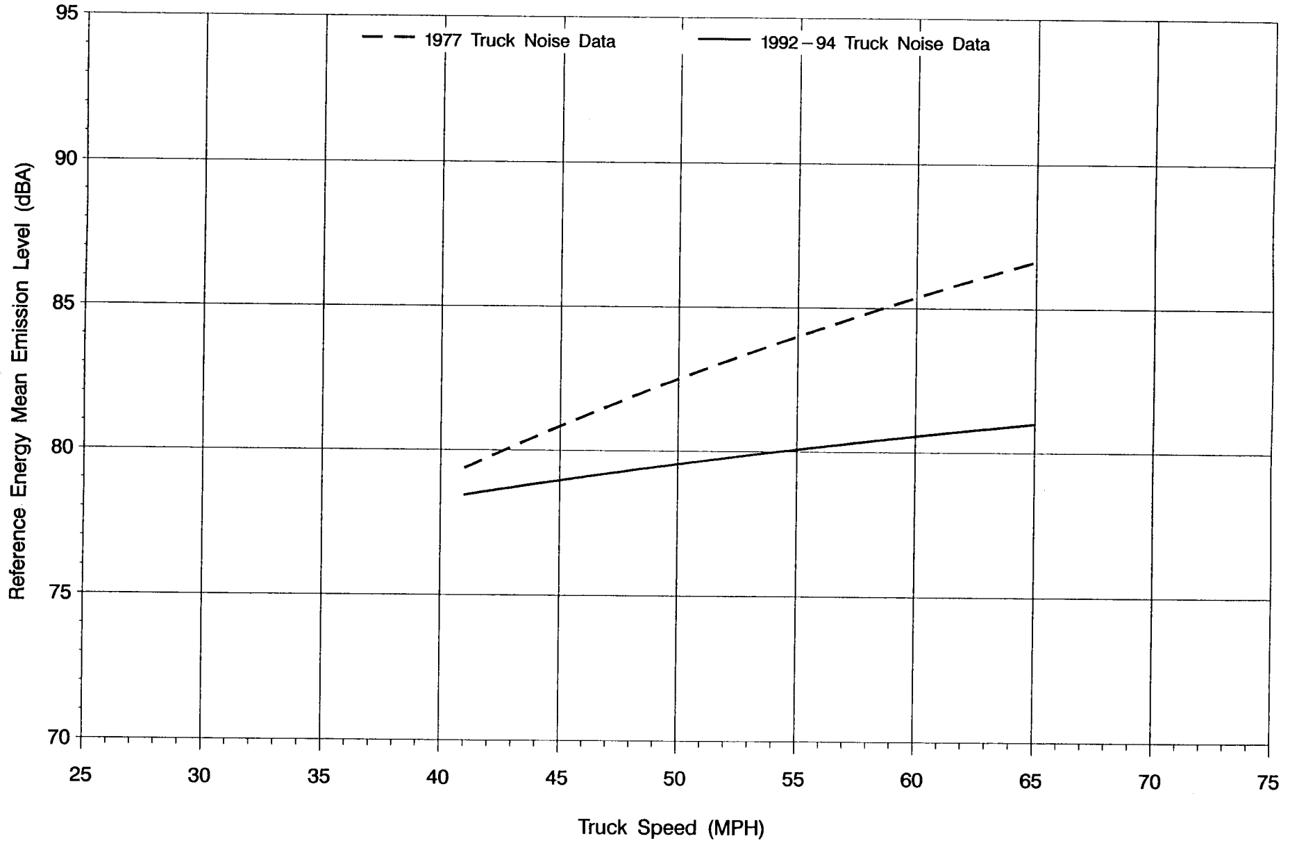
Figure 5: REMEL vs. Truck Speed ROADWAY TYPE 1 (Controlled Access, Level) – MEDIUM TRUCKS & BUSES
