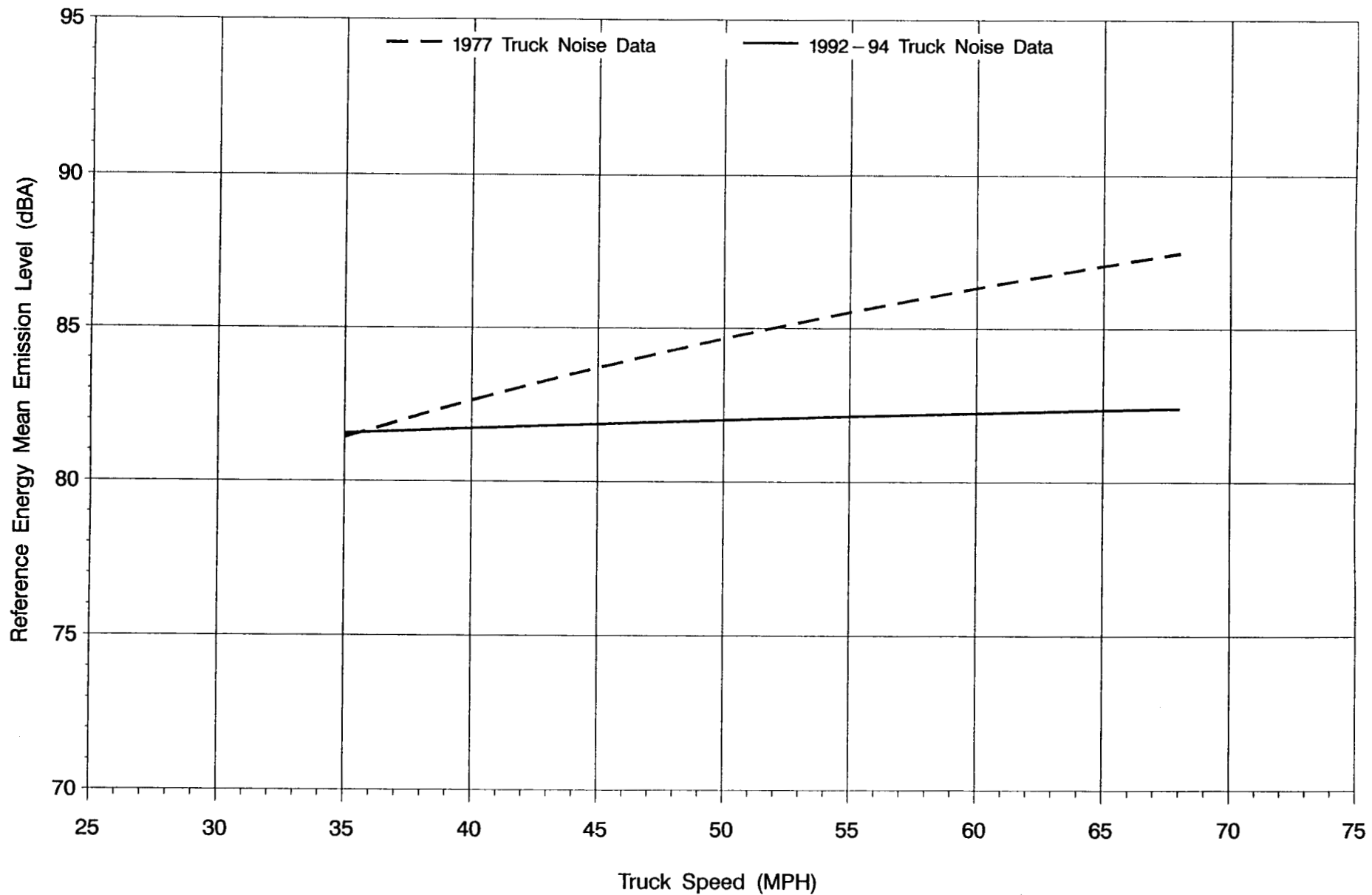
Figure 14: REMEL vs. Truck Speed ROADWAY TYPE 4 (Non-Controlled Access, Level) – HEAVY TRUCKS
