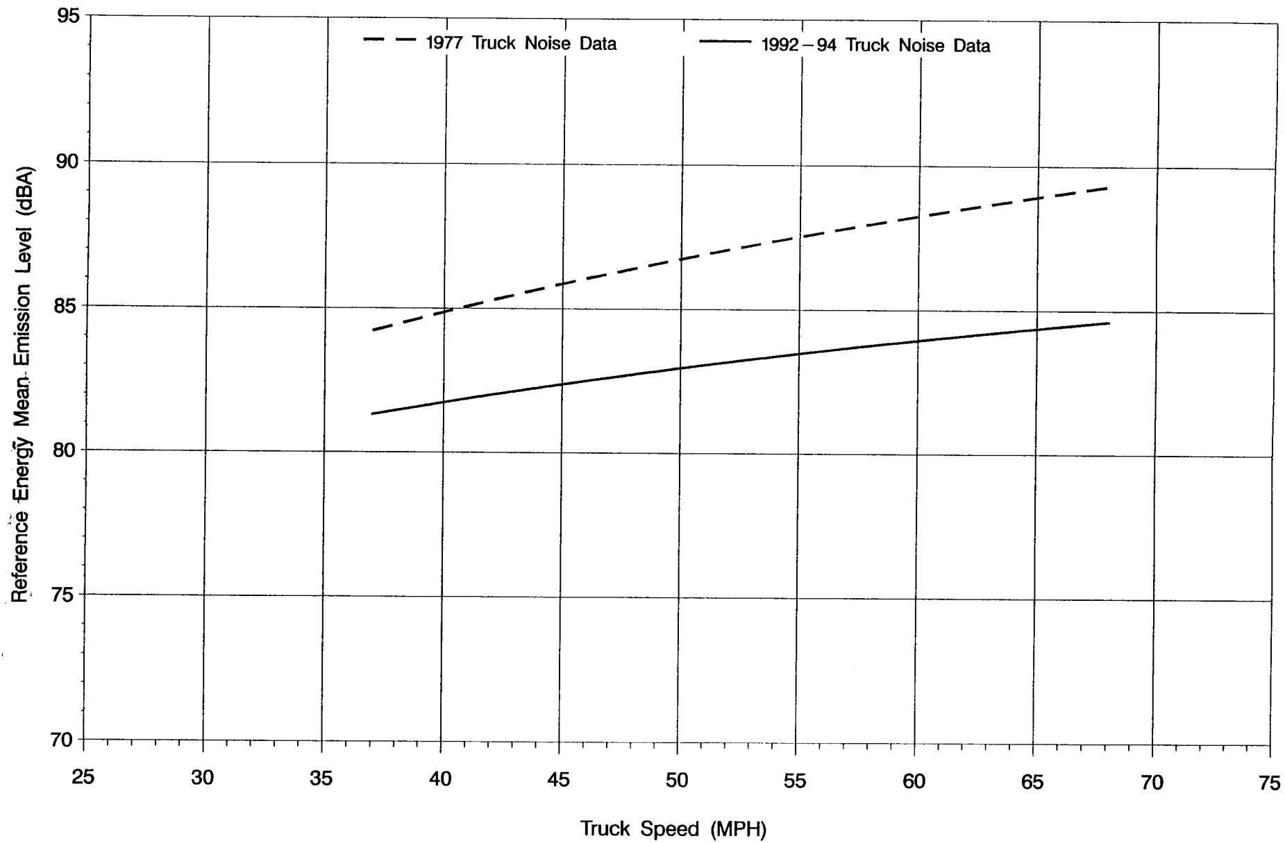
Figure 11: REMEL vs. Truck Speed ROADWAY TYPE 1 (Controlled Access, Level) – HEAVY TRUCKS
