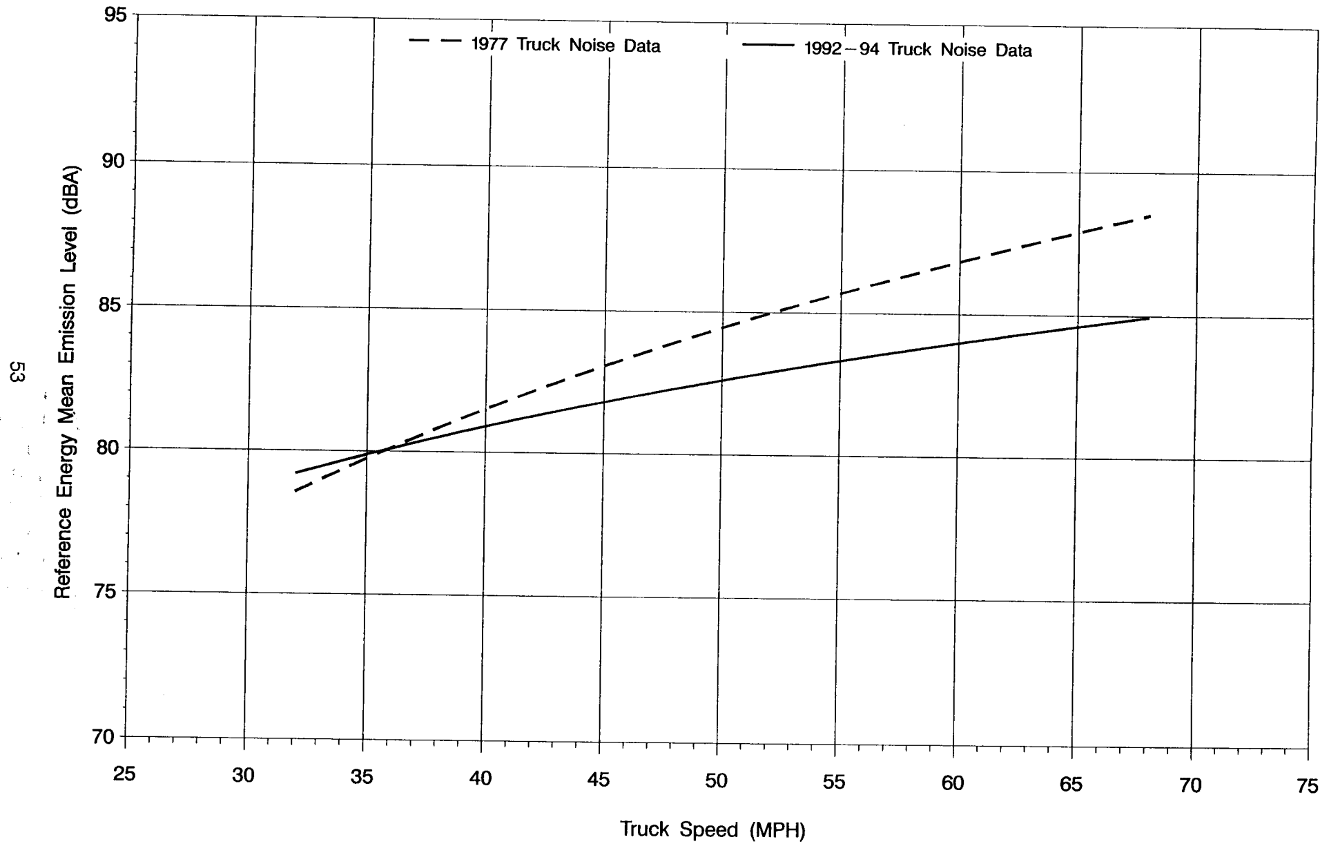
Figure 16: REMEL vs. Truck Speed ROADWAY TYPE 6 (Non-Controlled Access, Downgrade) – HEAVY TRUCKS
