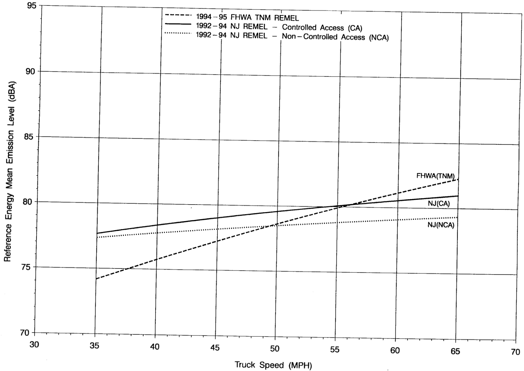
Figure 17: NJ REMELS VS. FHWA TNM REMELS – MEDIUM TRUCKS, LEVEL
