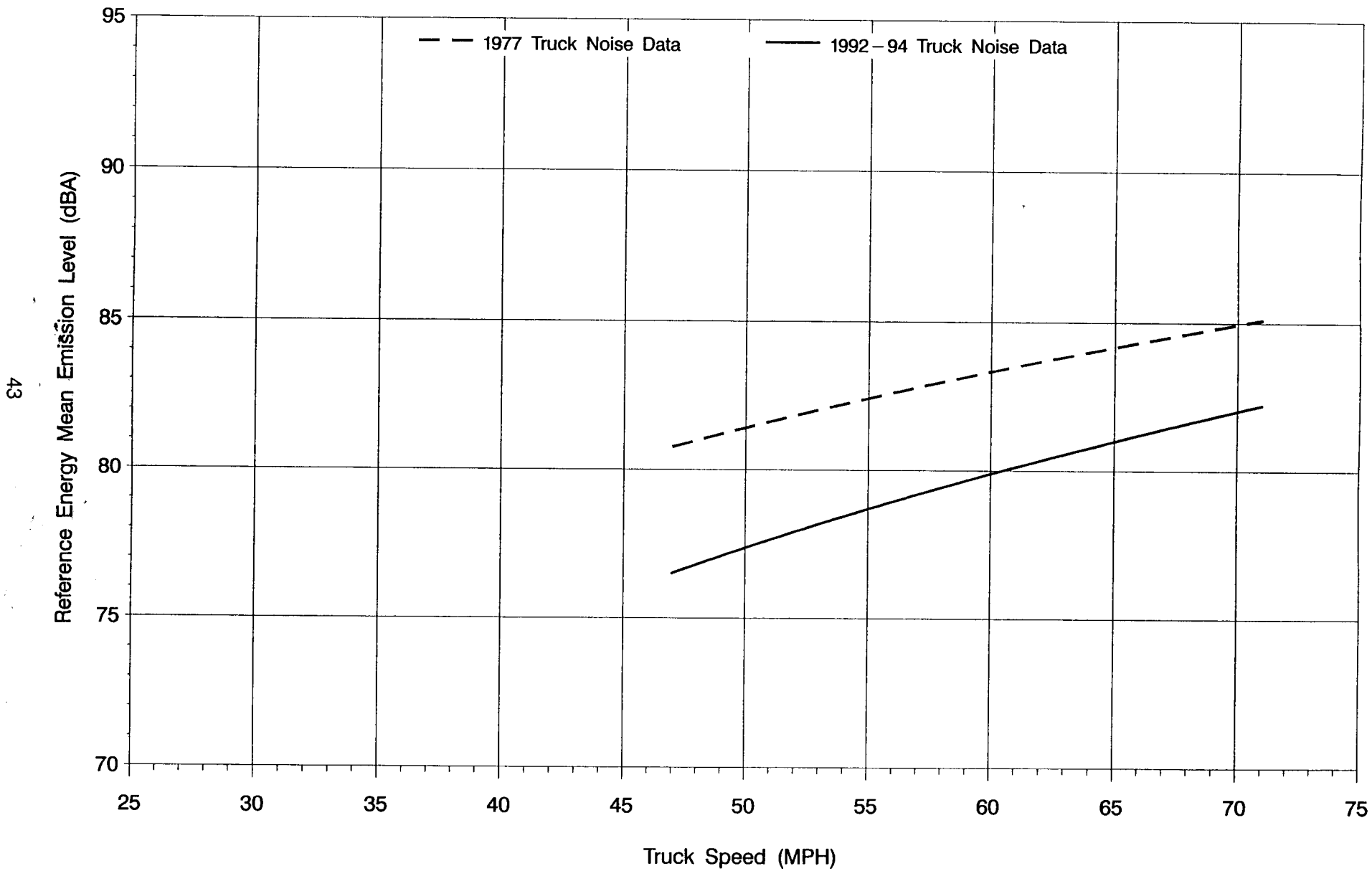
Figure 7: REMEL vs. Truck Speed ROADWAY TYPE 3 (Controlled Access, Downgrade) – MEDIUM TRUCKS & BUSES
