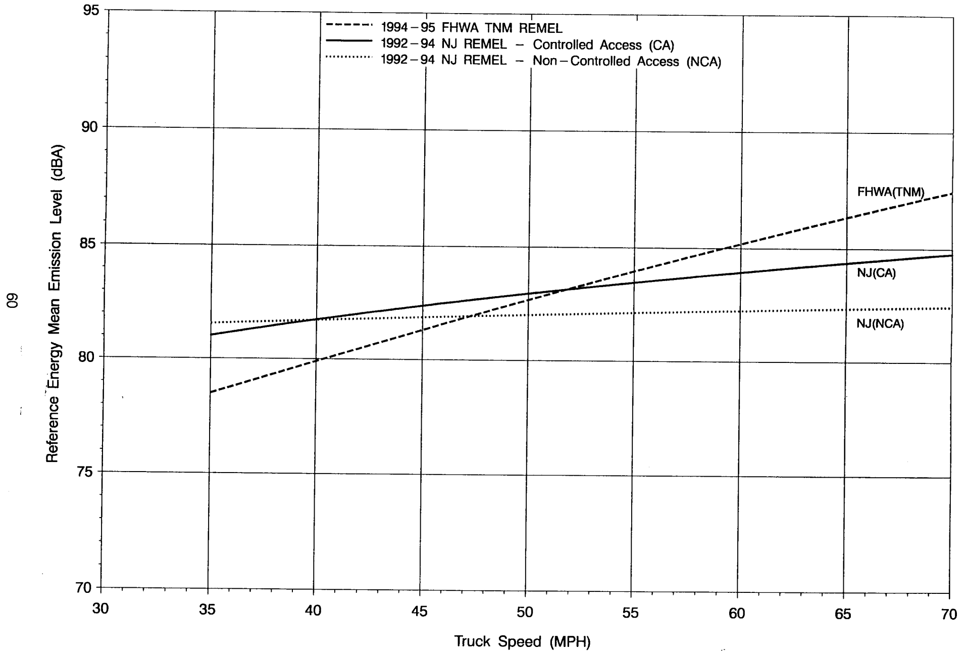
Figure 18: NJ REMELS VS. FHWA TNM REMELS – HEAVY TRUCKS, LEVEL
