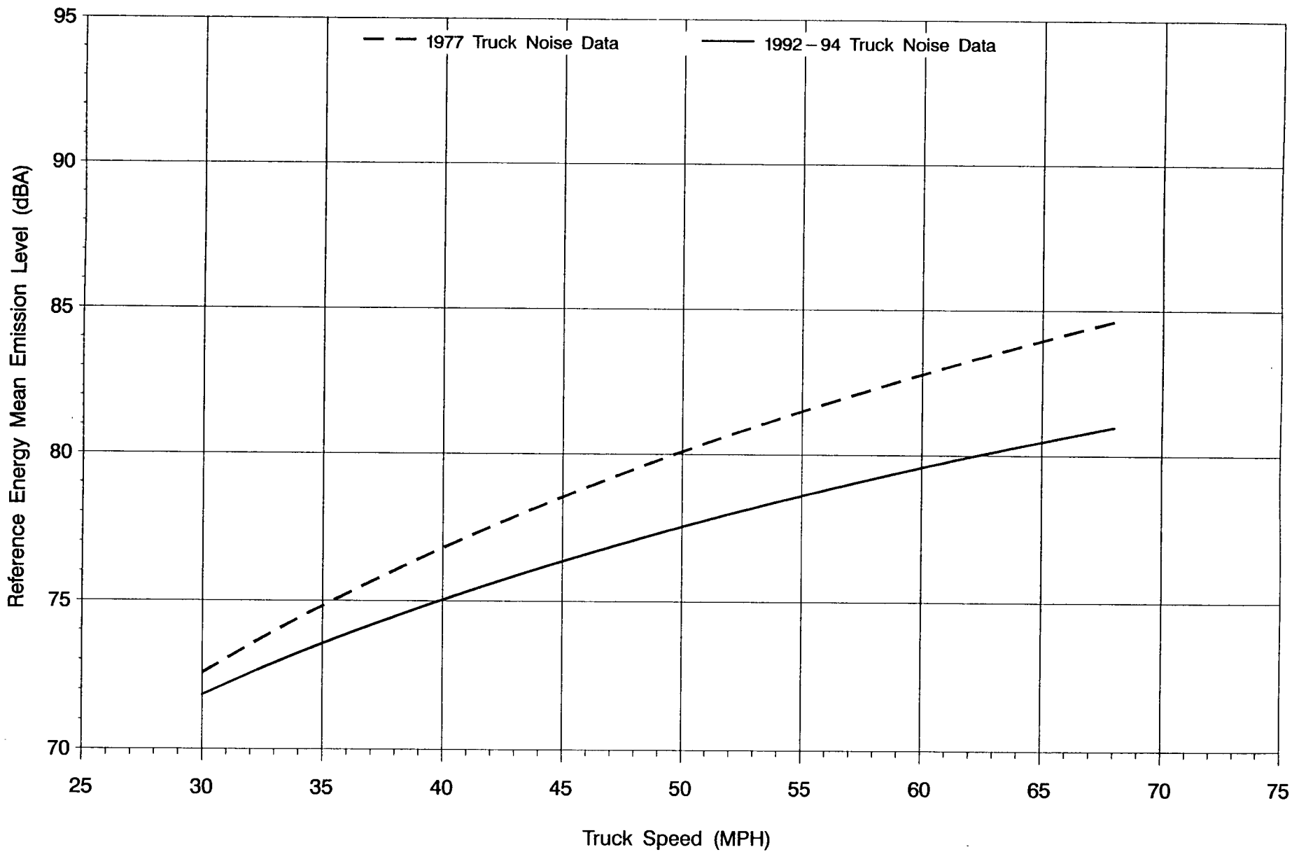
Figure 10: REMEL vs. Truck Speed ROADWAY TYPE 6 (Non-Controlled Access, Downgrade) – MEDIUM TRUCKS & BUSES
