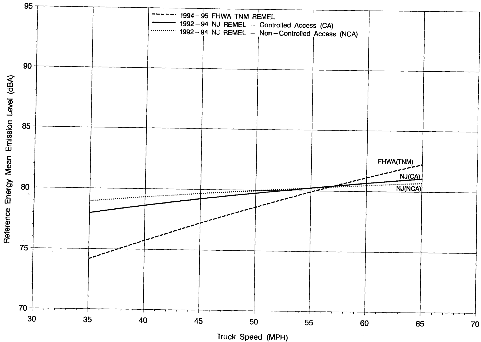
Figure 19: NJ REMELS VS. FHWA TNM REMELS – MEDIUM TRUCKS, UPGRADES
