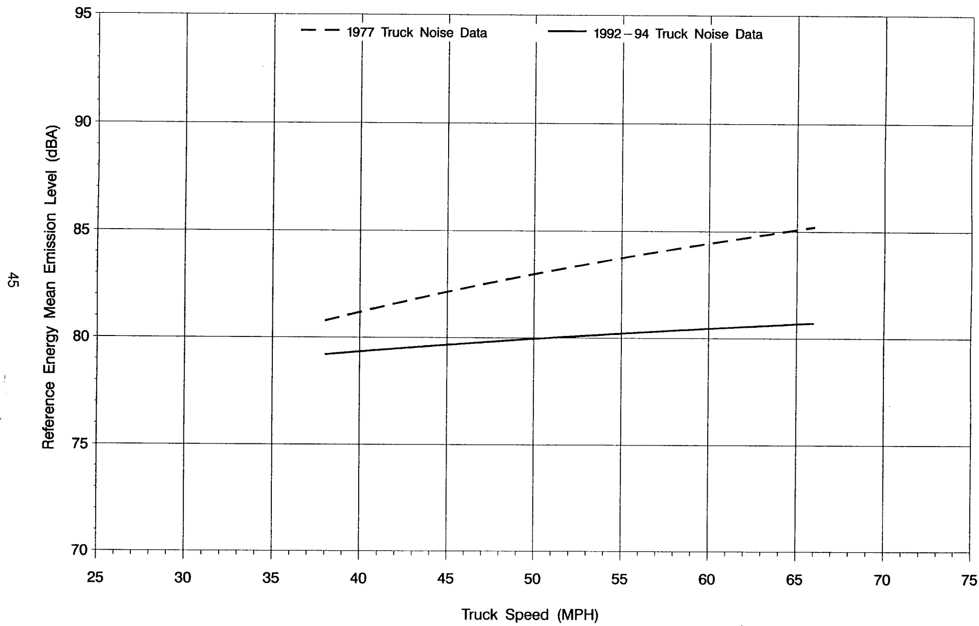
Figure 9: REMEL vs. Truck Speed ROADWAY TYPE 5 (Non-Controlled Access, Upgrade) – MEDIUM TRUCKS & BUSES
