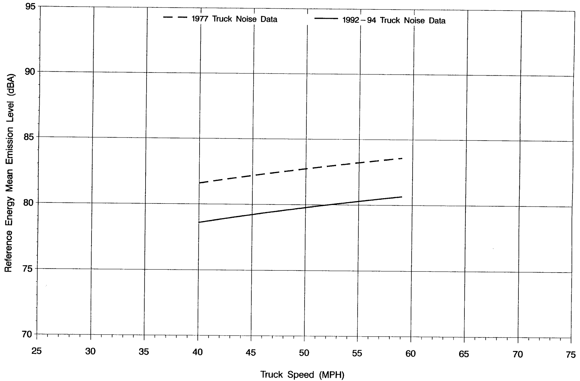
Figure 6: REMEL vs. Truck Speed ROADWAY TYPE 2 (Controlled Access, Upgrade) – MEDIUM TRUCKS & BUSES
