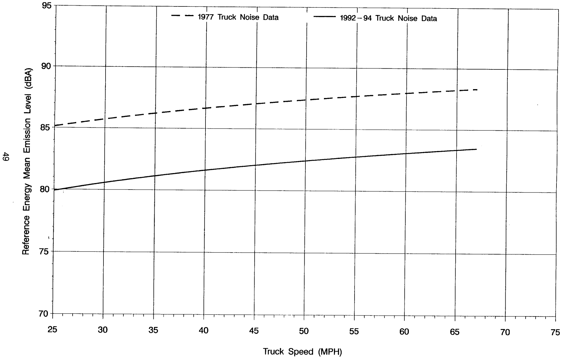
Figure 12: REMEL vs. Truck Speed ROADWAY TYPE 2 (Controlled Access, Upgrade) – HEAVY TRUCKS
