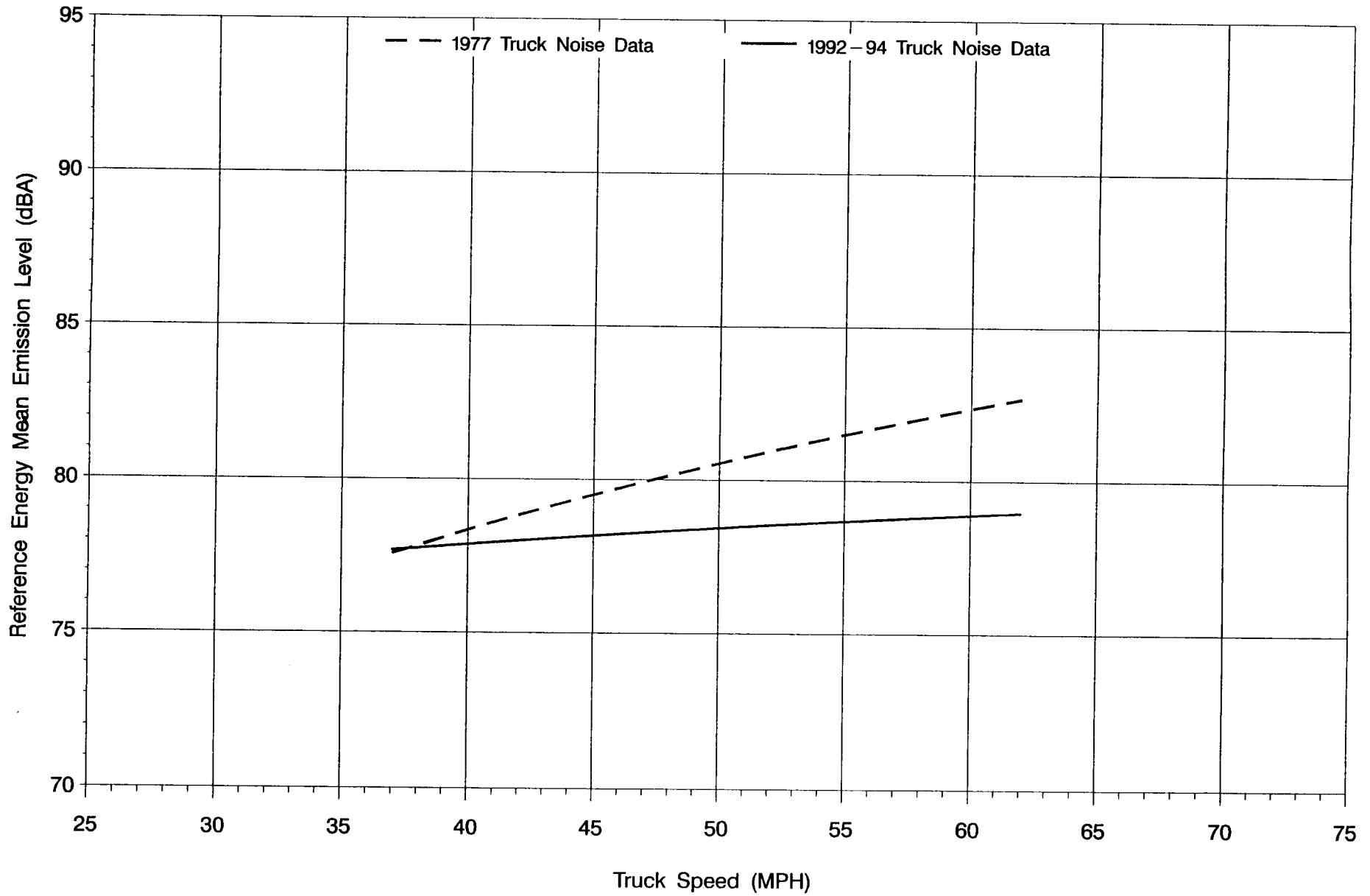
Figure 8: REMEL vs. Truck Speed ROADWAY TYPE 4 (Non-Controlled Access, Level) – MEDIUM TRUCKS & BUSES
