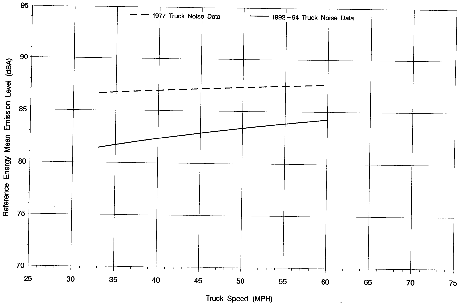
Figure 15: REMEL vs. Truck Speed ROADWAY TYPE 5 (Non-Controlled Access, Upgrade) – HEAVY TRUCKS
