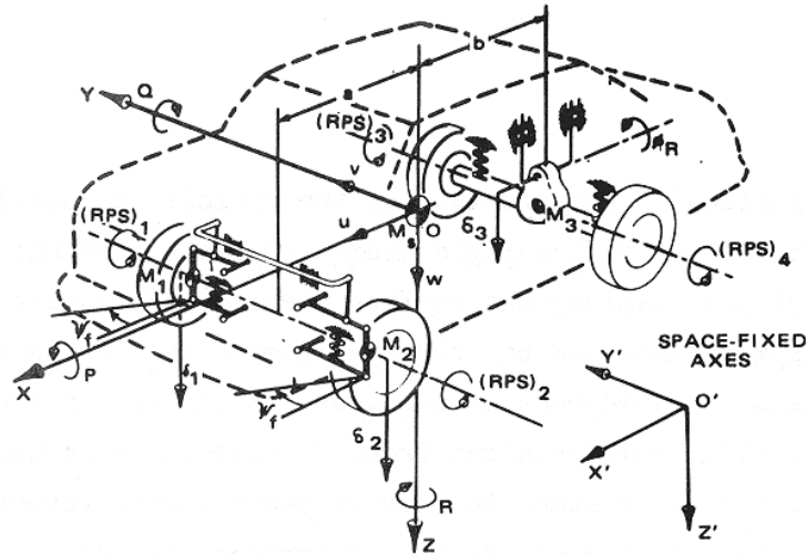
Figure 2. HVOSM Model of a Vehicle Having Independent Front Suspension and a Solid Rear Axle
