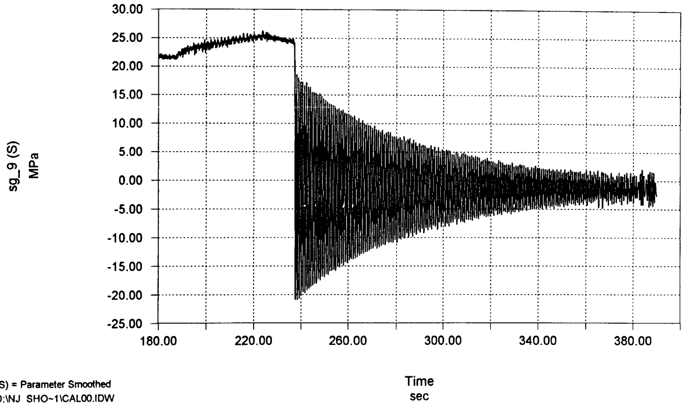
Figure 3-20 Damping of Motion in a Column Strain Gage.
