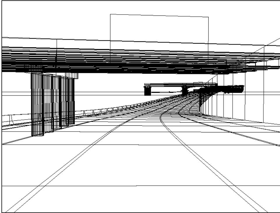
Figure 3. Wire-Frame View of Roadway, Bridge, Sign, and Retaining Wall Mesh Created by Meshing Program
