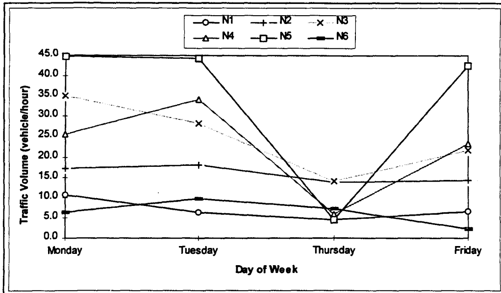
Figure 6. 12 Hourly Traffic Volume vs. Weekdays at Access Points of Gas Stations
