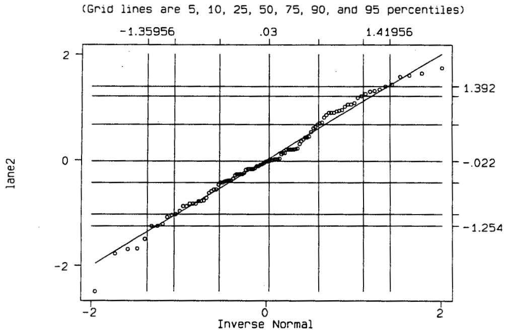
Figure 5.45(a) Normality plot of ln values of accident rate data of 2-lane highways
