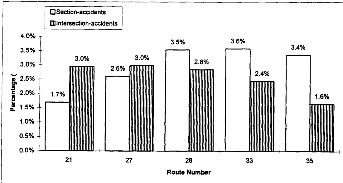
Figure 5. 20 Section-Accidents (%) and Intersection-Accidents (%) vs. Route Number (Head-on Collision)
