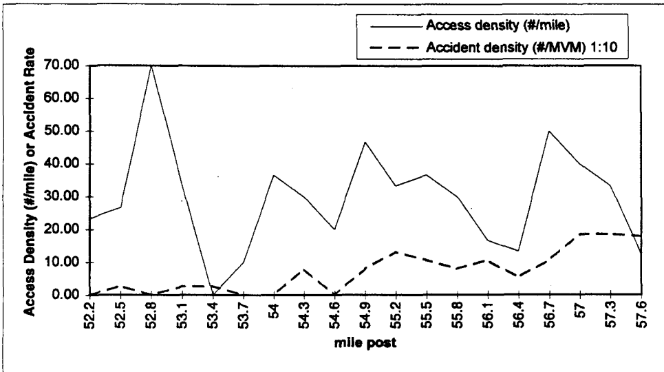
Figure 5. 7 Accident Rate and Access Density vs. Milepost (Rt. 35, Northbound, 1994)
