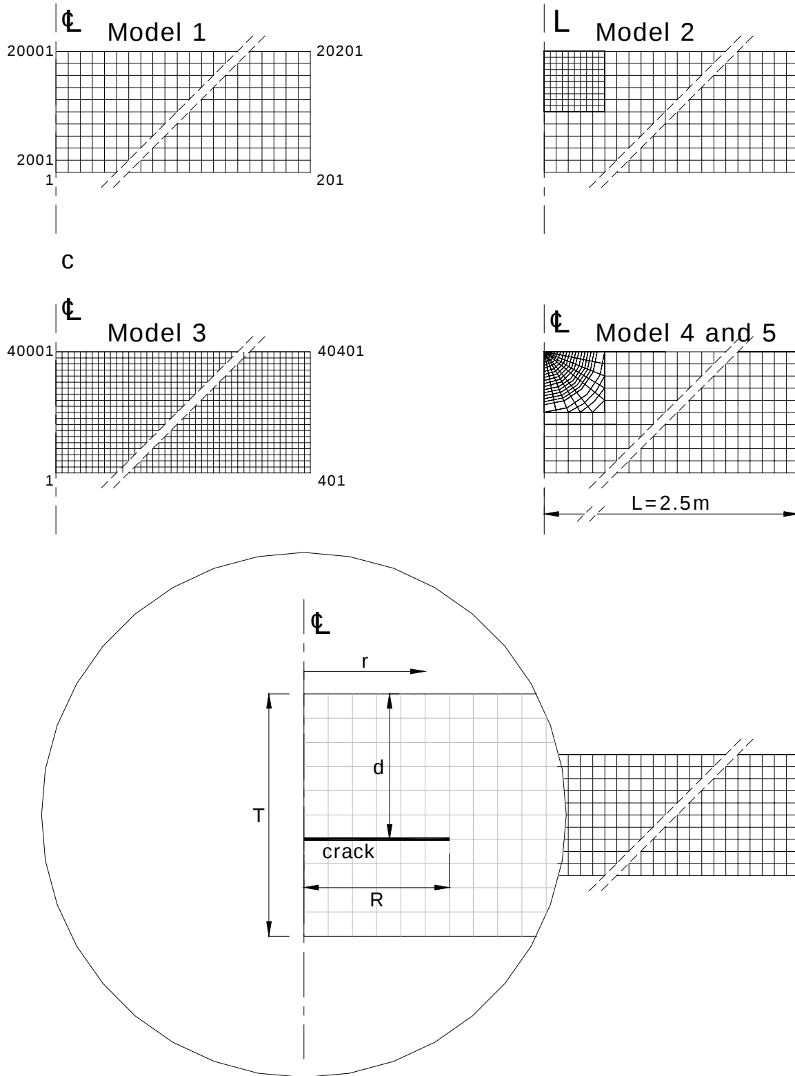
Figure 5.1. Finite element models used in simulation of PSPA testing.
