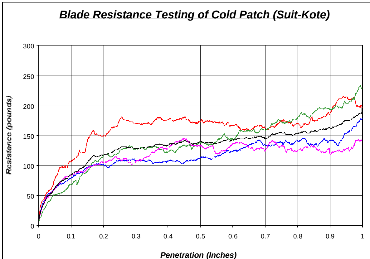
Figure 34. Blade Resistance Testing of Cold Patch (SuitKote)
