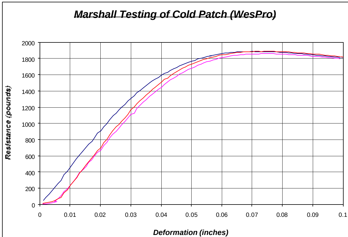
Figure 29. Marshall Testing of Cold patch (WesPro)
