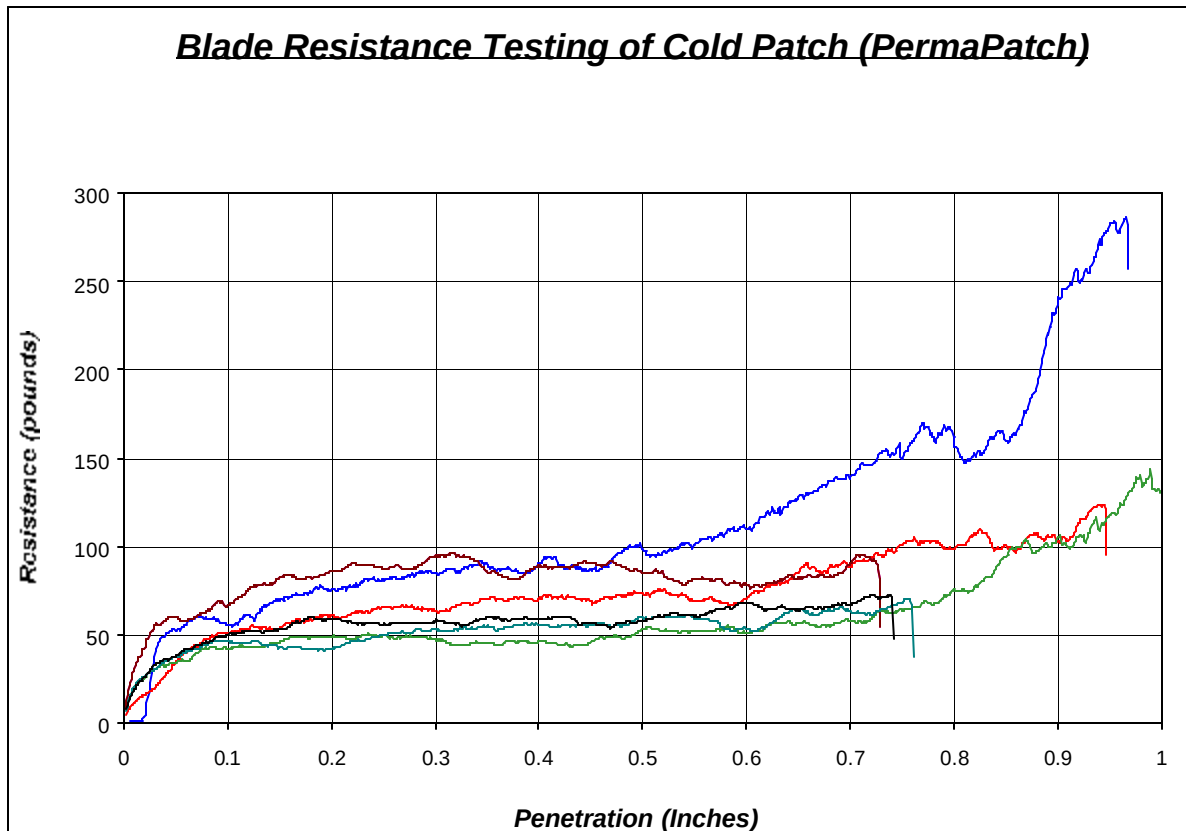
Figure 33. Blade Resistance Testing of Cold Patch (PermaPatch)
