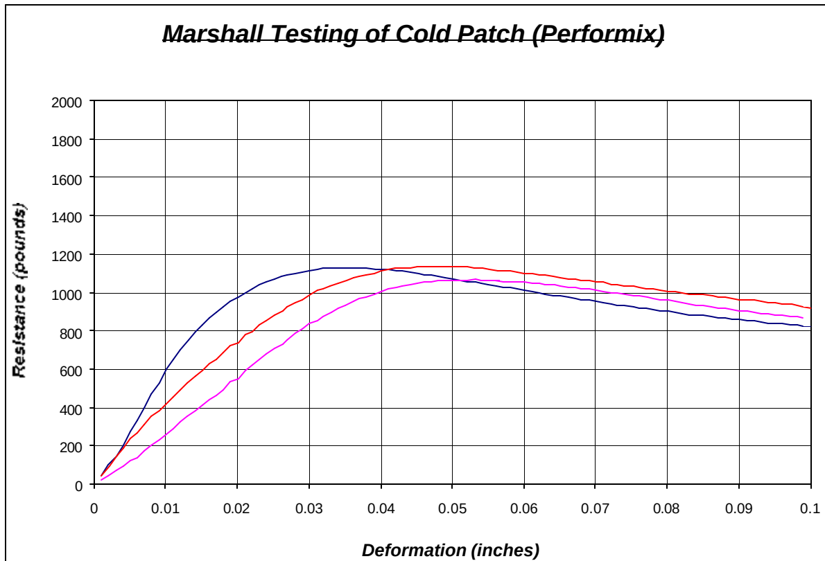
Figure 24. Marshall Testing of Cold patch (Performix)
