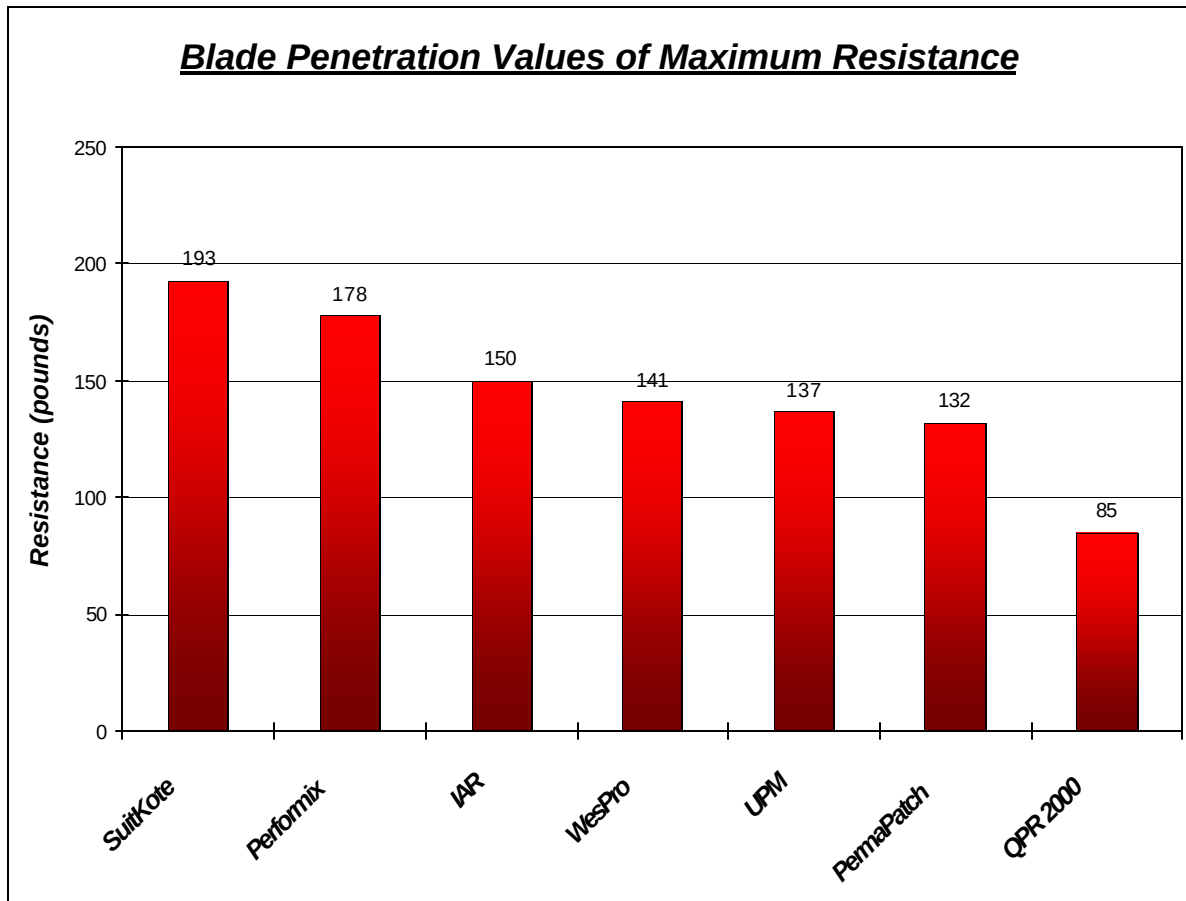
Figure 30. Blade Penetration Values of Maximum Resistance
