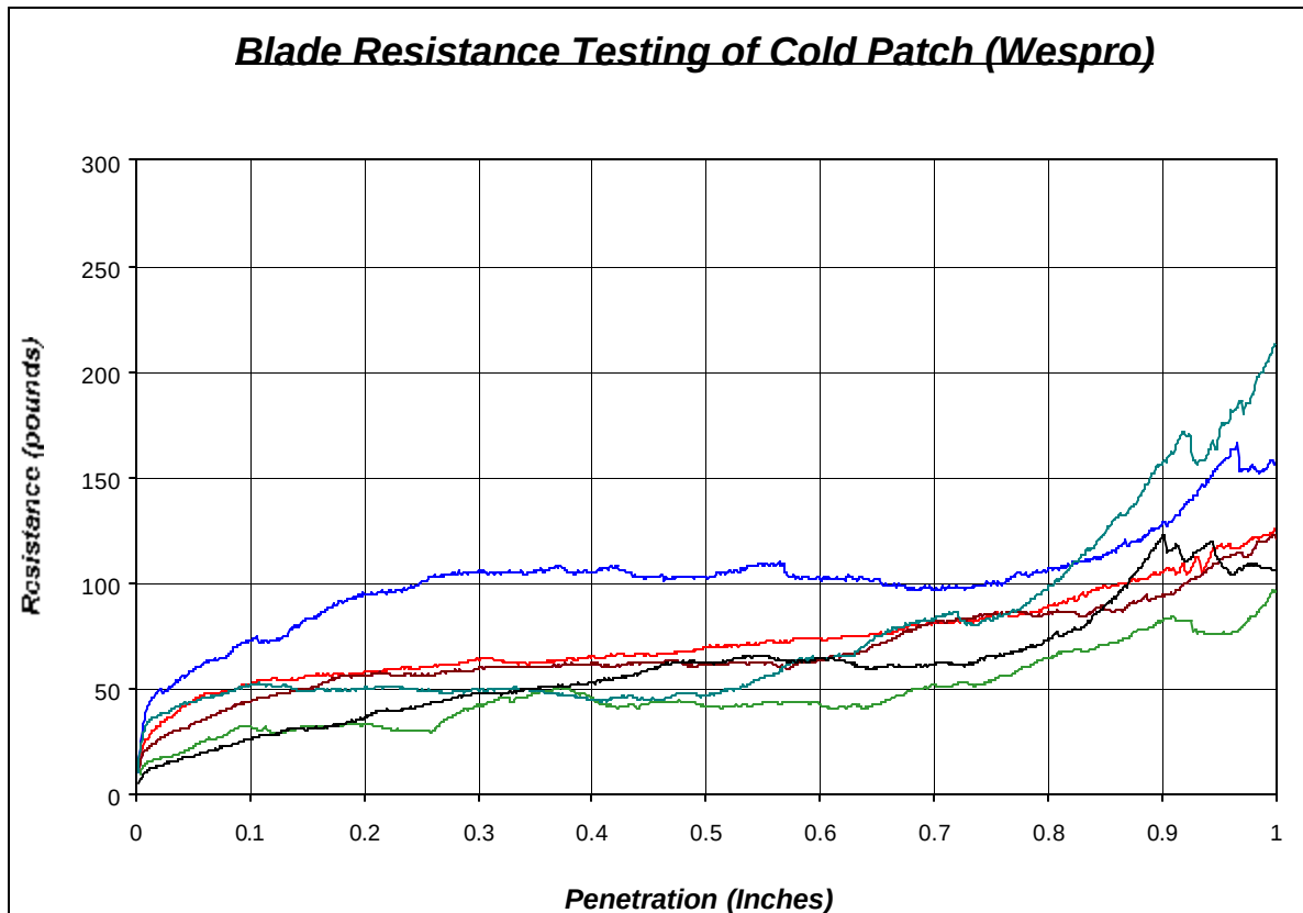
Figure 37. Blade Resistance Testing of Cold Patch (Wespro)
