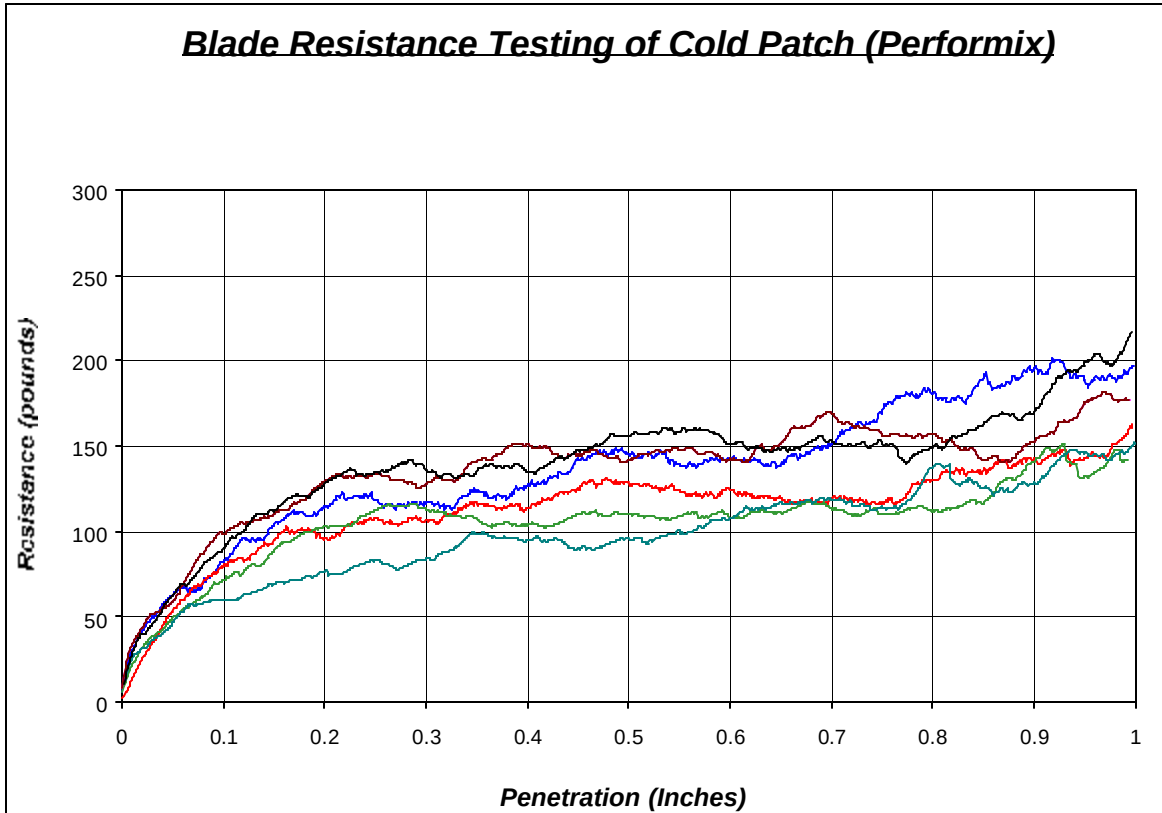
Figure 32. Blade Resistance Testing of Cold Patch (Performix)
