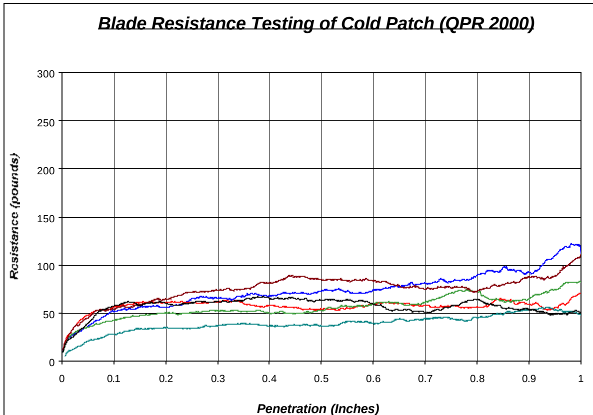
Figure 36. Blade Resistance Testing of Cold Patch (QPR 2000)
