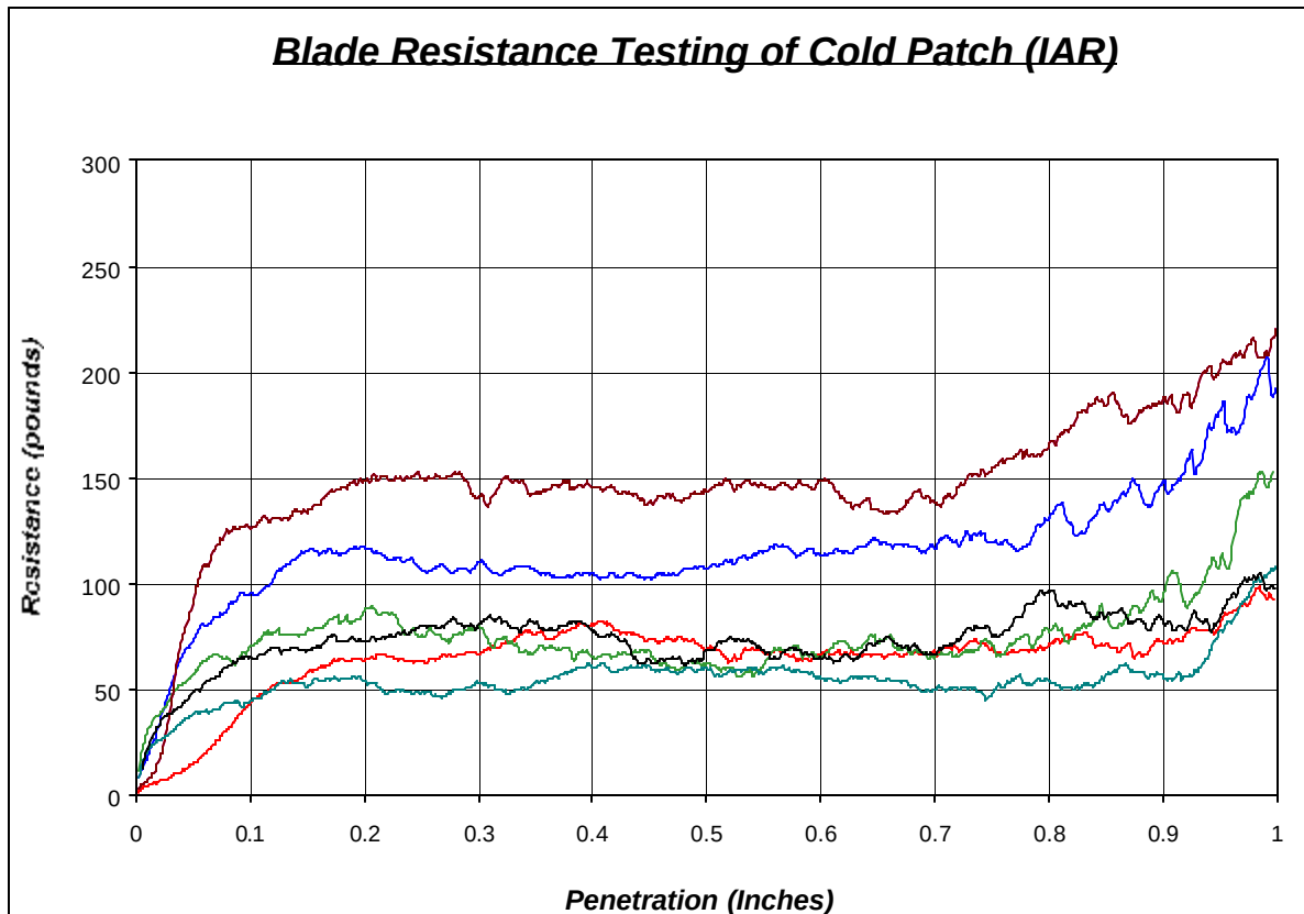
Figure 31. Blade Resistance Testing of Cold Patch (IAR)
