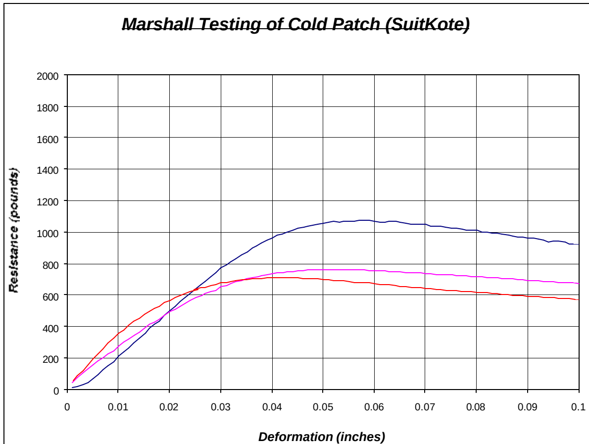
Figure 27. Marshall Testing of Cold Patch (SuitKote)
