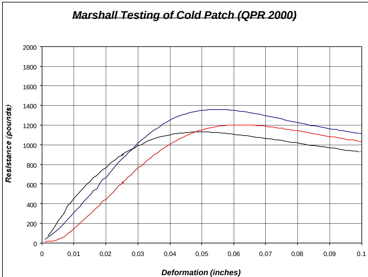
Figure 26. Marshall Testing of Cold Patch (QPR 2000)
