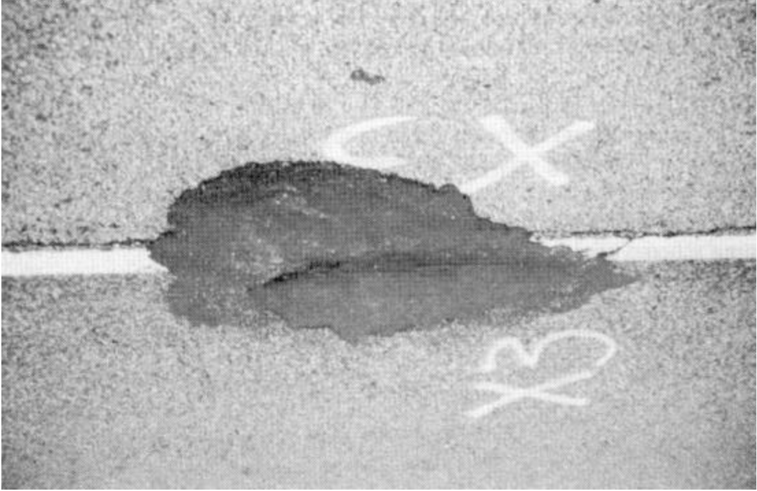
Figure 5. Shoving Distress (3)
