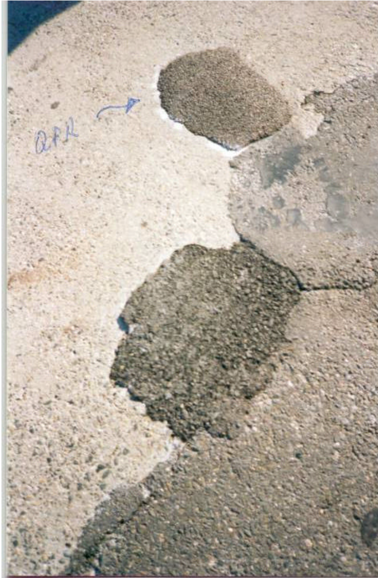
Figure 44. QPR 2 Month Inspection, Rt 21 SB MP 12.0 Passaic
