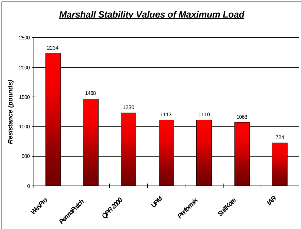
Figure 22. Marshall Stability Values of Maximum Load
