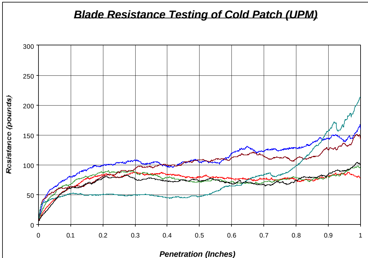
Figure 35. Blade Resistance Testing of Cold Patch (UPM)
