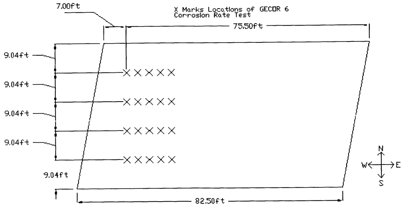
Fig. 3.14: Locations of GECOR 6 Corrosion Rate Meter Tests Wyckoff Road Eastbound
