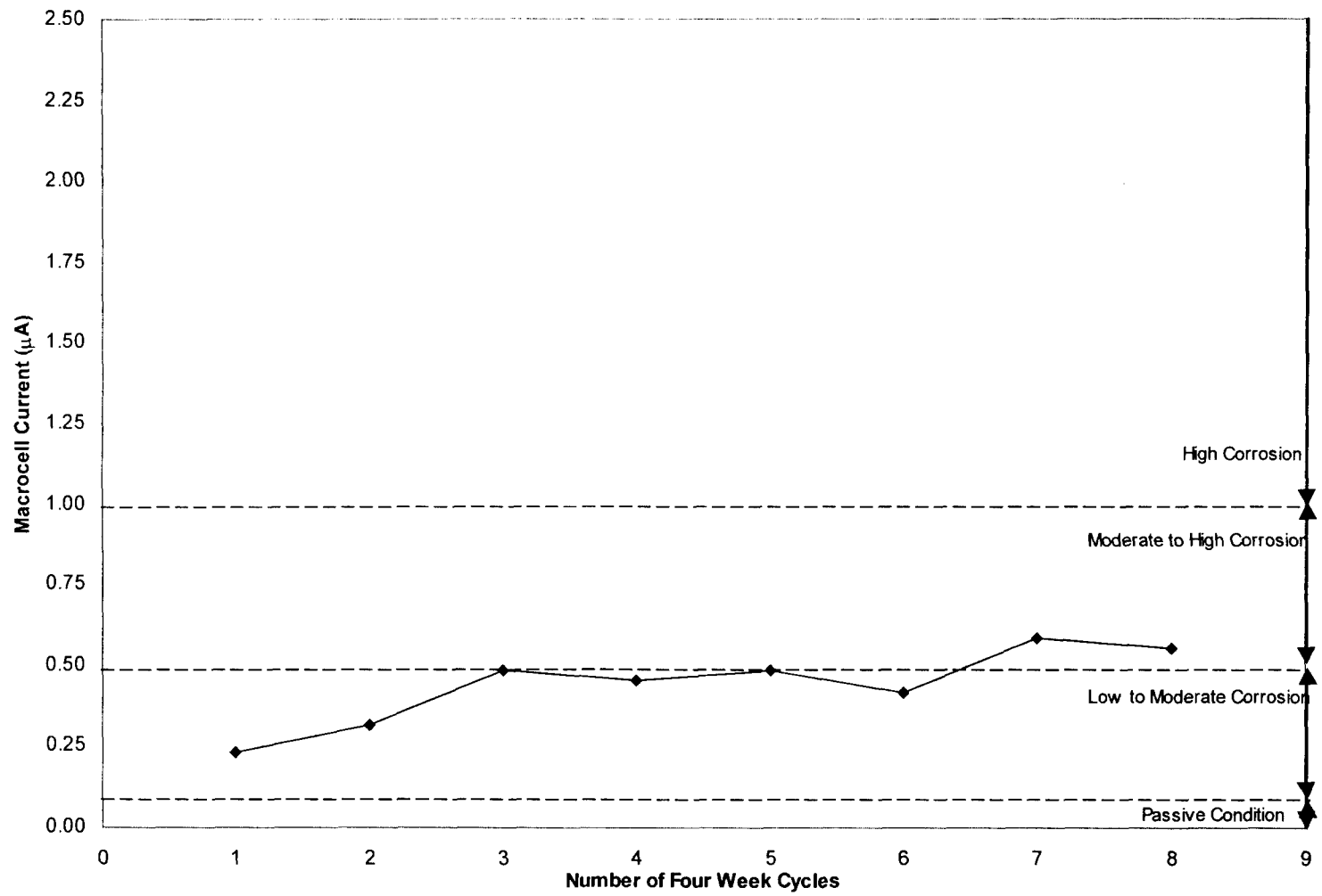
Fig. 4.15: Minideck C - Average Corrosion Rate Macrocell Current ( \mu\text{A} )
