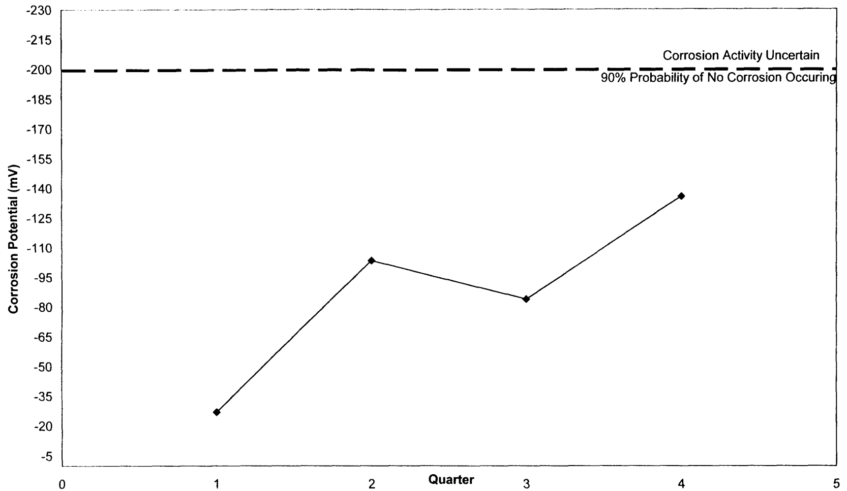
Fig. 4.18: Wyckoff Raod Westbound GECOR 6 Average Corrosion Potential (mV)
