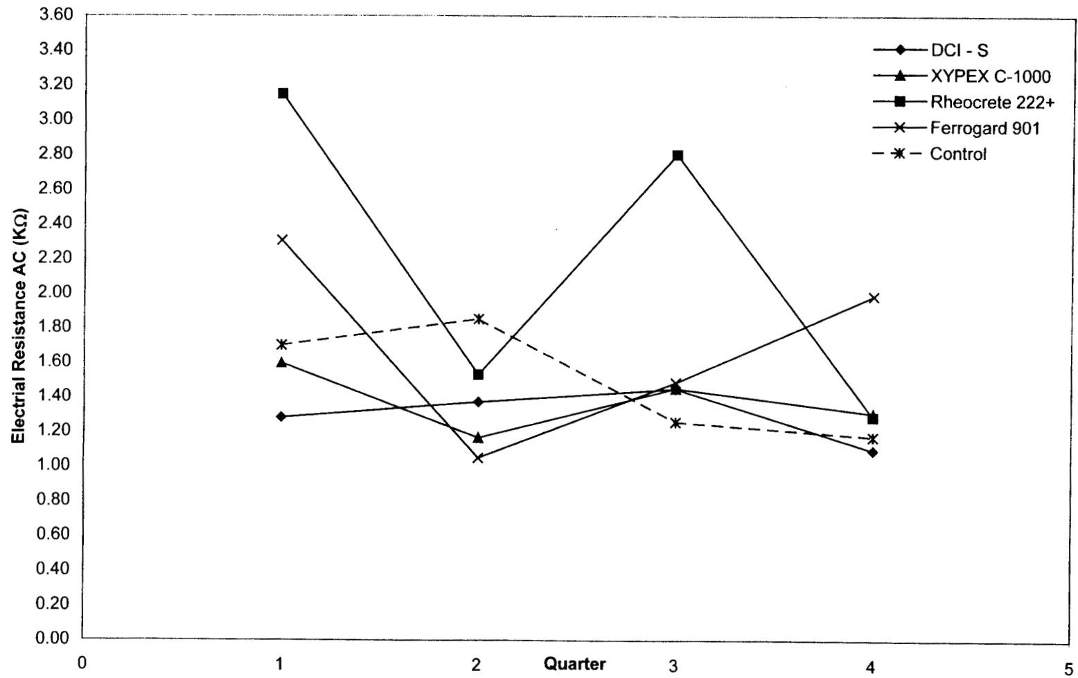
Fig. 4.40: Comparison of Corrosion Inhibitors GECOR 6 Average Electrical Resistance AC (KΩ)
