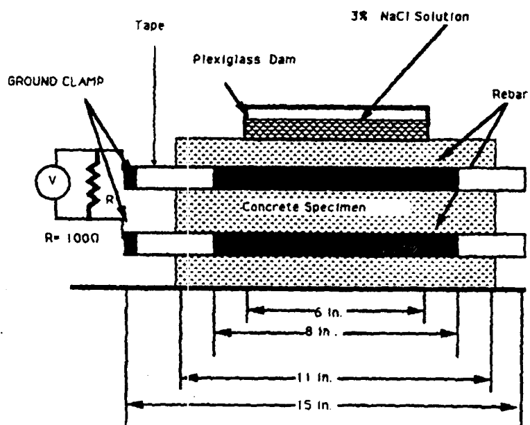
Fig. 3.10: View of Concrete Minideck (ASTM G 109)
