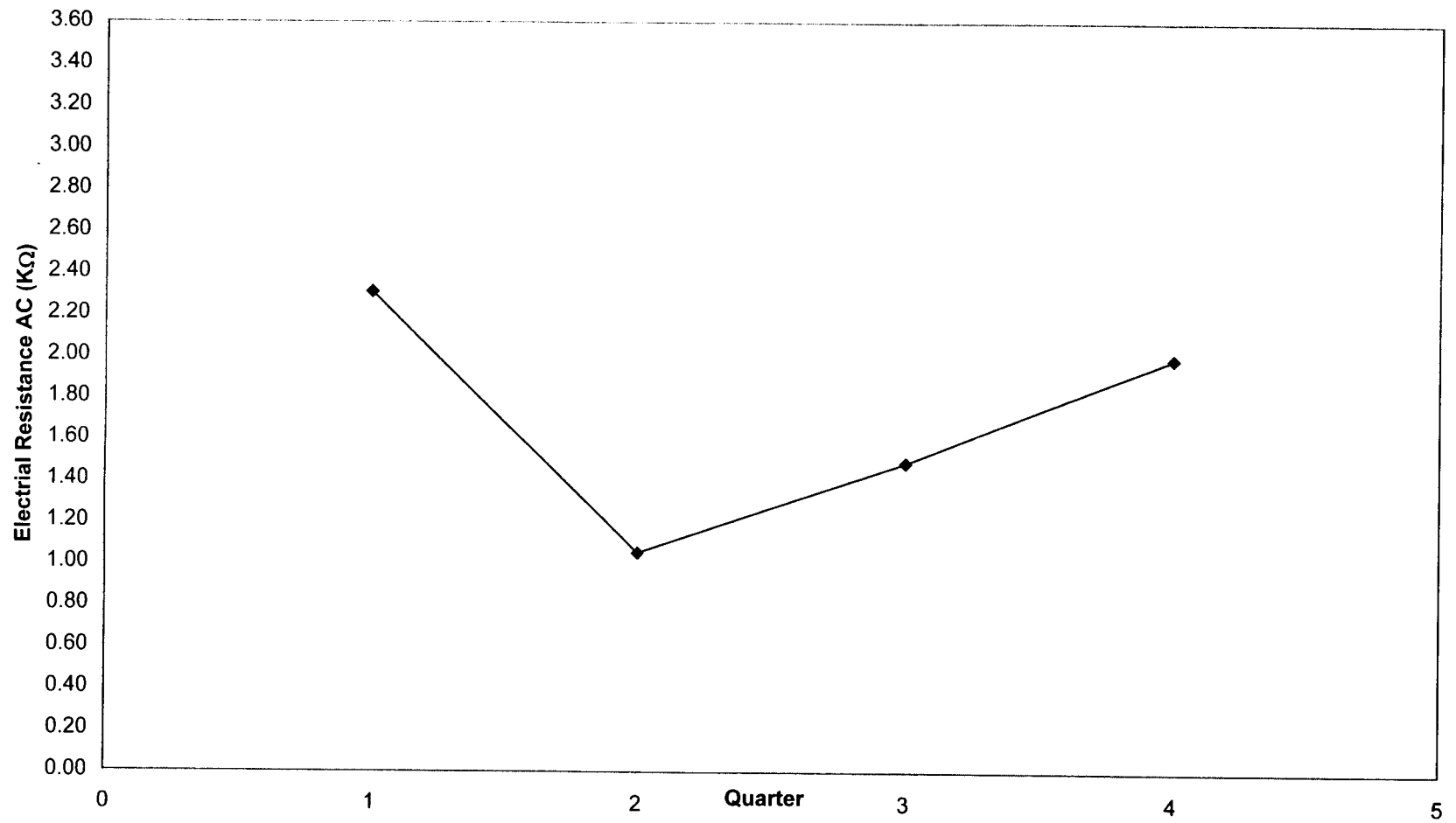
Fig. 4.26: Wyckoff Road Eastbound GECOR 6 Average Electrical Resistance AC (KΩ)
