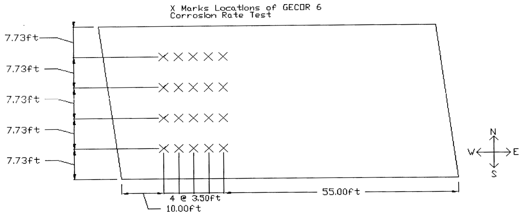
Fig. 3.11: Locations of GECOR 6 Corrosion Rate Meter Tests North Main Street Westbound
