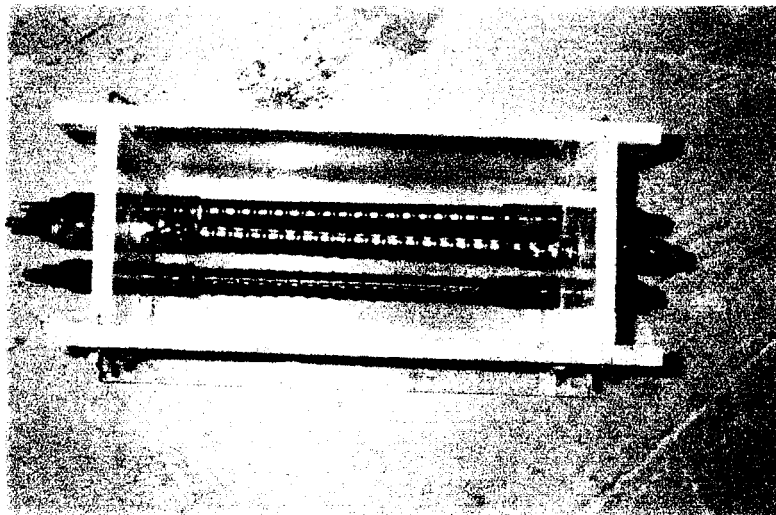
Fig. 3.46: Prepared Minideck Mold
