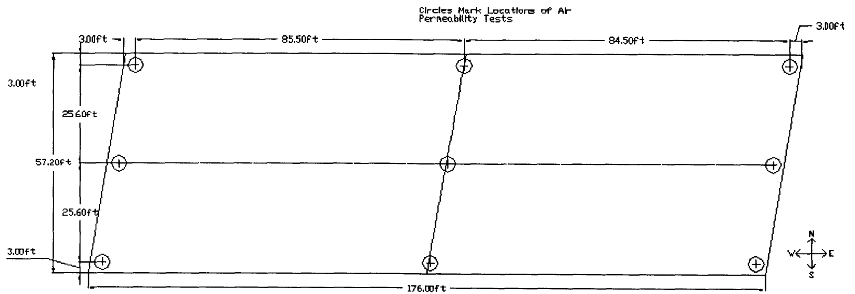
Fig. 3.40: Locations of Surface Air Flow Permeability Indicator Readings Route 130 Westbound
