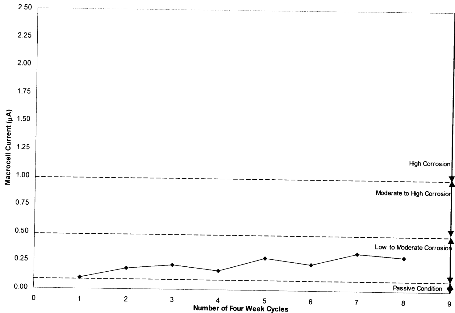
Fig. 4.8: Minideck B - Average Corrosion Rate Macrocell Current ( \mu\text{A} )
