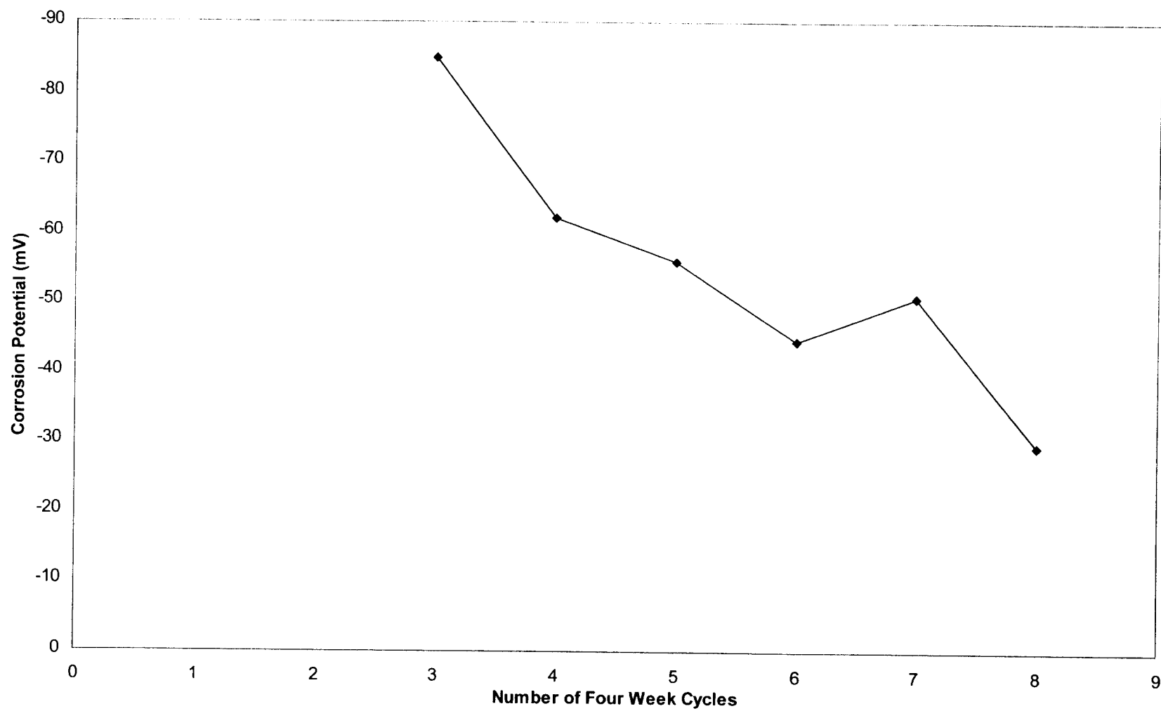
Fig. 4.30: Minideck E - Average Corrosion Potential (mV)
