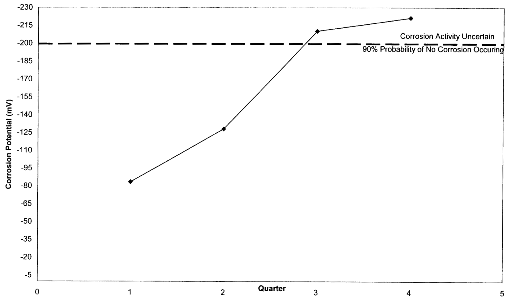
Fig. 4.4: North Main Street Westbound GECOR 6 Average Corrosion Potential (mV)
