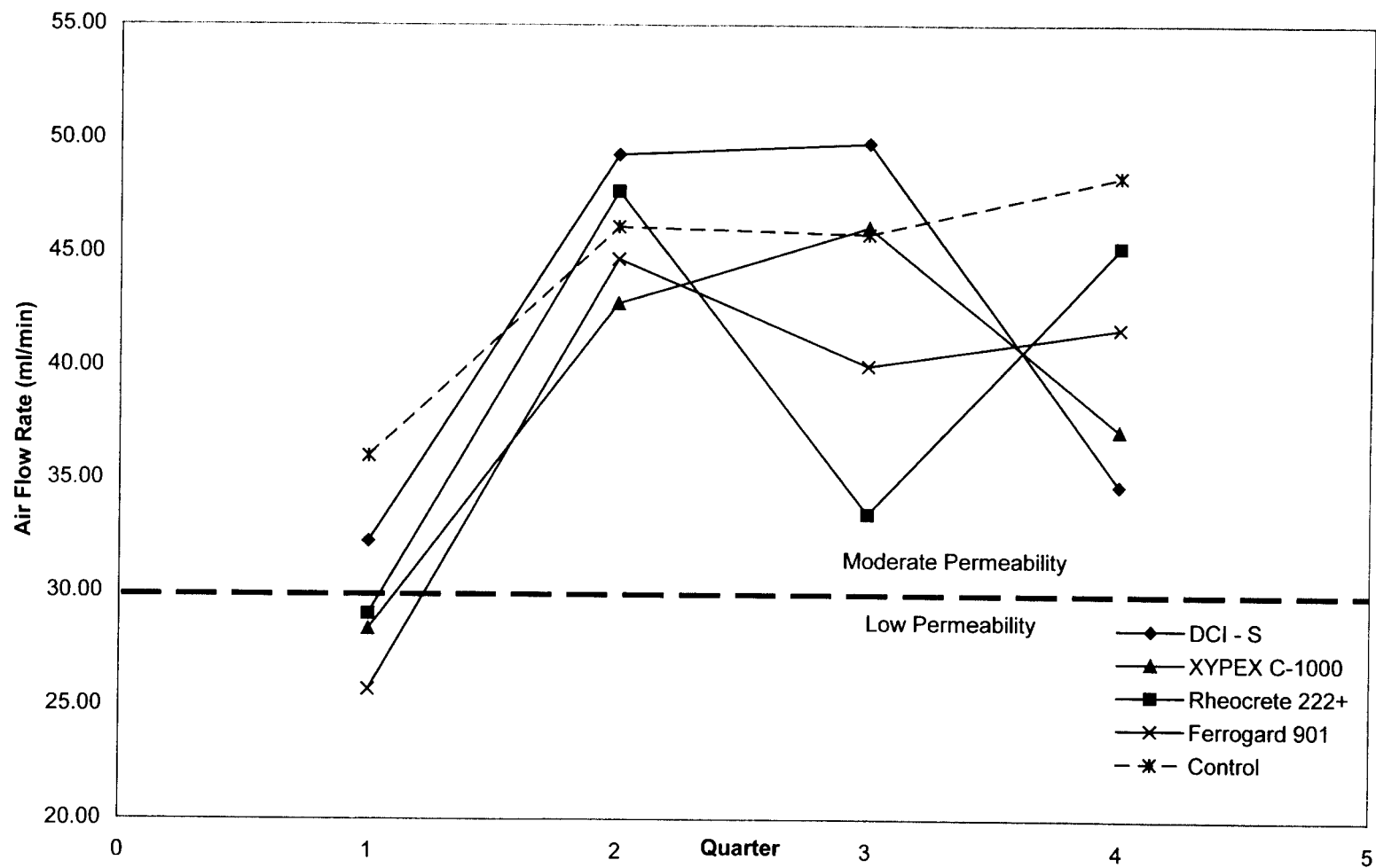
Fig. 4.41: Comparison of Corrosion Inhibitors Average Air Flow Rate (ml/min)
