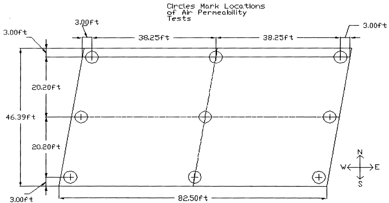
Fig. 3.38: Locations of Surface Air Flow Permeability Readings Wyckoff Road Westbound
