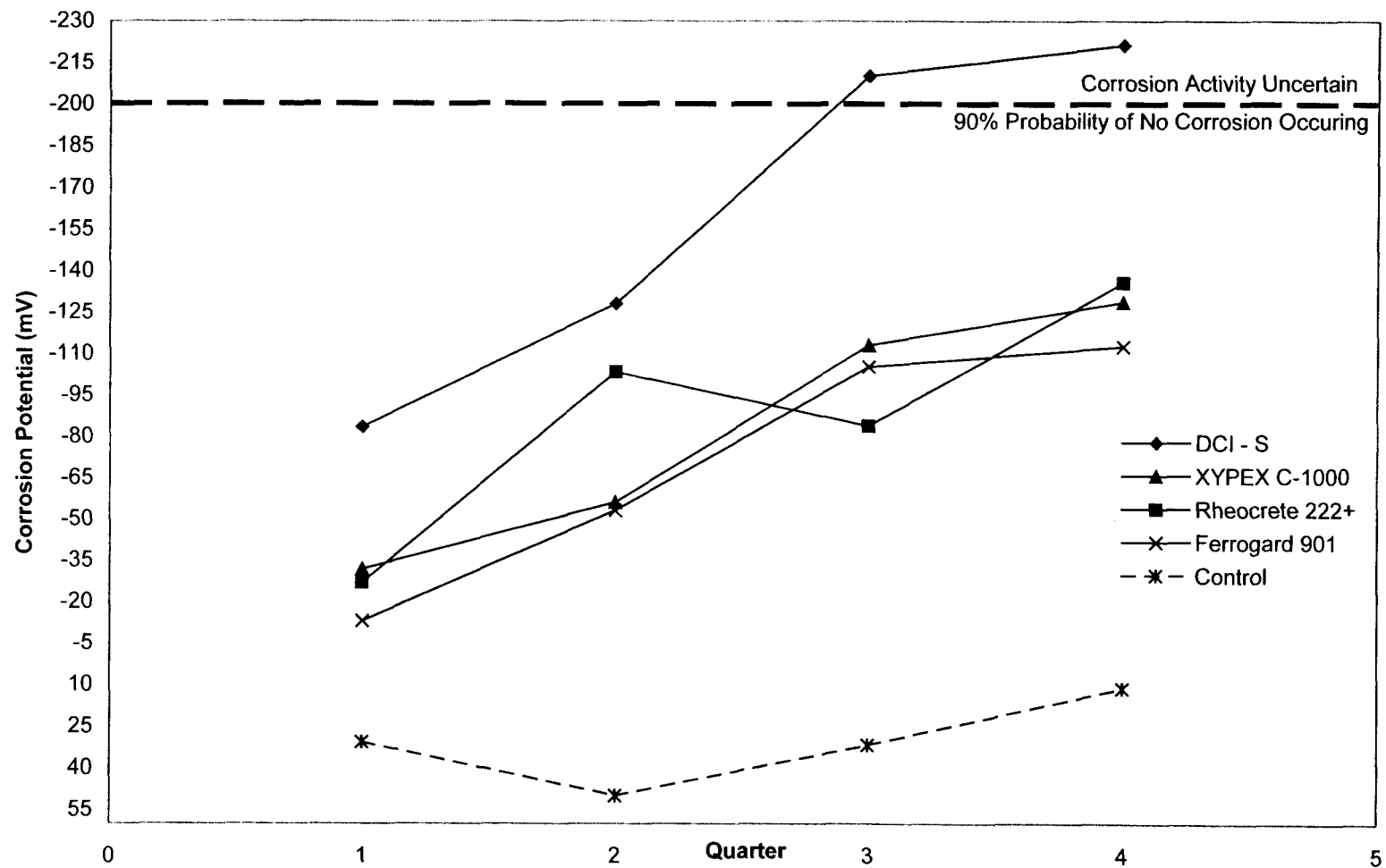
Fig. 4.39: Comparison of Corrosion Inhibitors GECOR 6 Average Corrosion Potential (mV)
