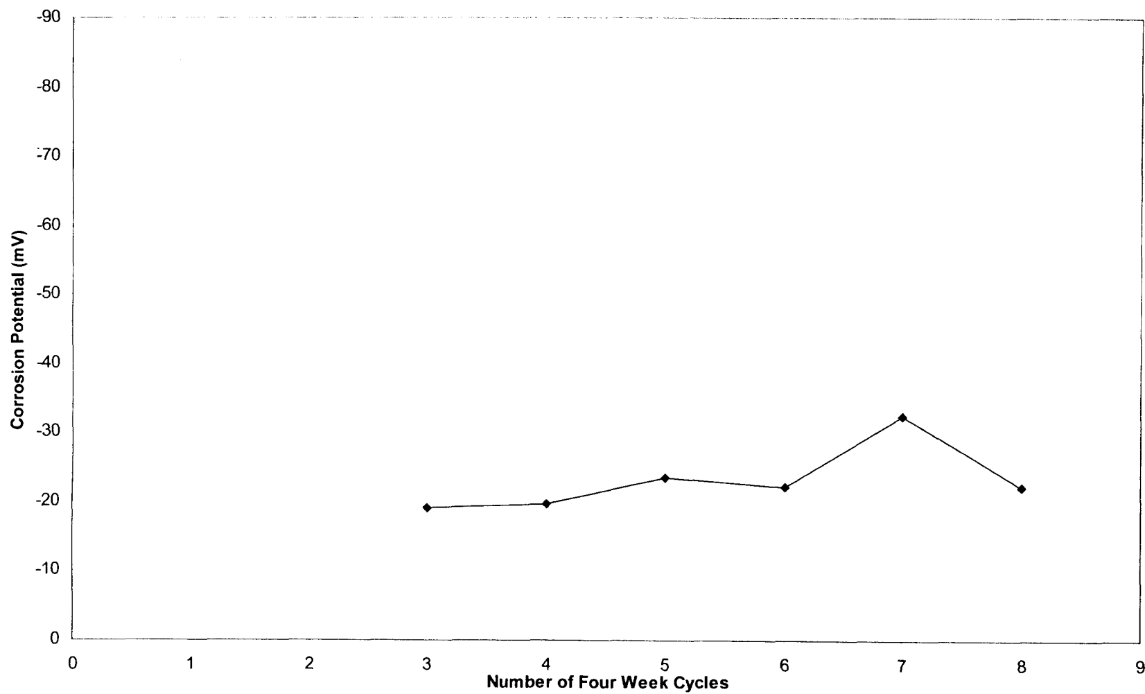
Fig. 4.9: Minideck B - Average Corrosion Potential (mV)
