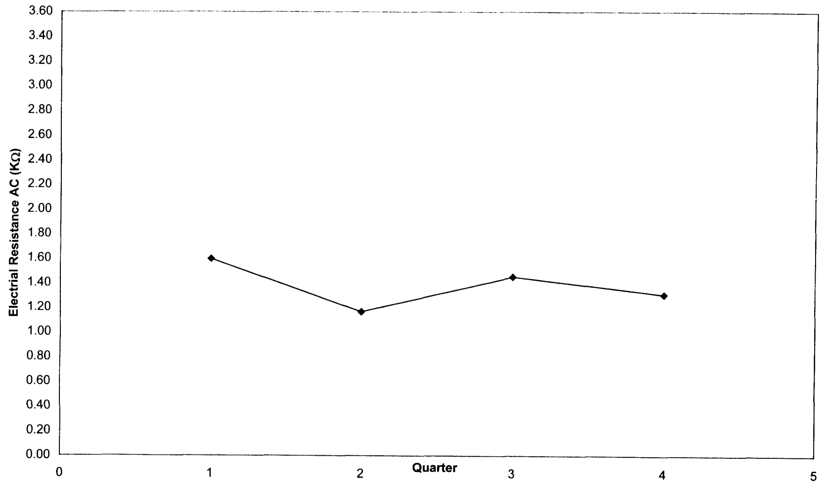
Fig. 4.12: North Main Street Eastbound GECOR 6 Average Electrical Resistance AC (KΩ)
