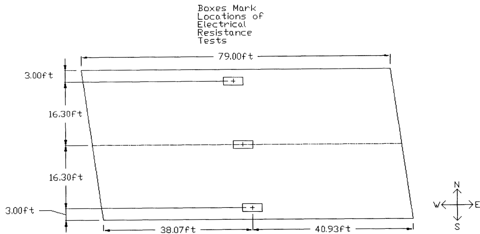
Fig. 3.42: Locations of Electrical Resistance Tests North Main Street Eastbound
