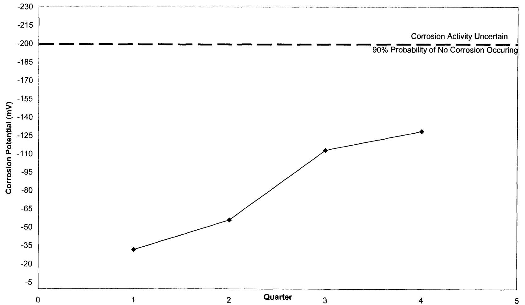
Fig. 4.11: North Main Street Eastbound GECOR 6 Average Corrosion Potential (mV)
