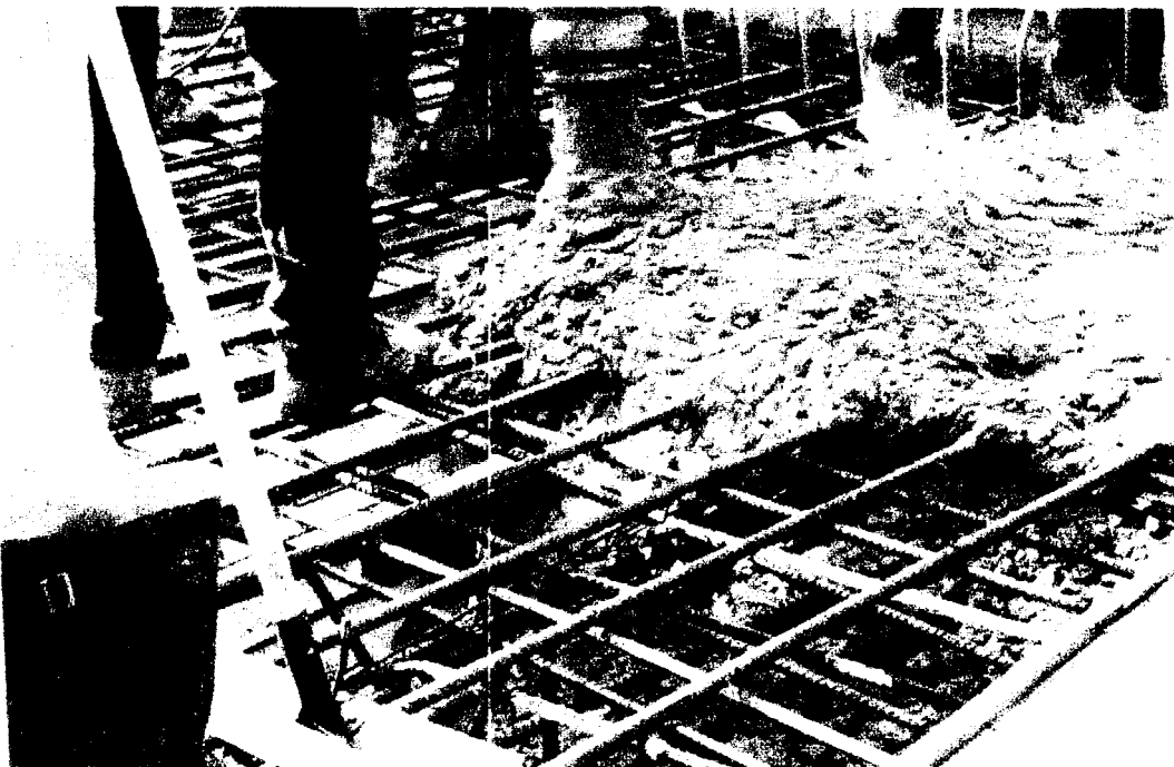
Fig. 3.29: Placement on Fresh Concrete at North Main Street Westbound
