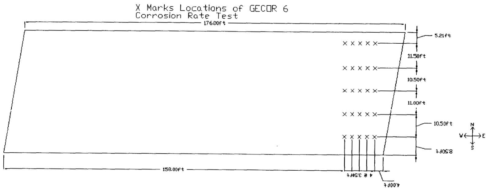
Fig. 3.15: Locations of GECOR 6 Corrosion Rate Meter Tests Route 130 Westbound
