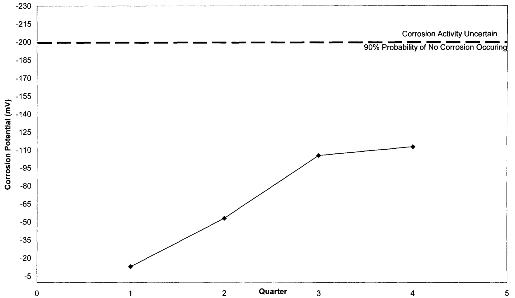
Fig. 4.25: Wyckoff Road Eastbound GECOR 6 Average Corrosion Potential (mV)
