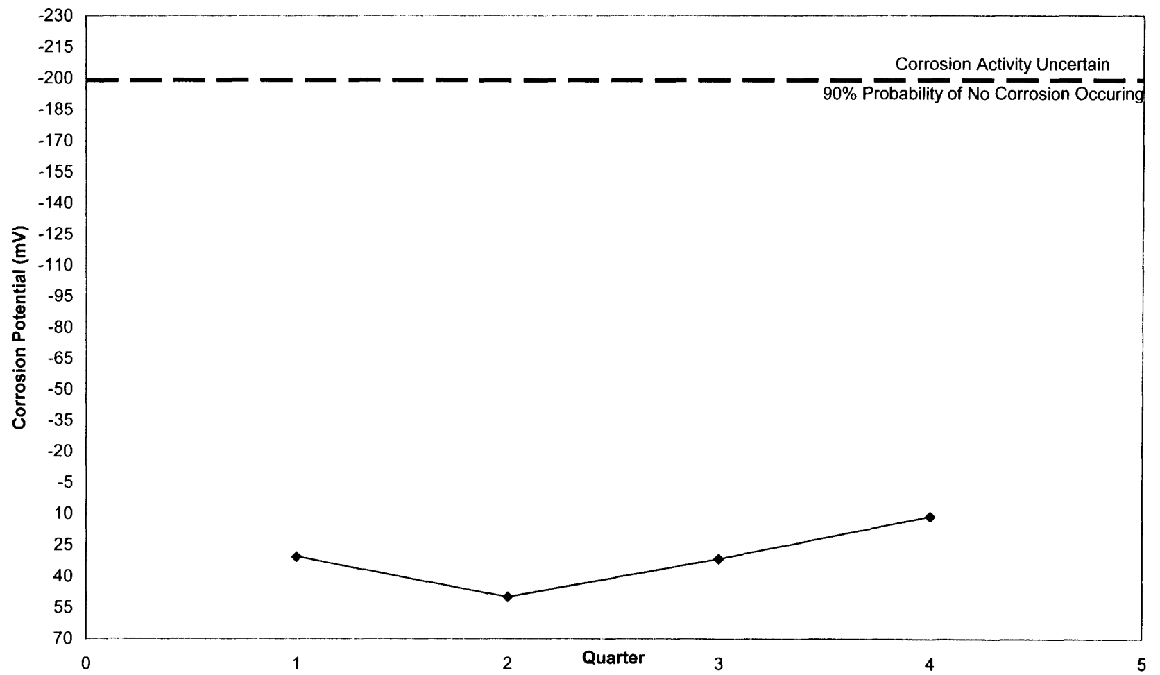
Fig. 4.32: Route 130 Westbound GECOR 6 Average Corrosion Potential (mV)
