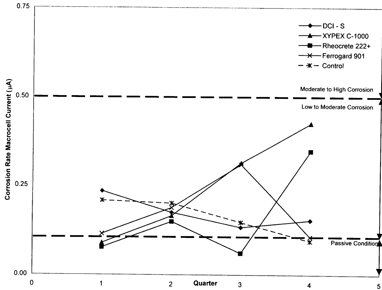
Fig. 4.38: Comparison of Corrosion Inhibitors GECOR 6 Average Corrosion Rate Macrocell Current ( \mu\text{A} )
