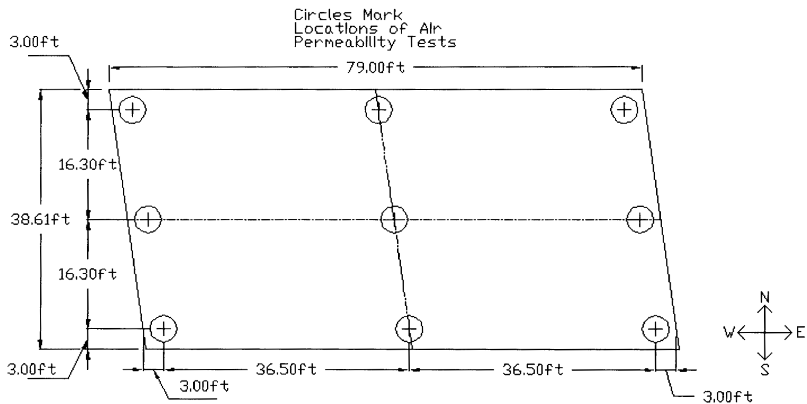
Fig. 3.37: Locations of Surface Air Flow Permeability Indicator Readings North Main Street Eastbound
