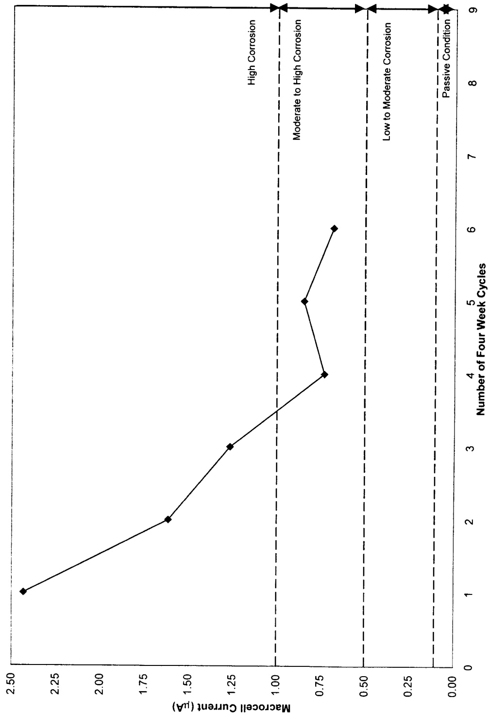
Fig. 4.29: Minideck E - Average Corrosion Rate Macrocell Current ( \mu\text{A} )
