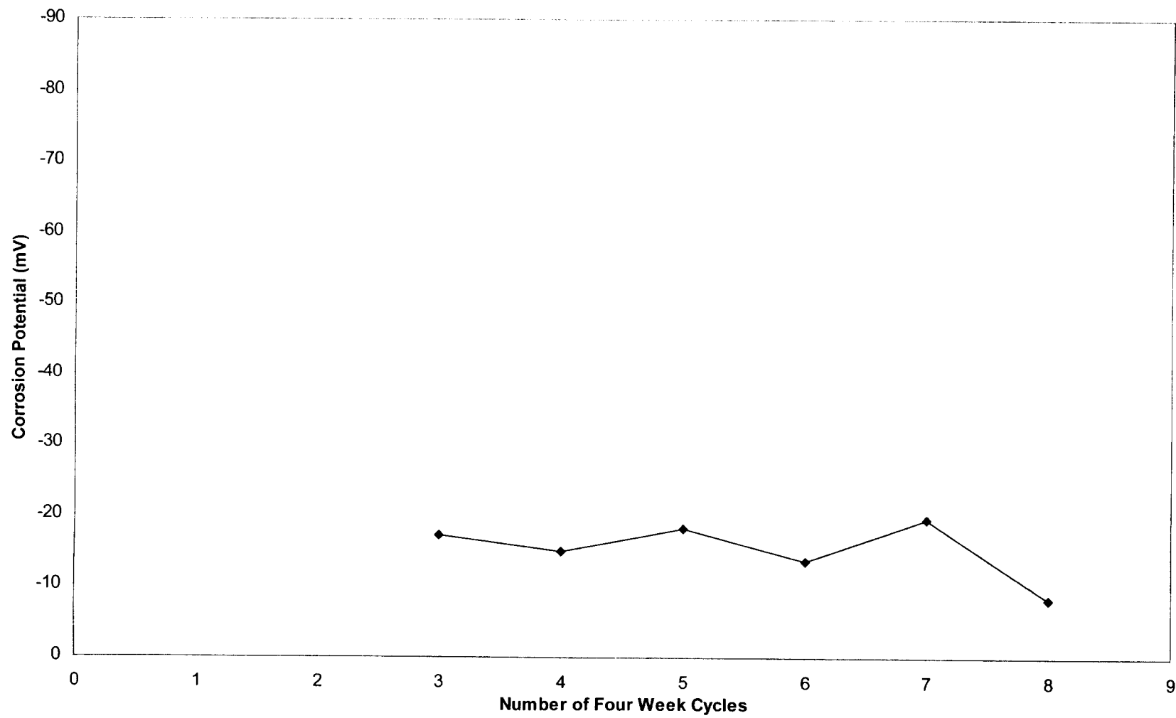
Fig. 4.23: Minideck D - Average Corrosion Potential (mV)
