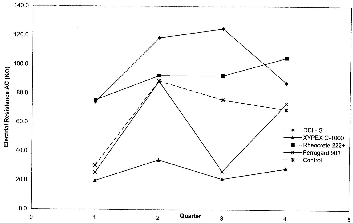
Fig. 4.42: Comparison of Corrosion Inhibitors Average Electrical Resistance AC (KΩ)
