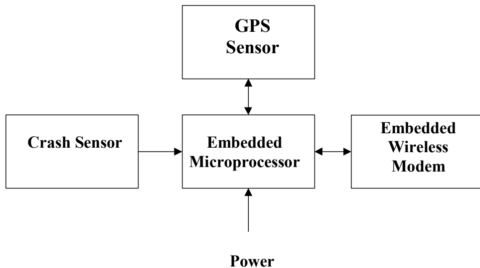
Figure 3-1. System Architecture
