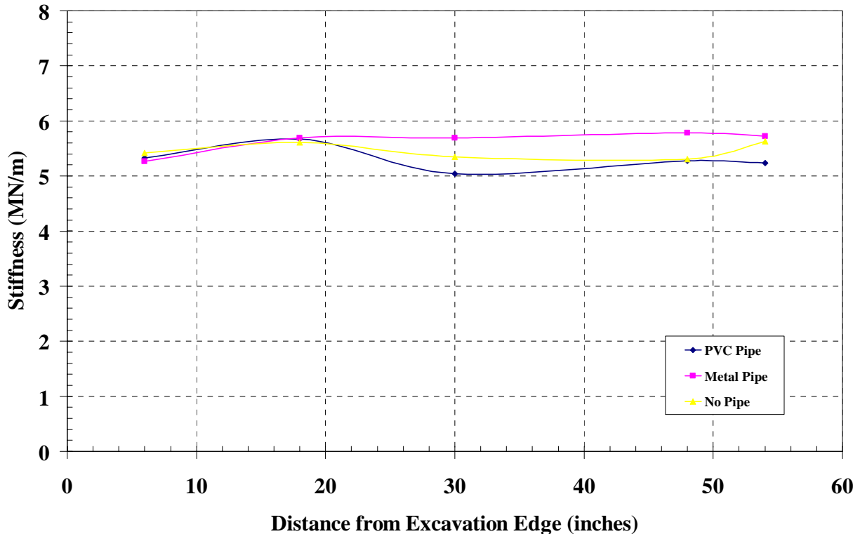
Figure 20 - Large Bin Measurements with Pipes Buried Six Inches Below Surface
