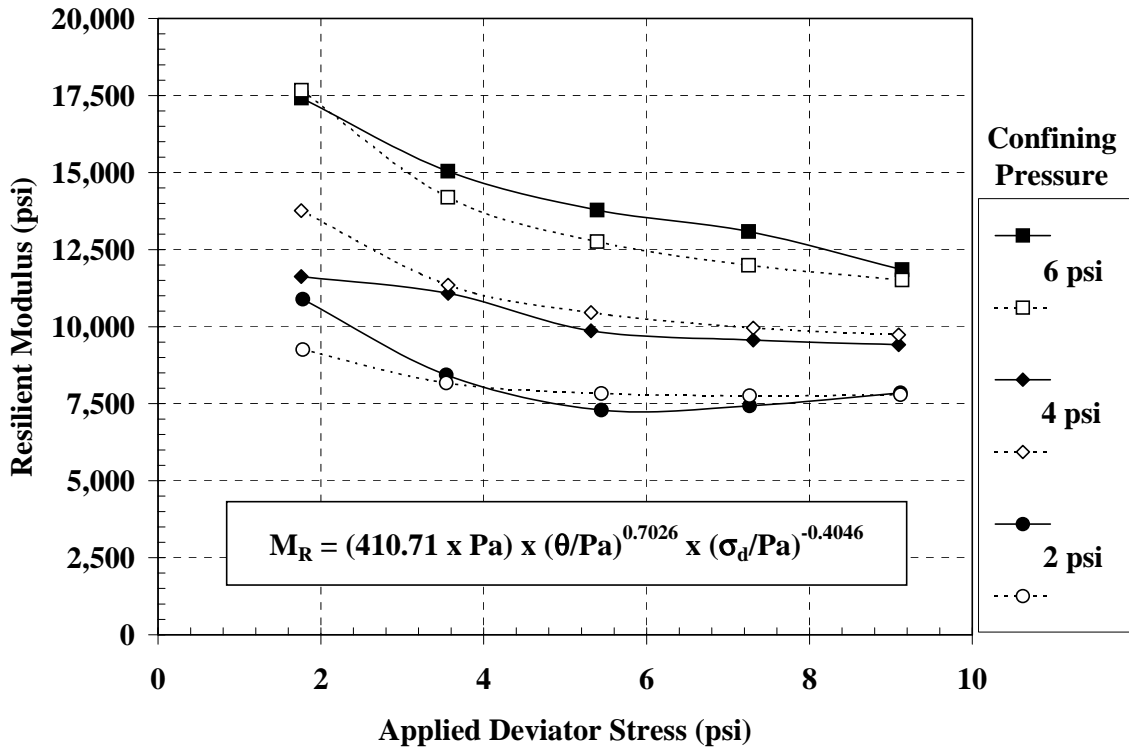
Figure 7 – Resilient Modulus Results of Soil #1
