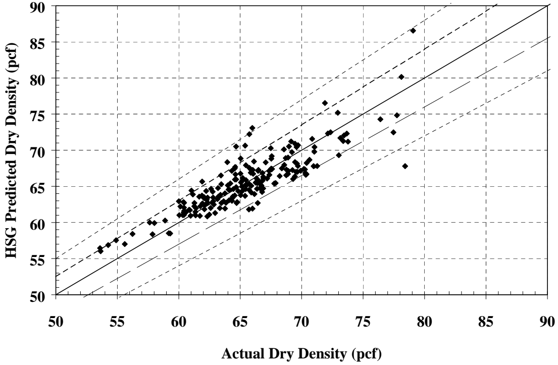
Figure 28 – Dry Density Comparison for Embankment #2
