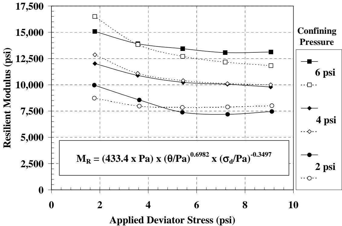
Figure 8 – Resilient Modulus Results of Soil #2
