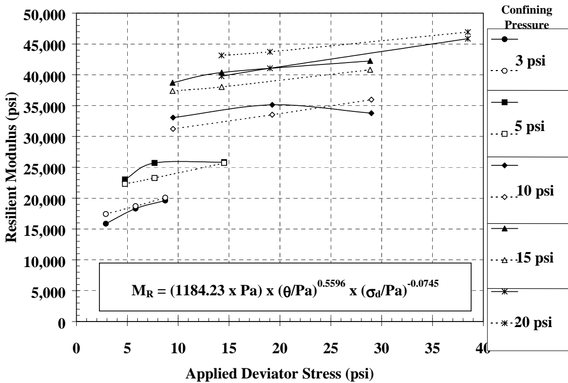
Figure 10 – Resilient Modulus Results of CJ I-3
