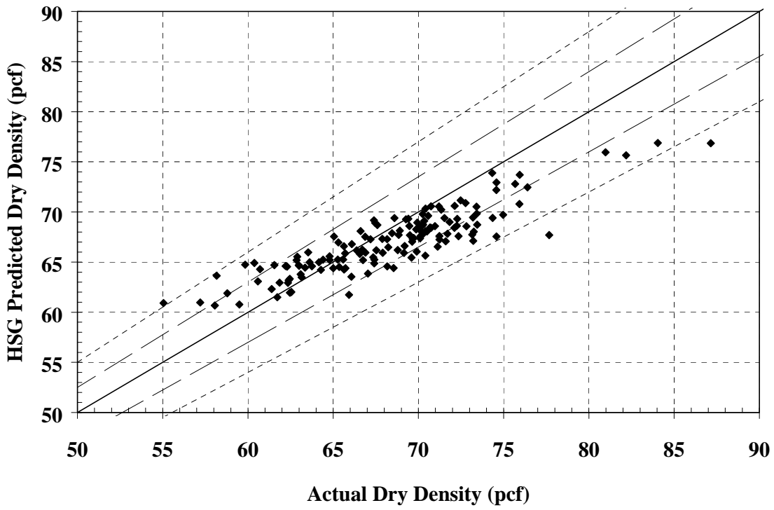
Figure 27 – Dry Density Comparison for Embankment #1
