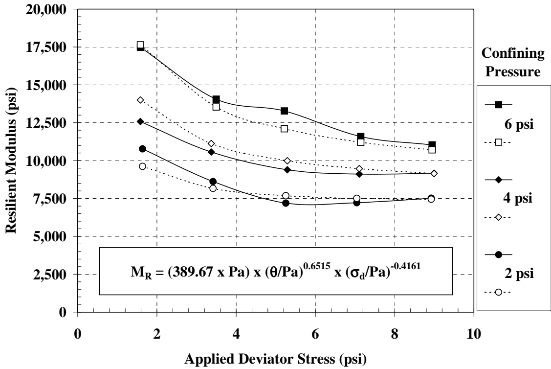
Figure 9 – Resilient Modulus Results of Soil #3
