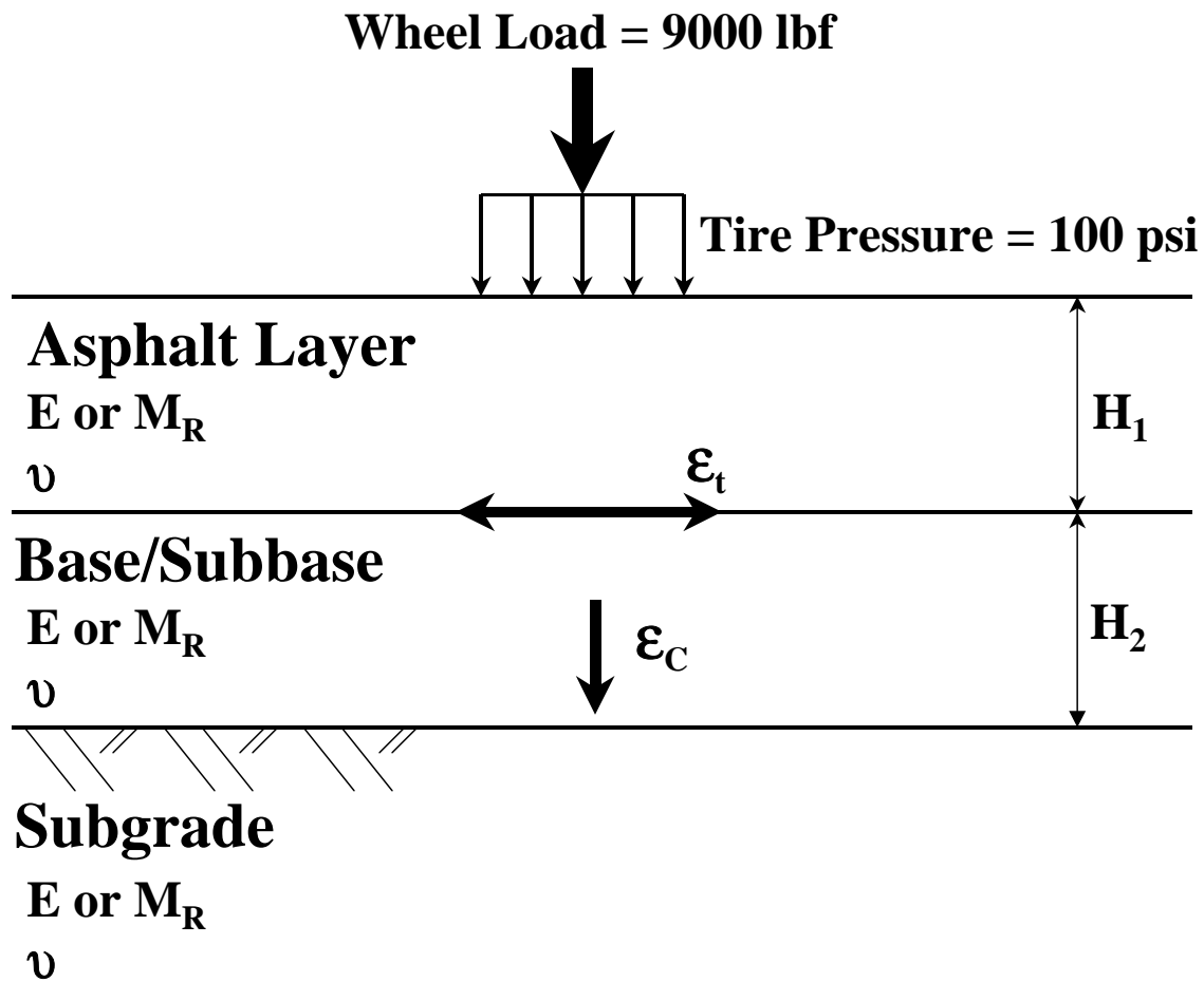
Figure 3 – Typical Mechanistic Pavement Design Characterization
