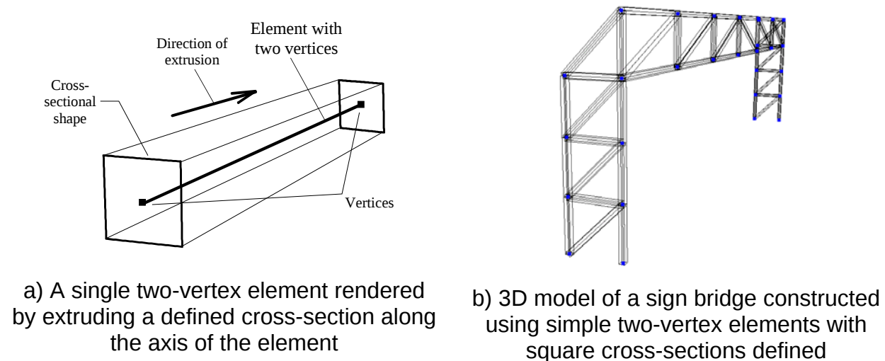
Figure 11. Use of cross-sectional extrusion to model a sign bridge structure.
