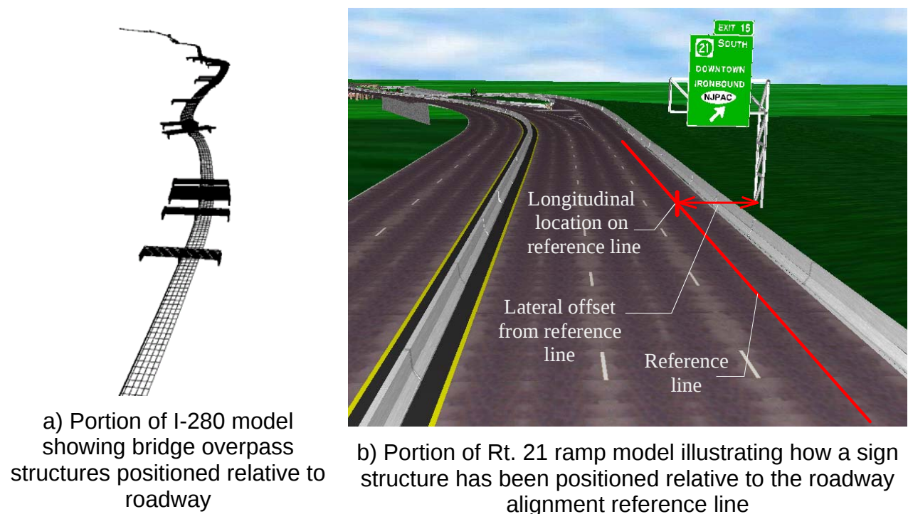
Figure 12. Using roadway alignment data to position roadside objects.
