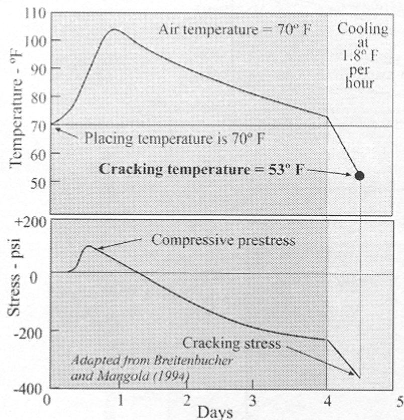
Figure 29. Typical results of cracking frame test (from Burrows, 1998).
