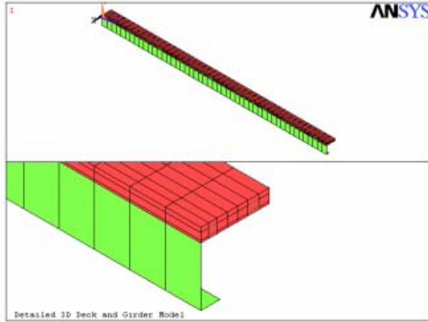
Figure 52. 3D finite element model.
