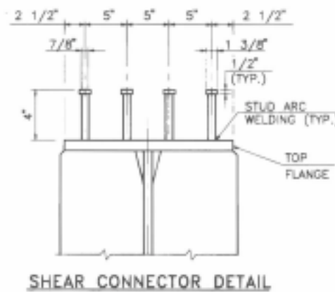
Figure 54. Shear Connector Detail.
