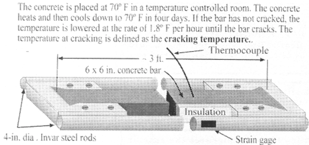
Figure 28. Cracking frame developed in Germany (from Burrows, 1998).
