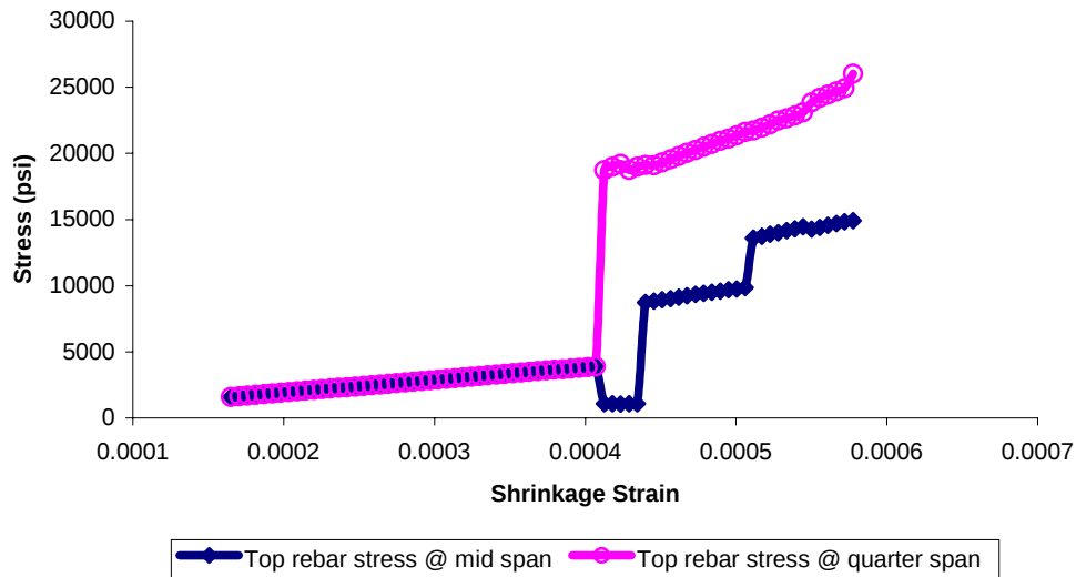
Figure 70. Reinforcement stress over girder at mid span and quarter span for pin-roller boundary condition.
