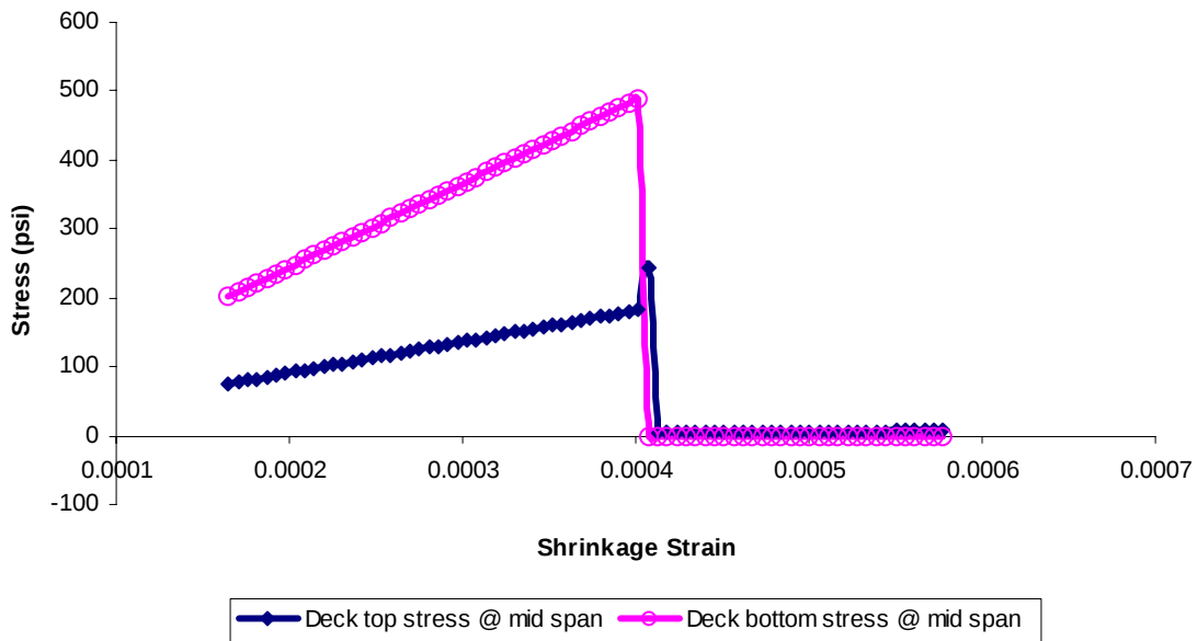
Figure 61. Deck top and bottom stress over girder at mid span for pin-roller boundary condition.
