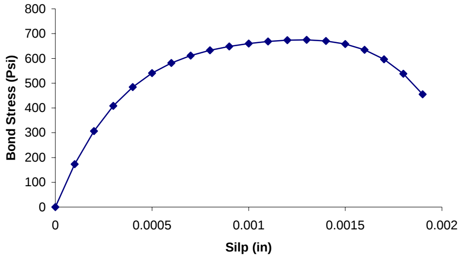
Figure 53. Bond-slip relationship (Houde, 1973).
