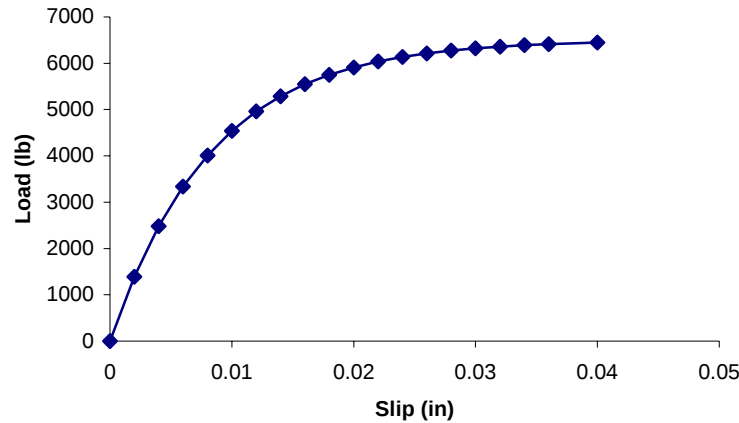
Figure 55. Shear Connector load slip behavior (Yam and Chapman, 1968).
