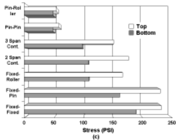
Figure 51. Deck top and bottom stresses for different boundary conditions and (a) shrinkage profile 1, (b) shrinkage profile 2, (c) shrinkage profile 3.
