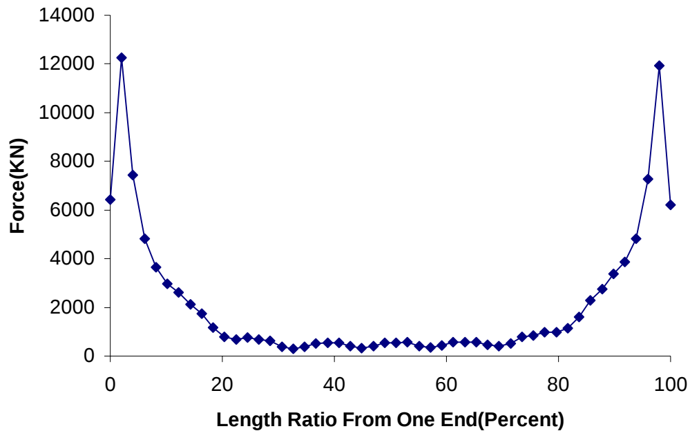
Figure 32. Lateral nodal forces along the deck assuming uniform displacements.
