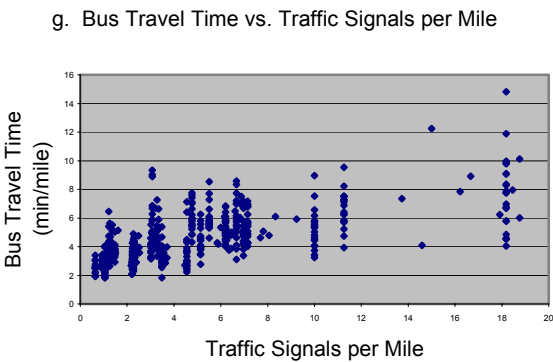
Figure 3. Relation of Bus Travel Time to Other Variables
