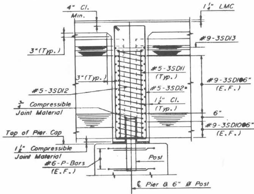
(b) Section
