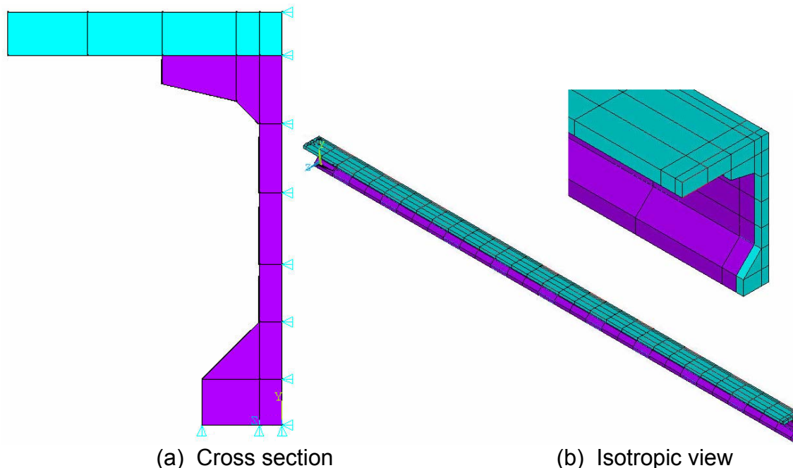
Figure 47. Finite element model.
