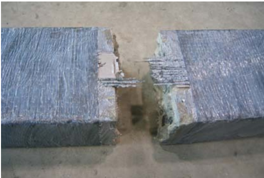
(c) CFRP rupture (beam9)
