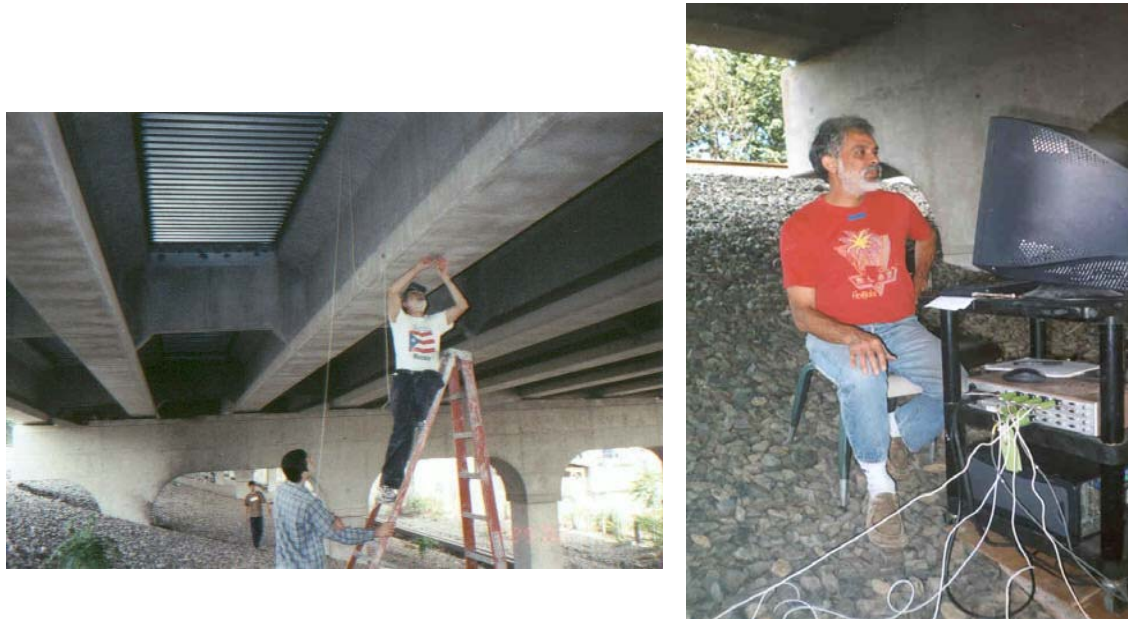
Figure 27. Installing strain gage at mid-span and monitoring responses.
