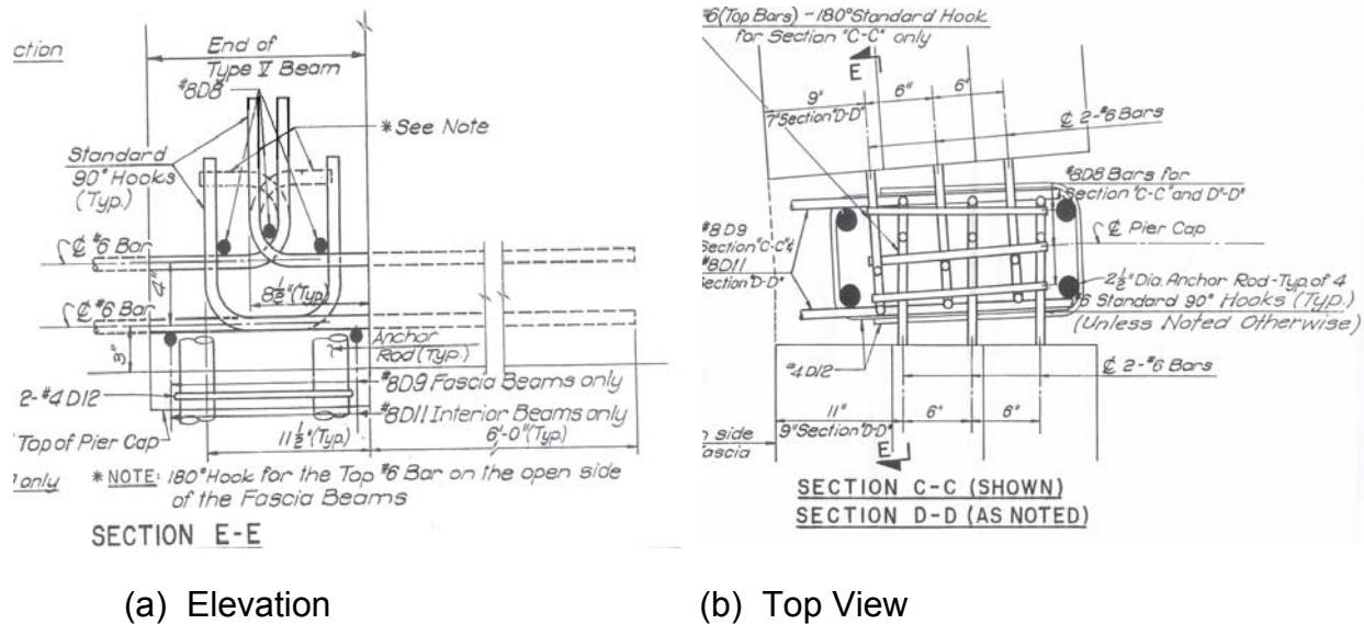
Figure 26. Diaphragm details at fixed piers (Rt. 1&9 design drawings).
