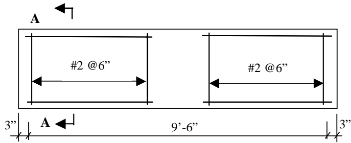
Elevation (Not to Scale)
