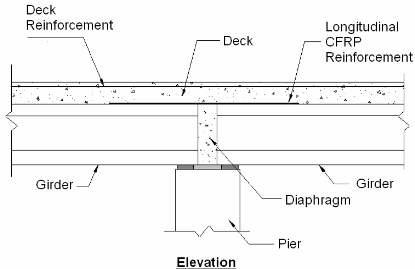
Figure 68. New connection.
