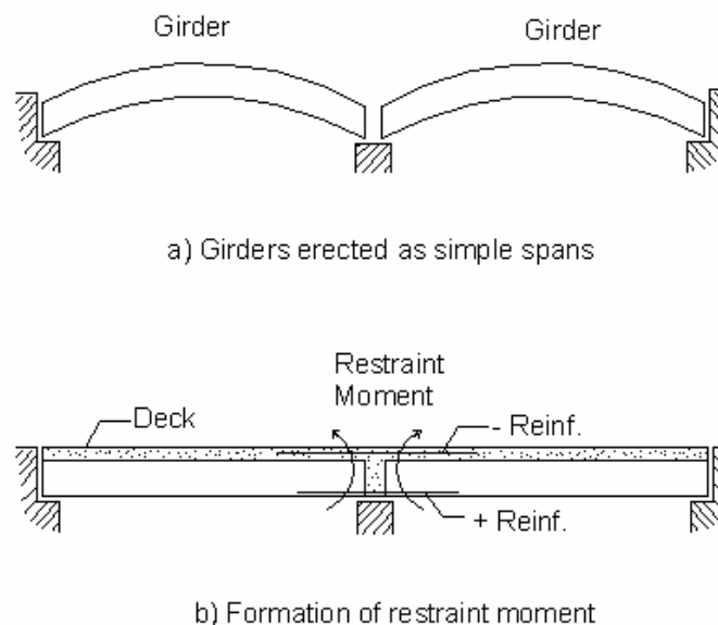
Figure 1. Formation of positive restraint moment under time dependent effects.
