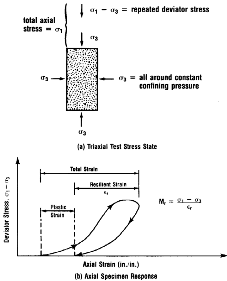
Figure 24 - Definition of Resilient Modulus (Barksdale, 1993)
