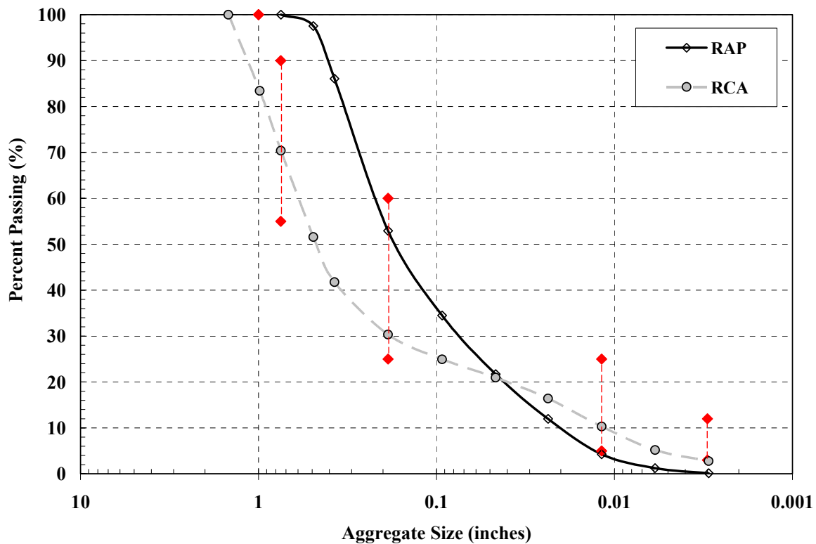
Figure 6 – RAP and RCA Gradations Shown with the DGABC Gradation Bands
