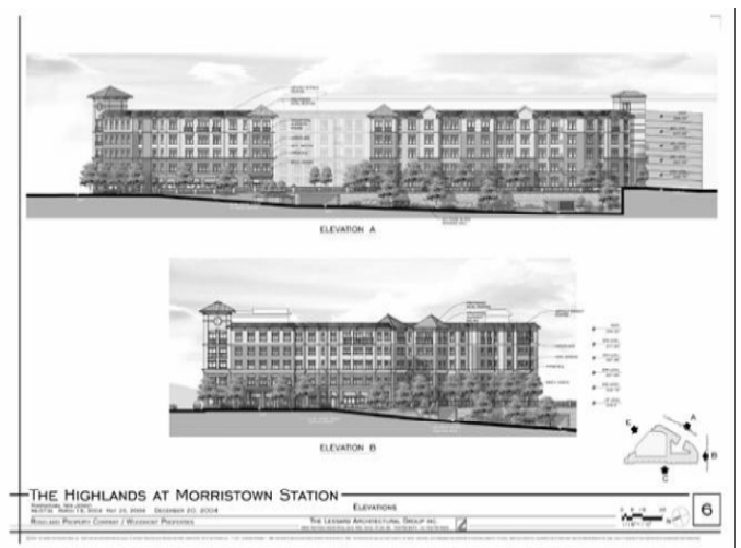
Elevations
