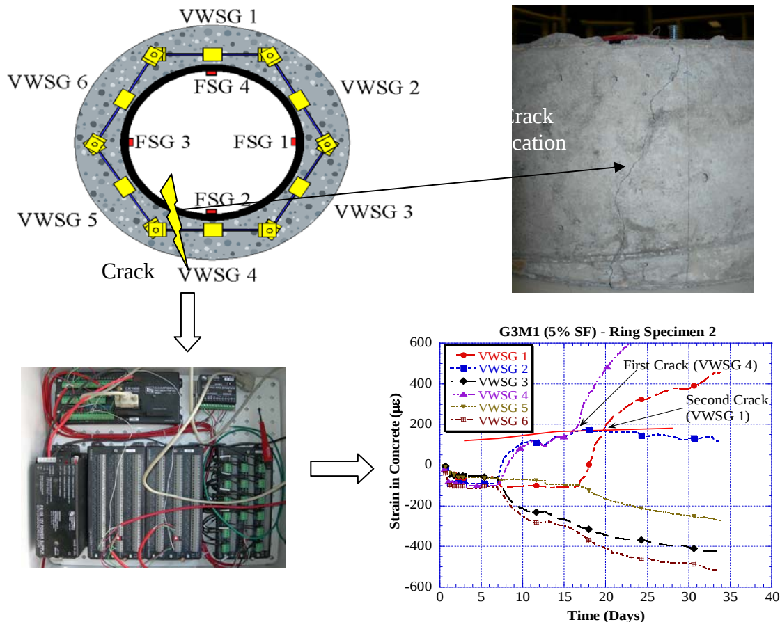
Figure 2. Schematic of the restrained shrinkage test setup, data collection schemes, and test results.
