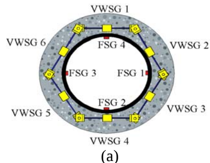
Figure 1. a) Schematic Diagram of Six VWSGs, and b) picture of the Six VWSG Restrained Shrinkage Test Setup.
