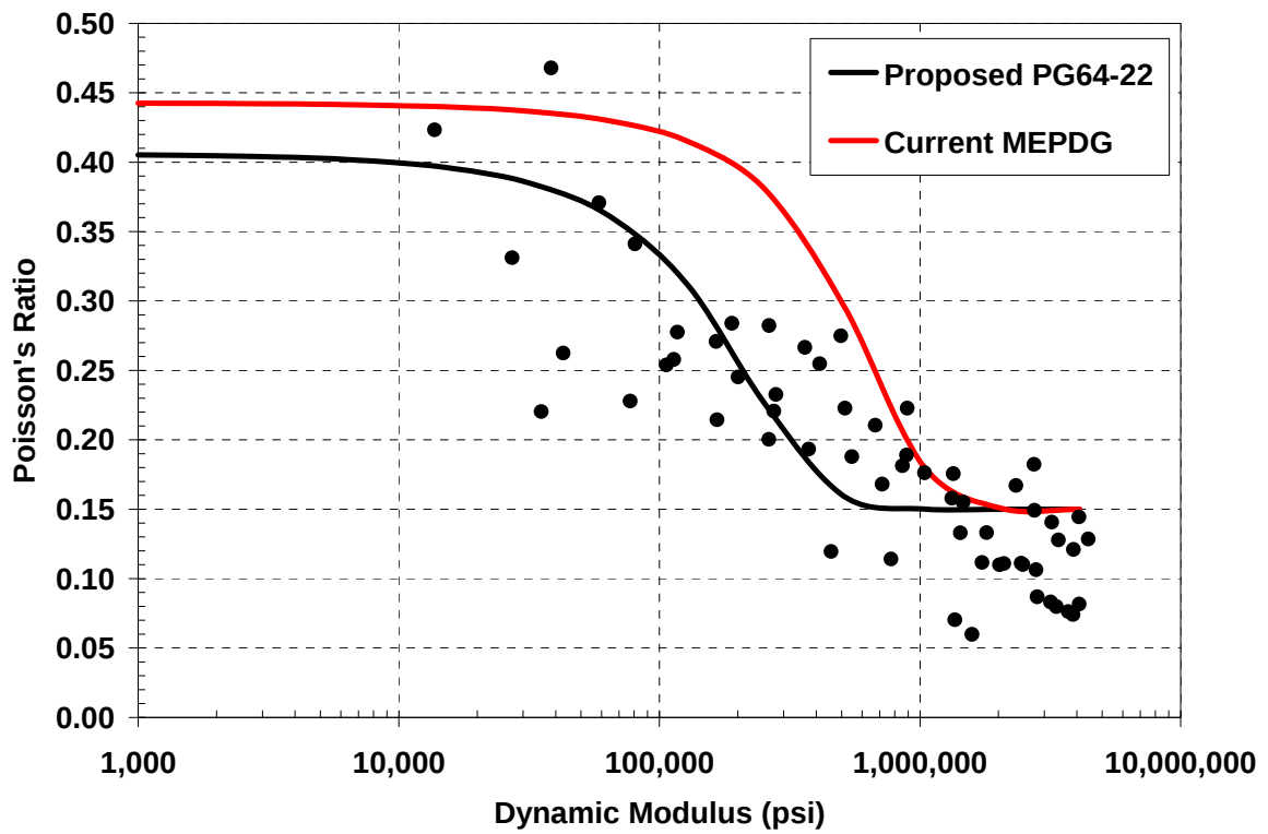
Figure 4a - Proposed PG64-22 Poisson's Ratio Prediction Equation
