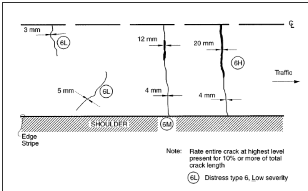
Figure 7. Transverse Cracking
