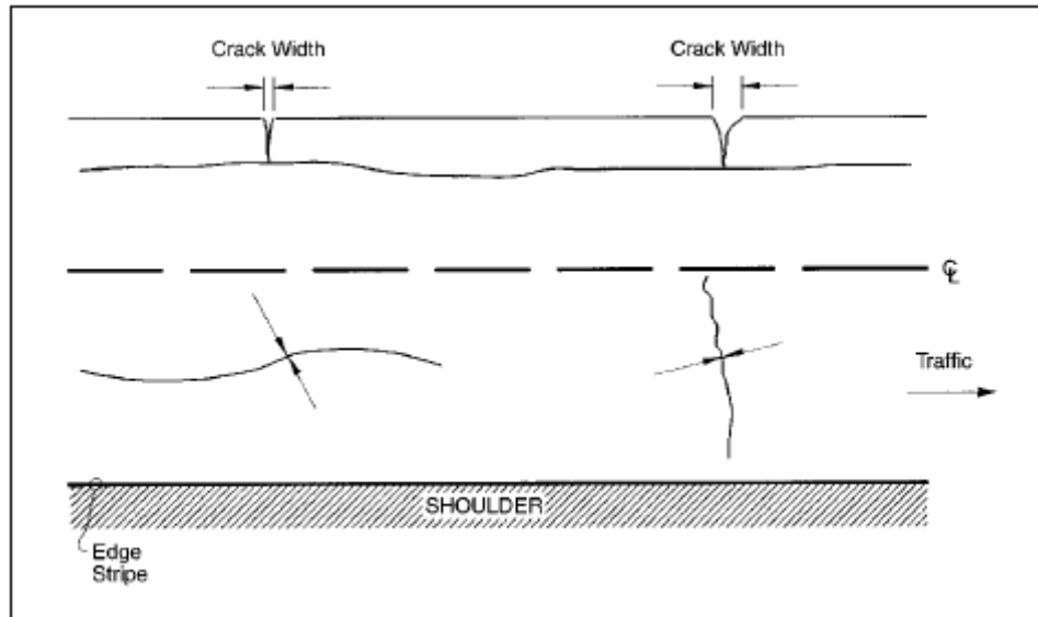
Figure 2. Measuring Crack Width in Asphalt Concrete-Surfaced Pavements
