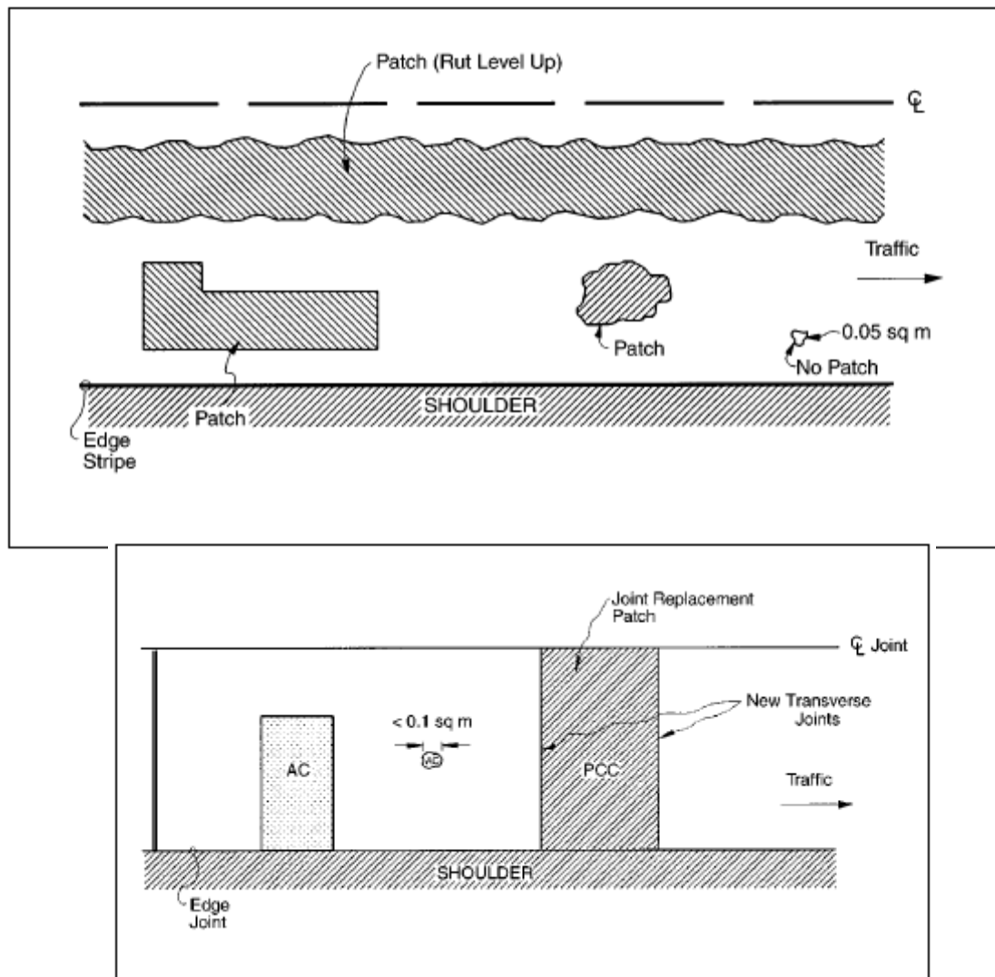
Figure 25. Patching
