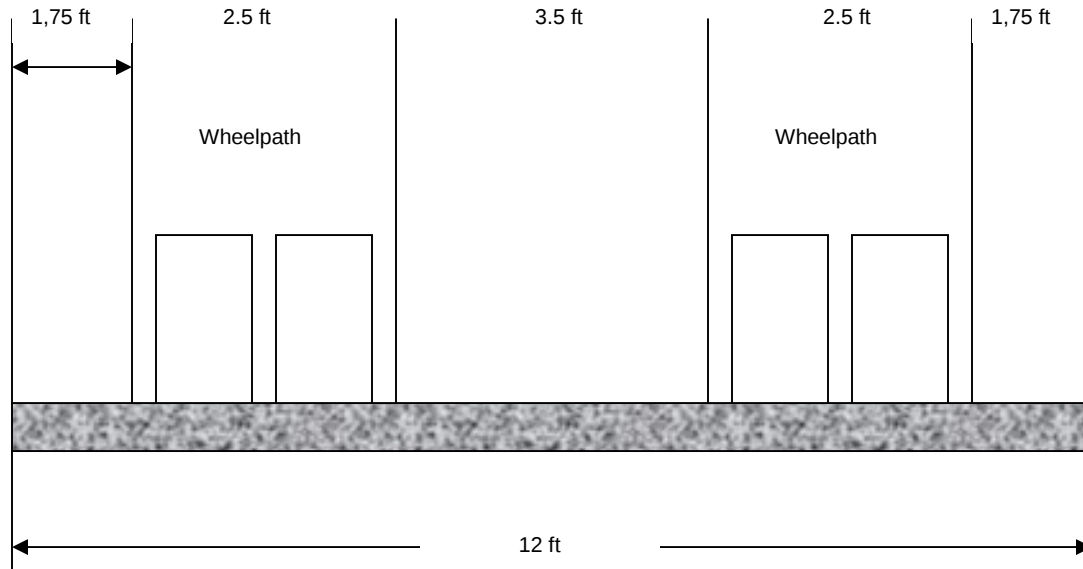
Figure 1. Locations of Wheelpaths for 12 Foot Lanes
