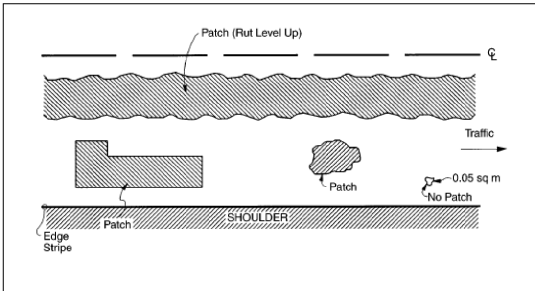
Figure 9. Patching
