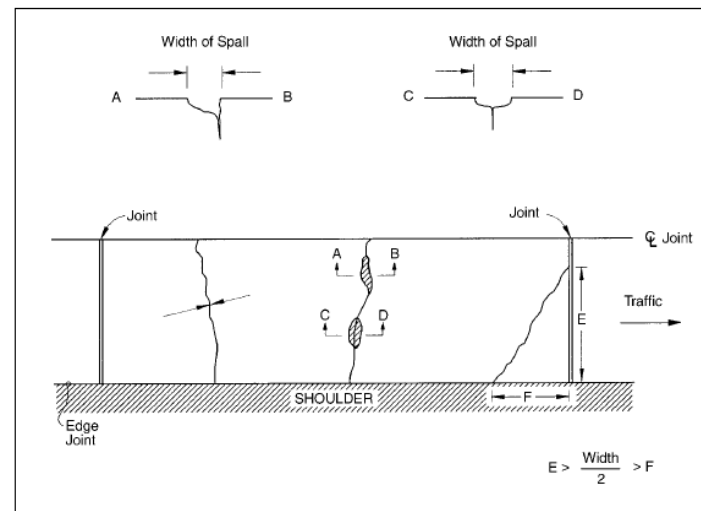
Figure 17. Transverse Cracking
