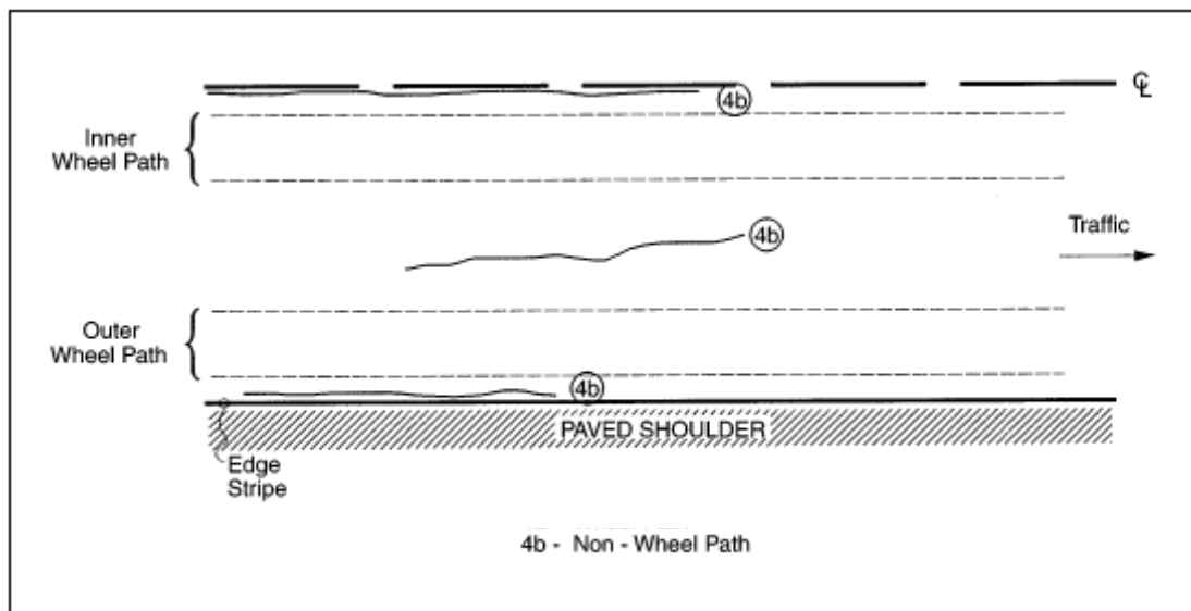
Figure 5. Non-Load Associated Longitudinal Cracking
