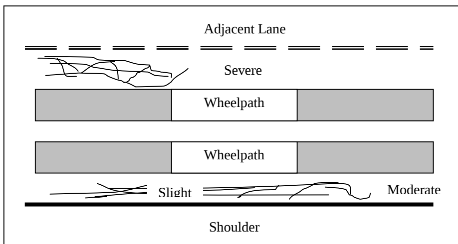
Figure 3. Multiple Cracking Levels
