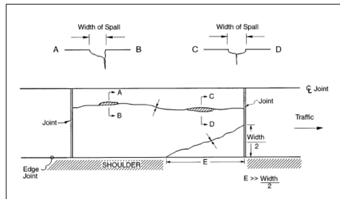
Figure 16. Longitudinal and Corner Cracking
