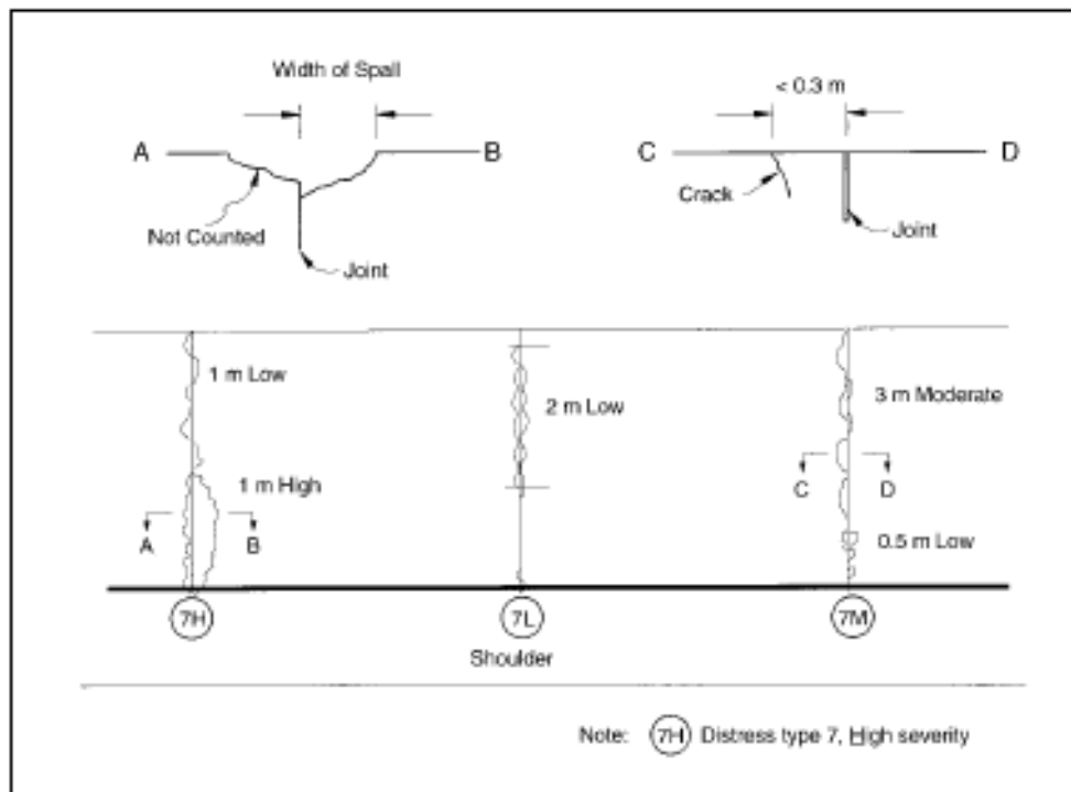
Figure 23. Spalling of Transverse Joints
