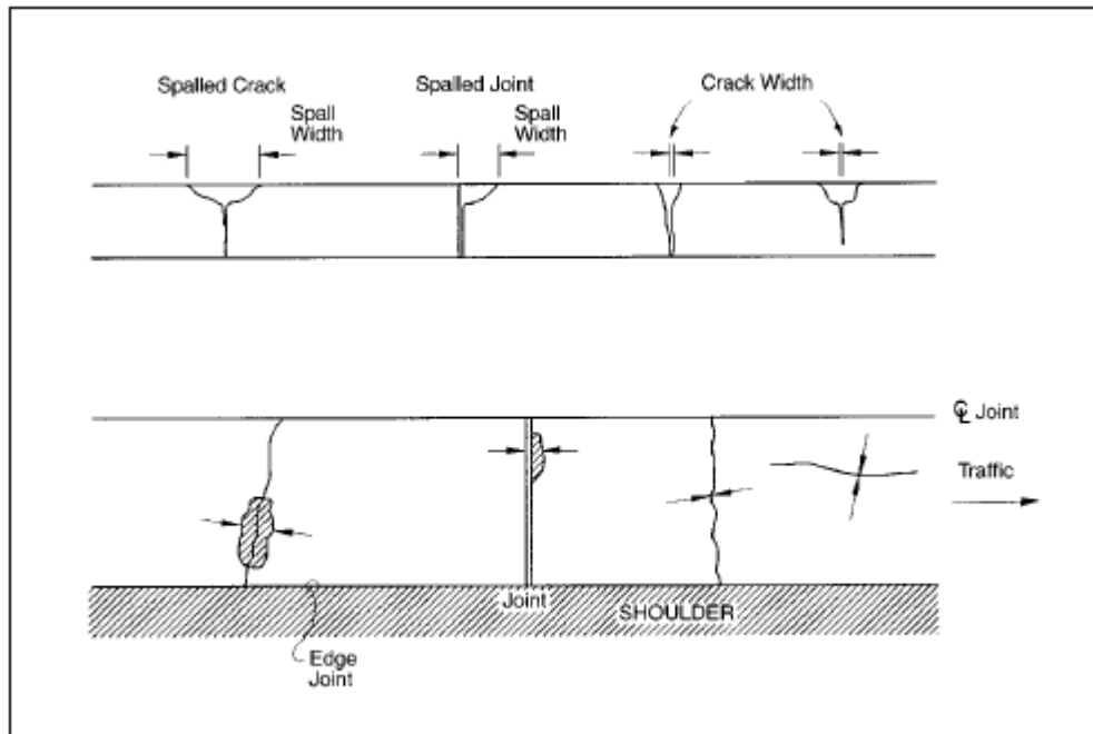
Figure 15. Measuring Widths of Spalls and Cracks in Jointed Concrete Pavement
