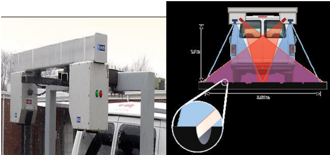
Figure 5. Dynatest-INO Imaging System
