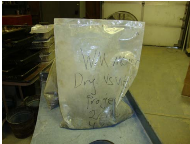
Figure 14. Aggregate Blend Saturating
