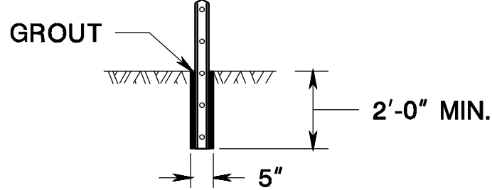
ROCK INSTALLATION
