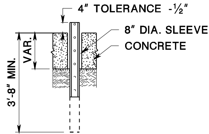
CONCRETE INSTALLATION
