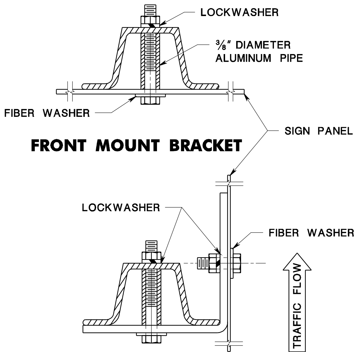
SIDE MOUNT BRACKET
