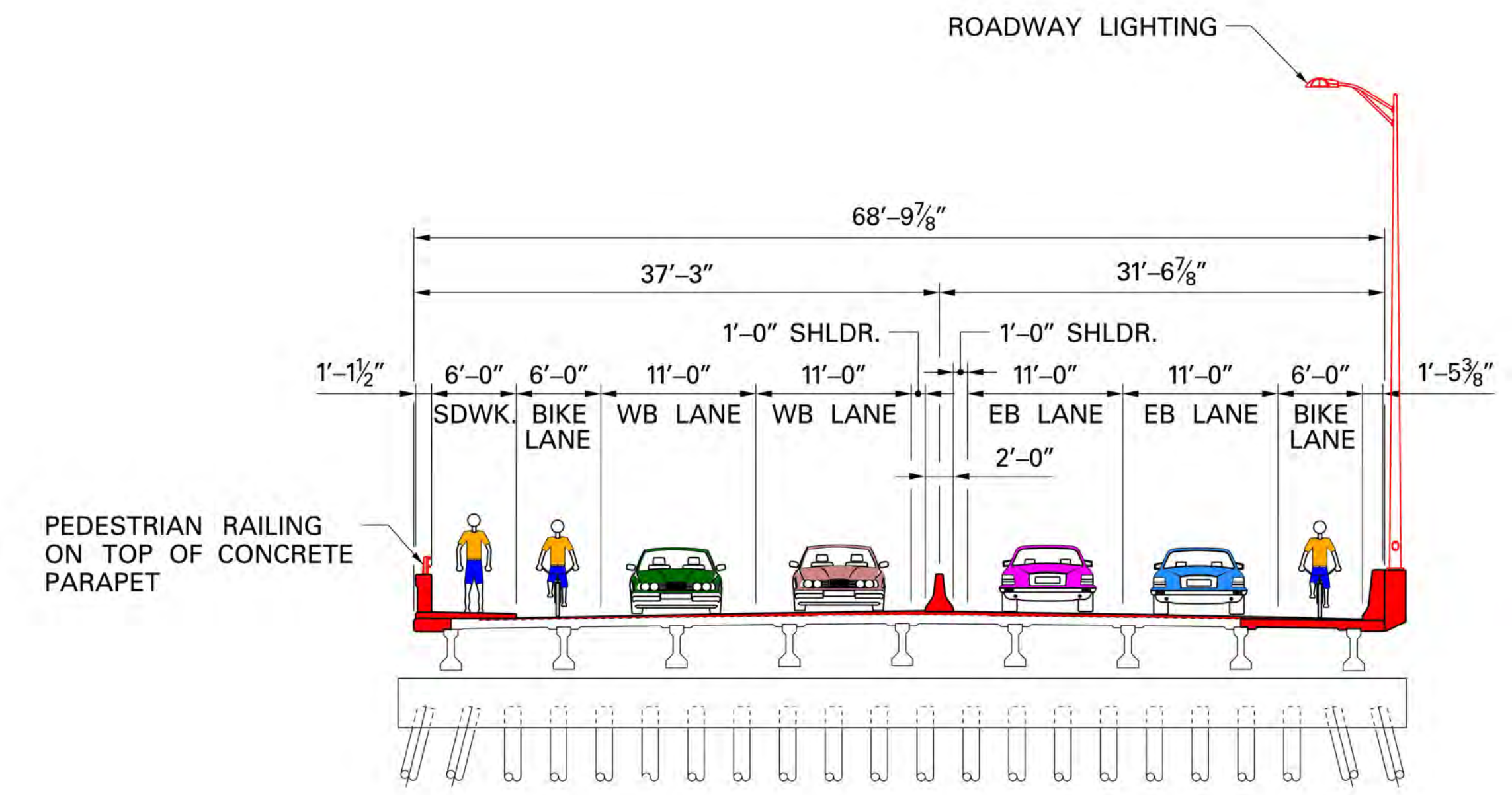
PROPOSED TRESTLE BRIDGES (LOOKING EAST)
