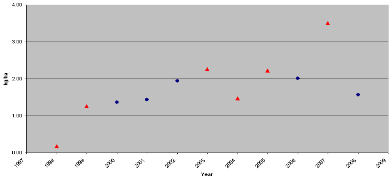
Figure 7 Ammonium (NH 4 ) NADP/NTN Site NJ00 (Edwin B. Forsythe National Wildlife Refuge) Annual Wet Depositions (1998 - 2008) Kilograms Per Hectare (kg/ha)
