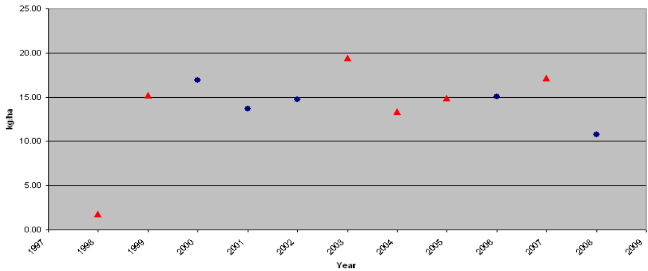
Figure 6 Sulfate (SO 4 ) NADP/NTN Site NJ00 (Edwin B. Forsythe National Wildlife Refuge) Annual Wet Depositions (1998 - 2008) Kilograms Per Hectare (kg/ha)
