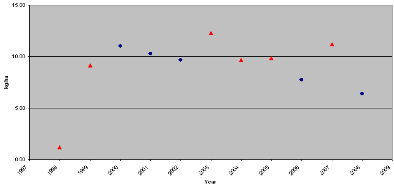
Figure 8 Nitrate (NO 3 ) NADP/NTN Site NJ00 (Edwin B. Forsythe National Wildlife Refuge) Annual Wet Depositions (1998 - 2008) Kilograms Per Hectare (kg/ha)
