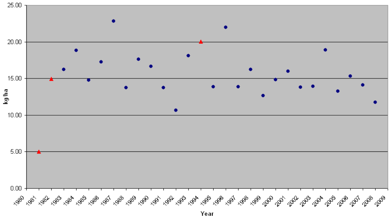
Figure 5 Nitrate (NO 3 ) NADP/NTN Site NJ99 (Washington Crossing State Park) Annual Wet Depositions (1981 - 2008) Kilograms Per Hectare (kg/ha)
