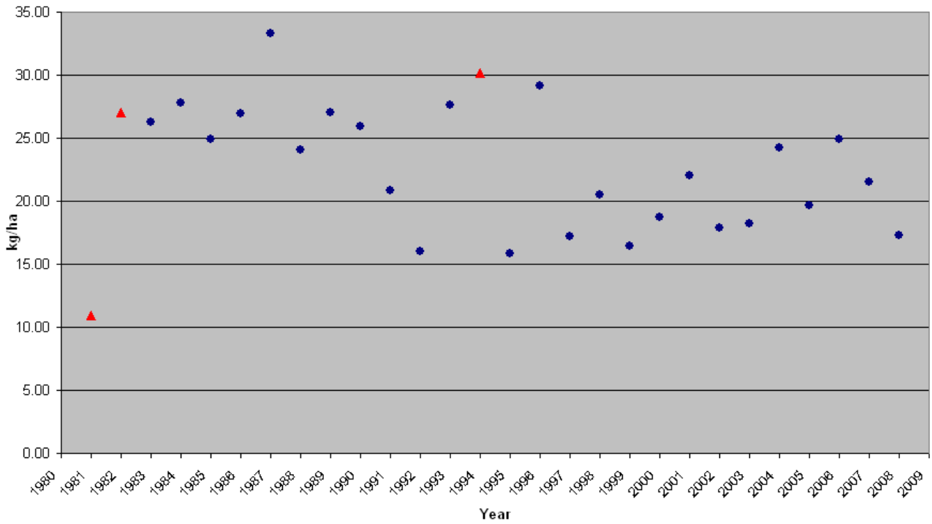
Figure 3 Sulfate (SO 4 ) NADP/NTN Site NJ99 (Washington Crossing State Park) Annual Wet Depositions (1981 - 2008) Kilograms Per Hectare (kg/ha)
