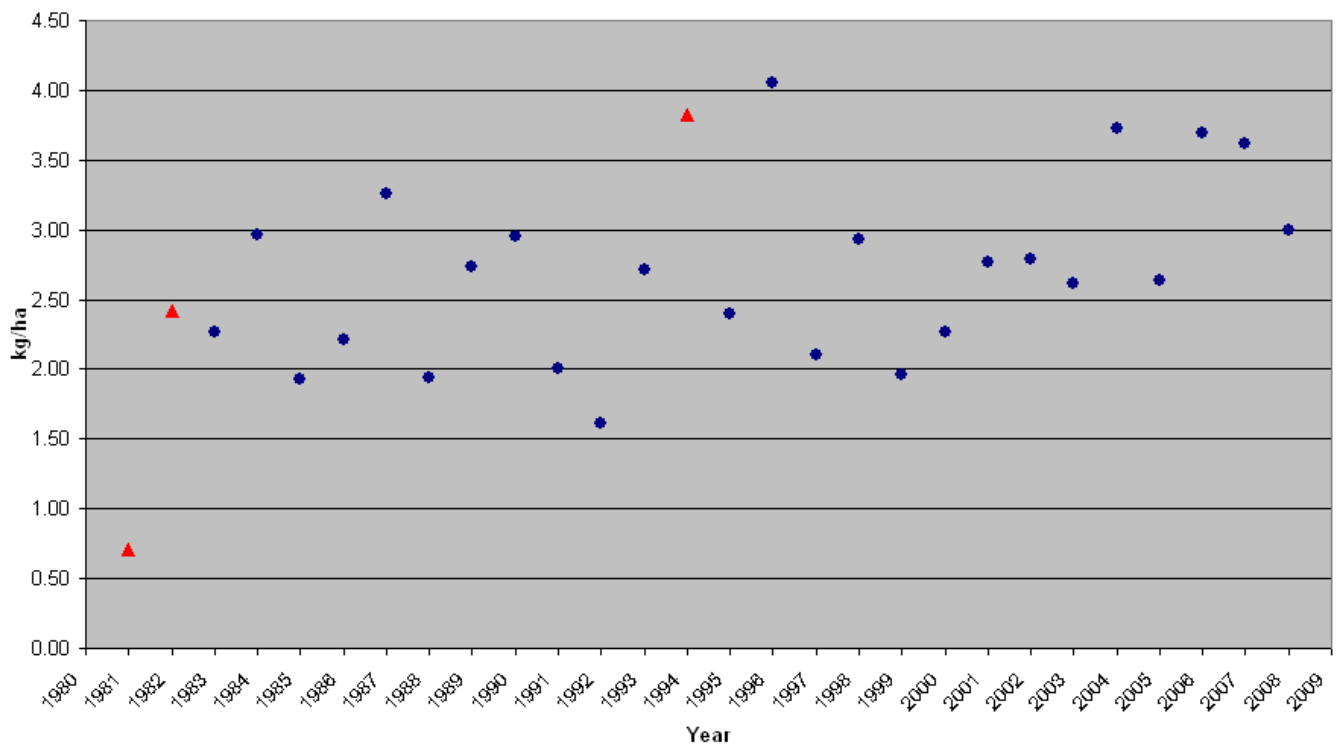
Figure 4 Ammonium (NH 4 ) NADP/NTN Site NJ99 (Washington Crossing State Park) Annual Wet Depositions (1981 - 2008) Kilograms Per Hectare (kg/ha)
