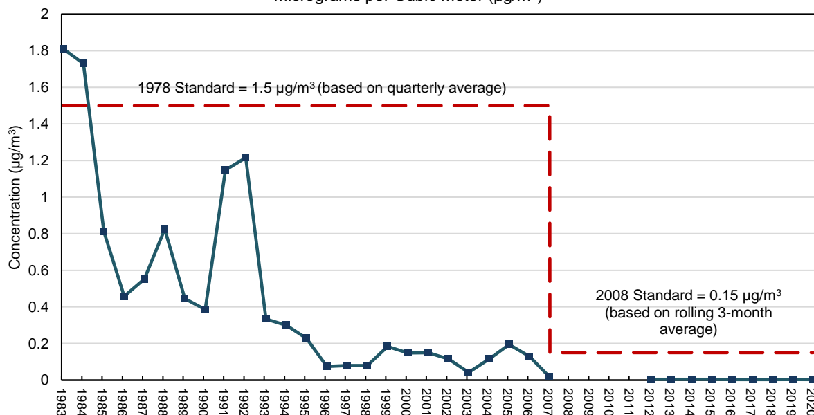
Figure 9-2 Statewide New Jersey Lead Trend, 1983-2020 Highest 3-Month Averages
