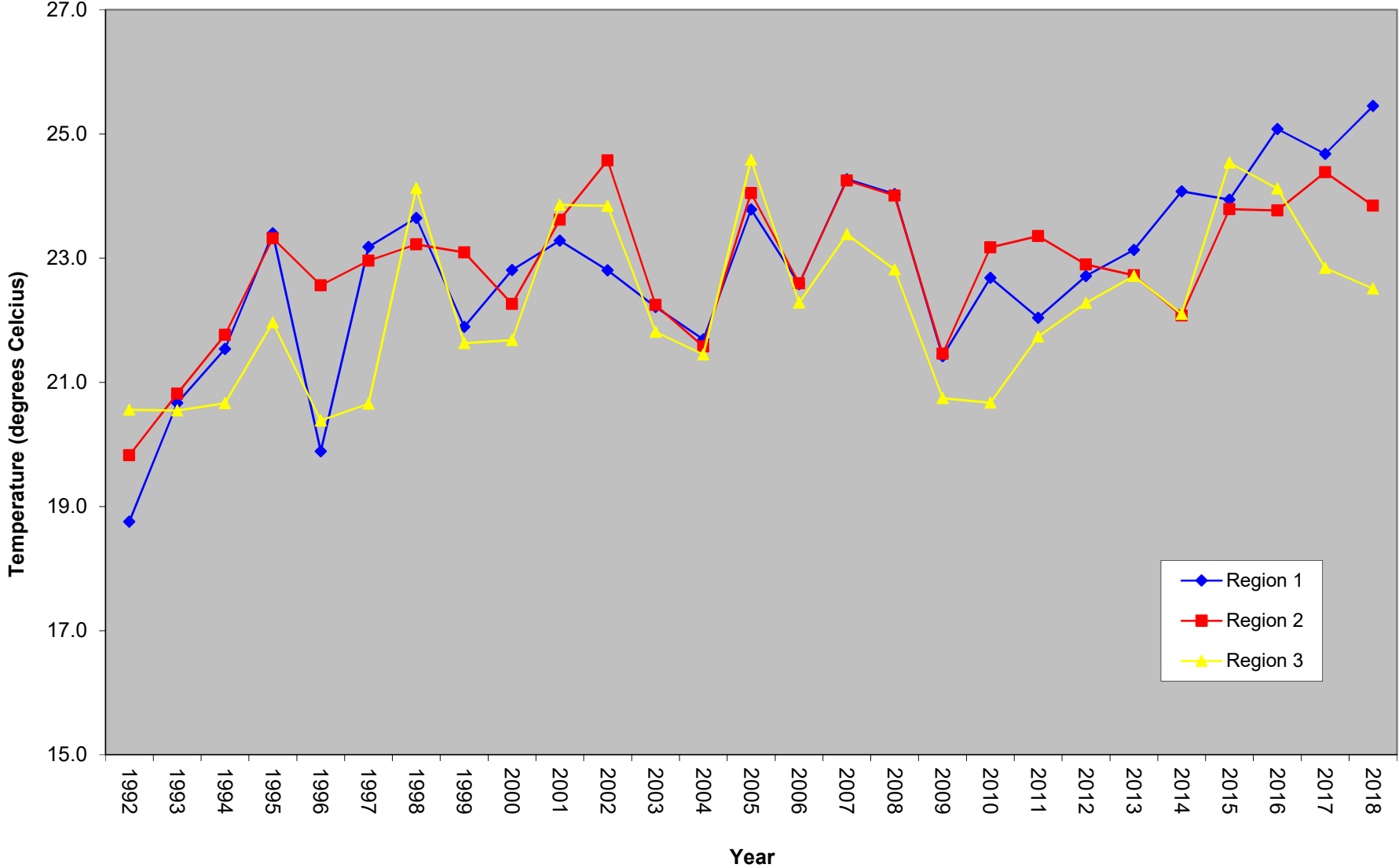
Delaware River Average Water Temperature
