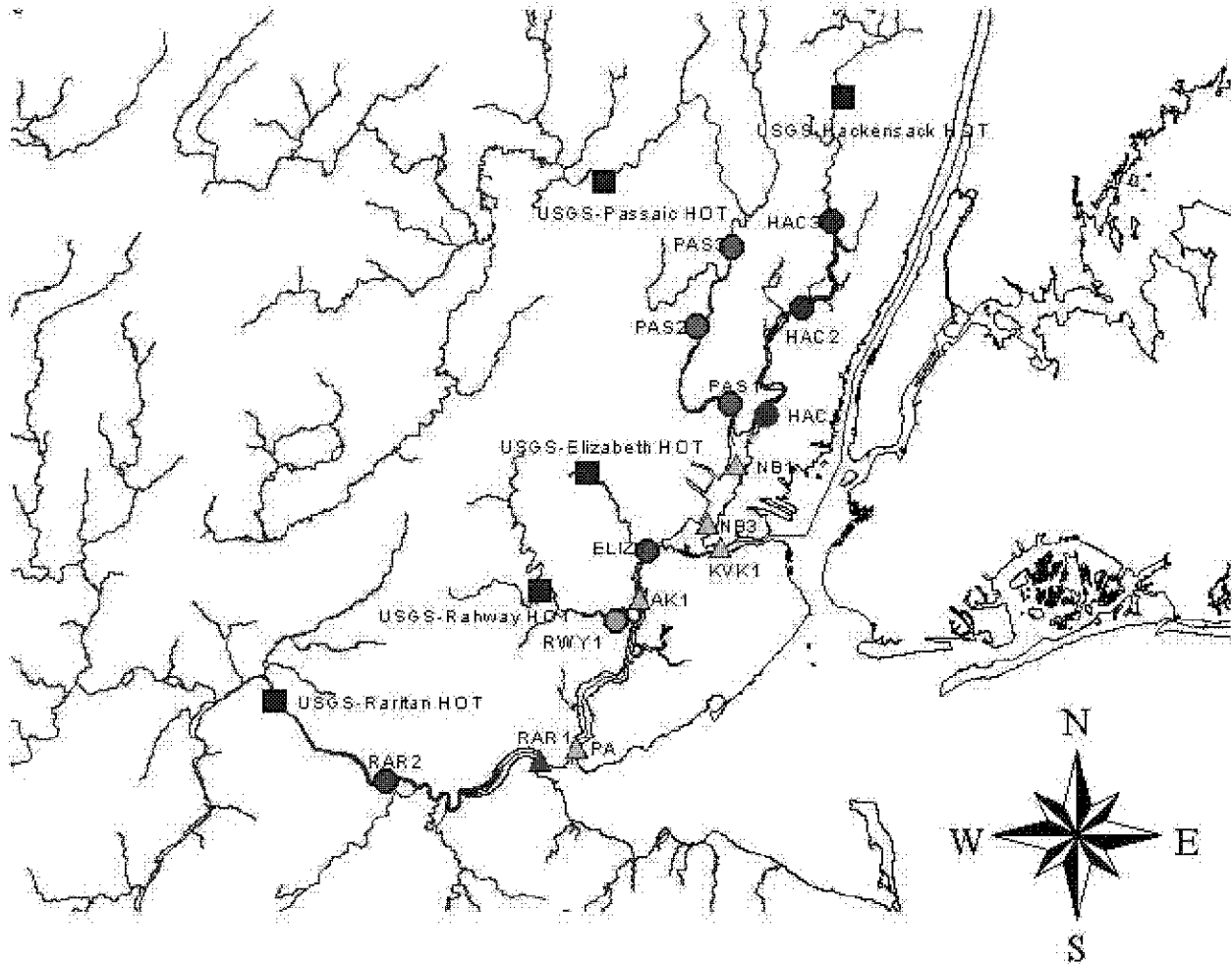
Figure1: Approximate locations of the NJTRWP water quality sampling stations.
