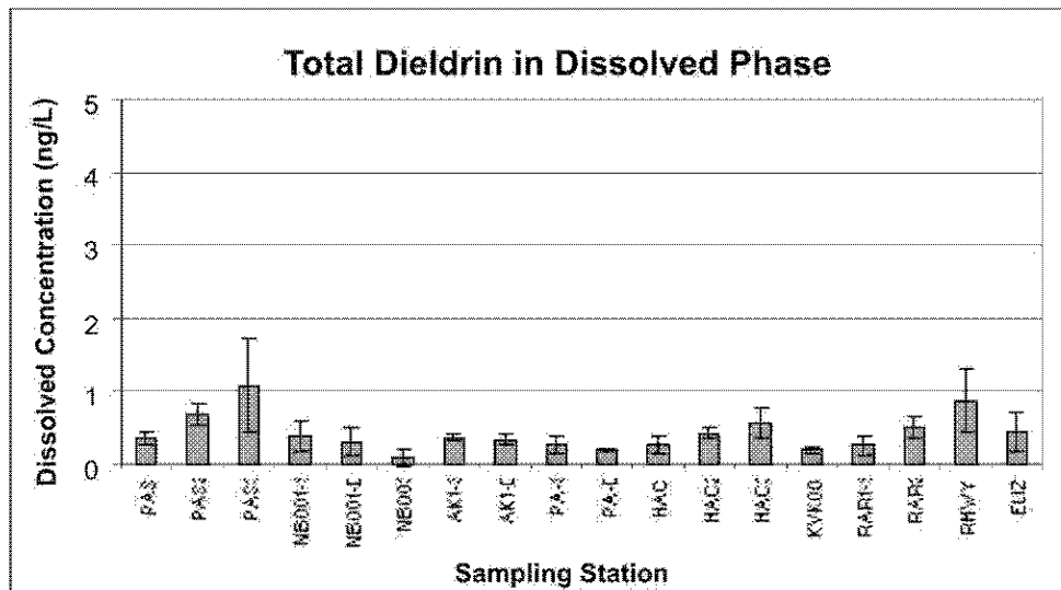
Figure 66: Mean ± standard deviation dissolved Dieldrin concentration (ng/L) at each sampling station.
