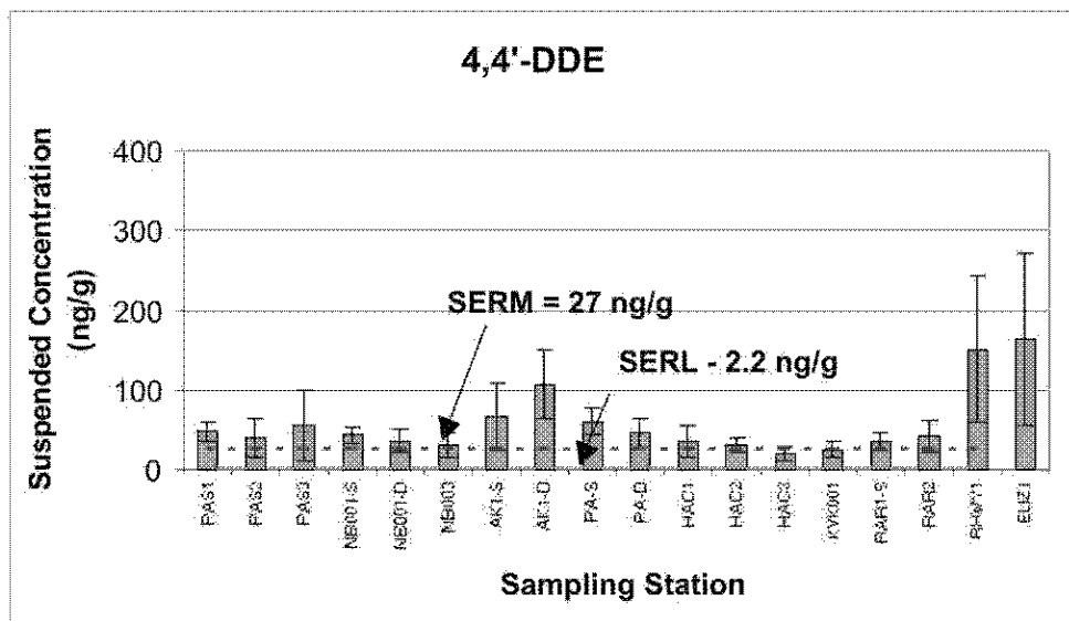
Figure 70: Mean \pm standard deviation suspended sediment 4,4'-DDE concentration (ng/g) at every sampling station.
