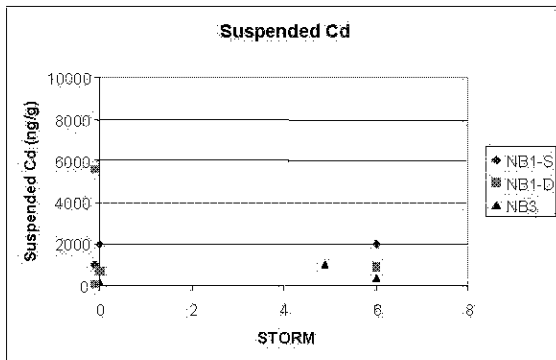
Figure 28(a-e): Dissolved Cd (ng/L), Total Cd (ng/L) and Suspended Sediment Cd (ng/g sed) Concentrations – Wet and Dry Sampling Events. (a) Passaic River, (b) Haekensack River, (c) Newark Bay, (d) Elizabeth and Rahway Rivers, (e) Raritan River.
