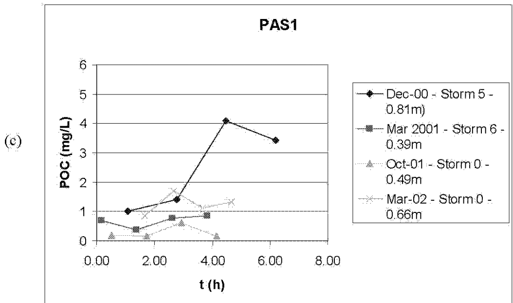
Figure 12: (a) SS, (b) DOC and (c) POC measurements at the PAS1 sampling station
