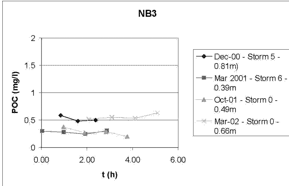
Figure 20: (a) SS, (b) DOC and (c) POC measurements at the NB3 sampling station
