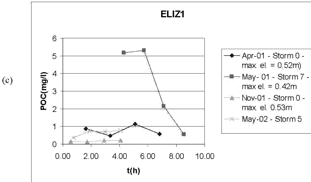
Figure 21: (a) SS, (b) DOC and (c) POC measurements at the ELIZ 1 sampling station
