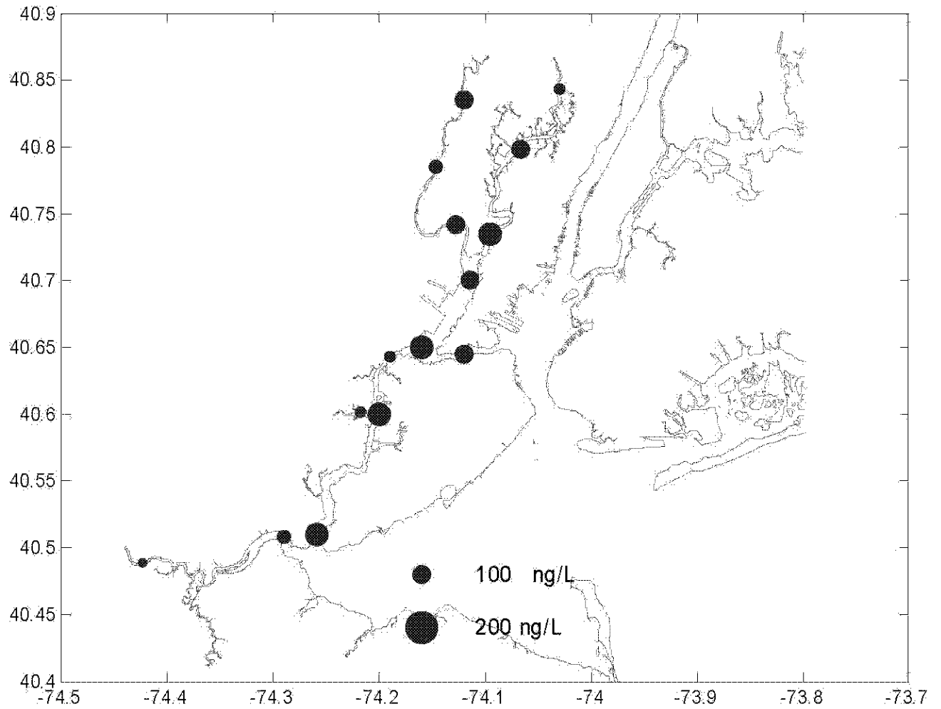
Figure 27: Mean Dissolved Cd concentration at each sampling station (ng/L).
