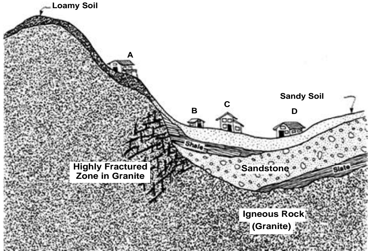
Figure 1. Illustration of a hypothetical geological region containing some igneous, metamorphic, and sedimentary rocks. The granite is high in uranium, whereas the concentrations of uranium in the other rock materials are lower. Four houses are situated in the region (A through D). Loamy soil is found on the main hill, and contains a mixture of sand, silt, and clay. Sandy soil covers the valley bottom. The sandstone contains an abundance of shell fossils from marine organisms.
