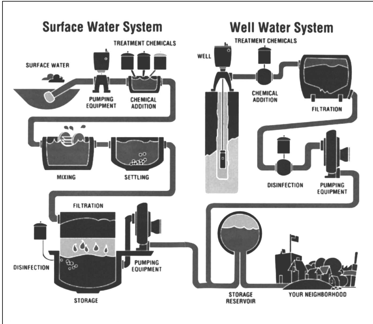
Figure 3: Example of Drinking Water Treatment
