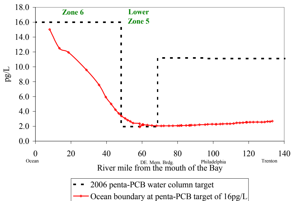
Figure 13: Simulation results under the loading conditions developed up to Step 3 and assigned ocean boundary at the penta-PCB water quality target of 16pg/L.
