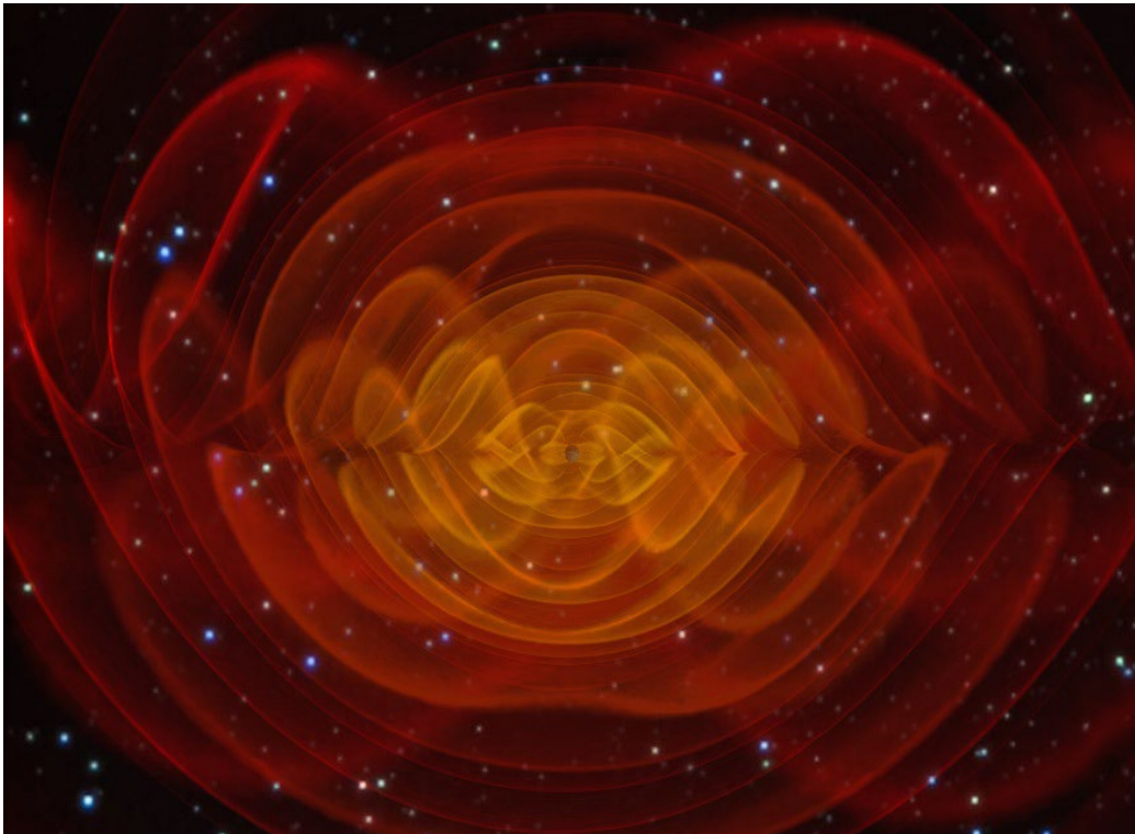
Image from NASA's Doing Astronomy With our Eyes Closed
