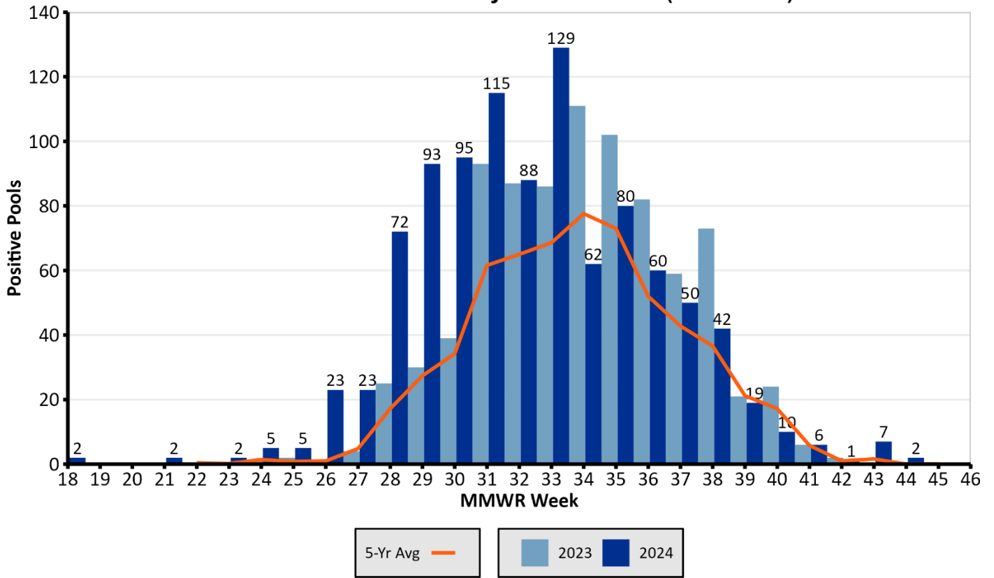
WNV Positive Pools by MMWR Week (2023-2024)
