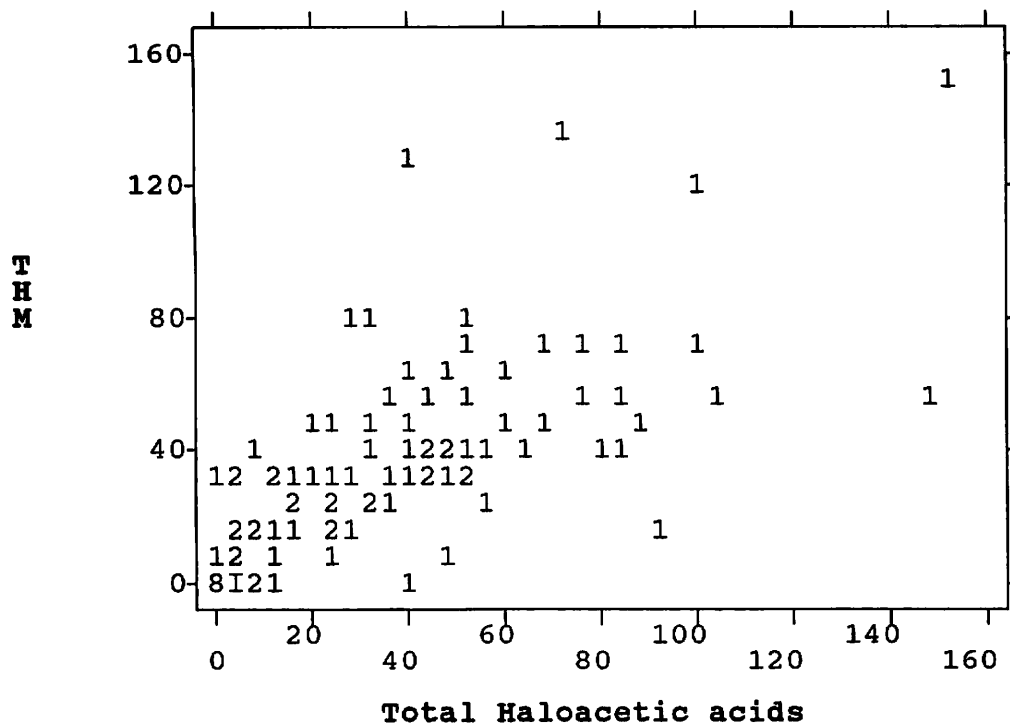
Plot of Total Trihalomethanes with Total Haloacetic Acids among Controls (mixed and surface water sources only, N = 111)
