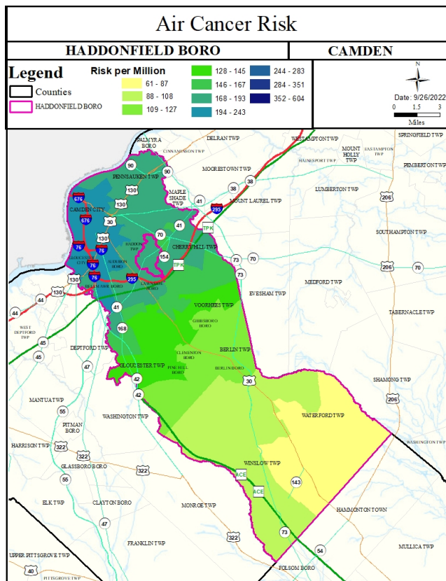
This map shows the cancer risk estimates for Haddonfield Borough in Camden County. Overall, Haddonfield Borough has a mean cancer risk of 177 in a million.
