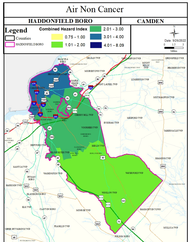
This map shows the noncancer risk for Haddonfield Borough in Camden County. Overall the noncancer risk is 2.8.
