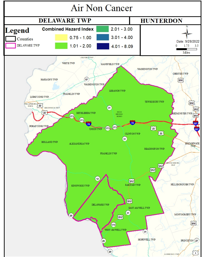
This map shows the noncancer risk for Delaware Township in Hunterdon County. Overall the noncancer risk is 1.4.
