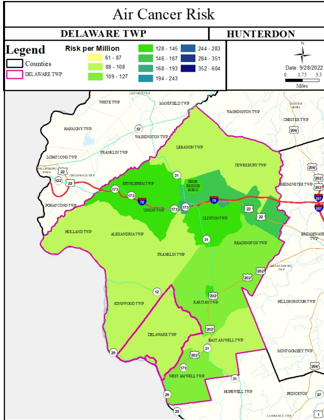
This map shows the cancer risk estimates for Delaware Township in Hunterdon County. Overall, Delaware Township has a mean cancer risk of 98 in a million.
