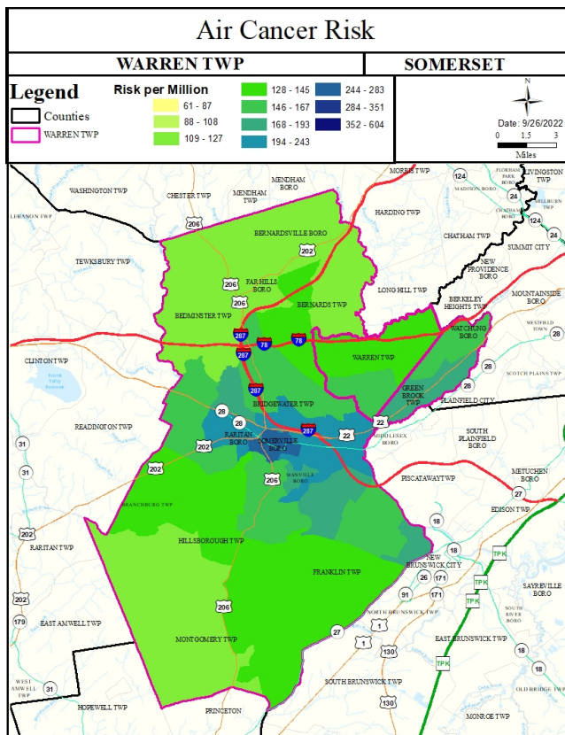
This map shows the cancer risk estimates for Warren Township in Somerset County. Overall, Warren Township has a mean cancer risk of 147 in a million.
