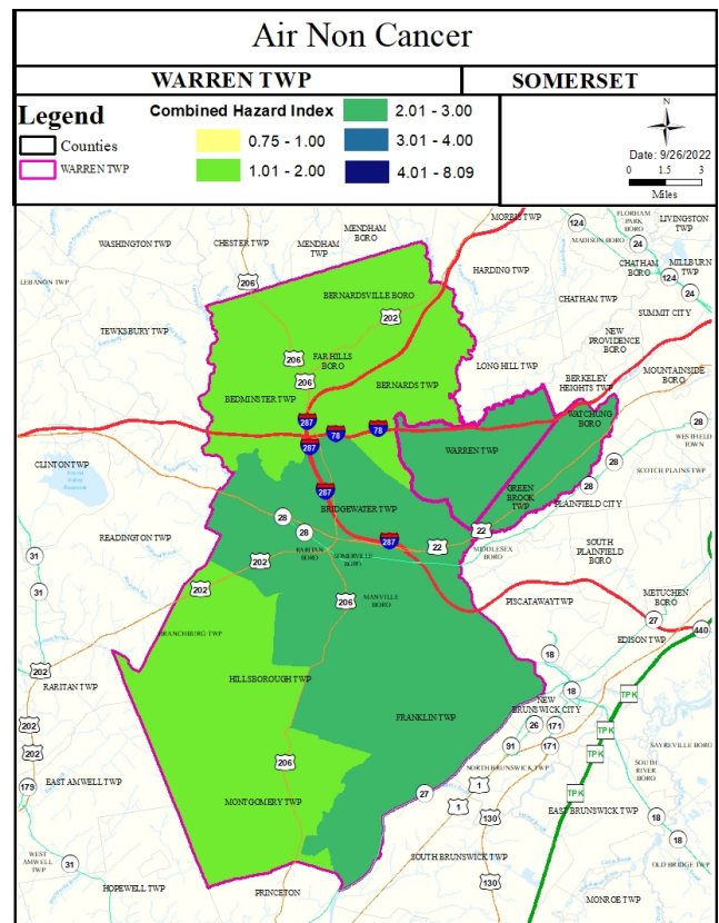
This map shows the noncancer risk for Warren Township in Somerset County. Overall the noncancer risk is 2.2.
