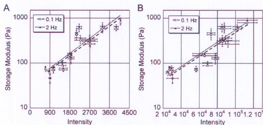
Figure 6. Correlation of average storage modulus ( \pm std err) with average fluorescence intensity ( \pm std err) measured with epifluorescence microscopy (A) or spectrofluorimetrically (B) for 0.1 and 2 Hz. In all cases, strong, exponential correlations were observed, indicating that stiffness can be assayed optically following appropriate calibration. Increasing frequency shifted the correlation curve to the left.
