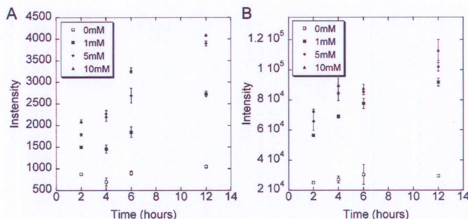
Figure 5. Fluorescence intensity (average \pm std err) of genipin-crosslinked collagen measured using (A) epifluorescent microscopy (590 nm excitation, 630 nm emission) and (B) spectrofluorimetrically (590 nm excitation, 645 nm emission). For both, the intensity of fluorescence emission increased significantly with genipin concentration and duration of incubation ( p < 0.001 ). Post hoc analysis (Fisher's LSD test) revealed significant differences among all pairwise comparisons of concentrations except 5 mM versus 10 mM (max p = 0.199 ) and among all pairwise comparisons of duration except 4 h versus 6 h ( p = 0.240 ).
