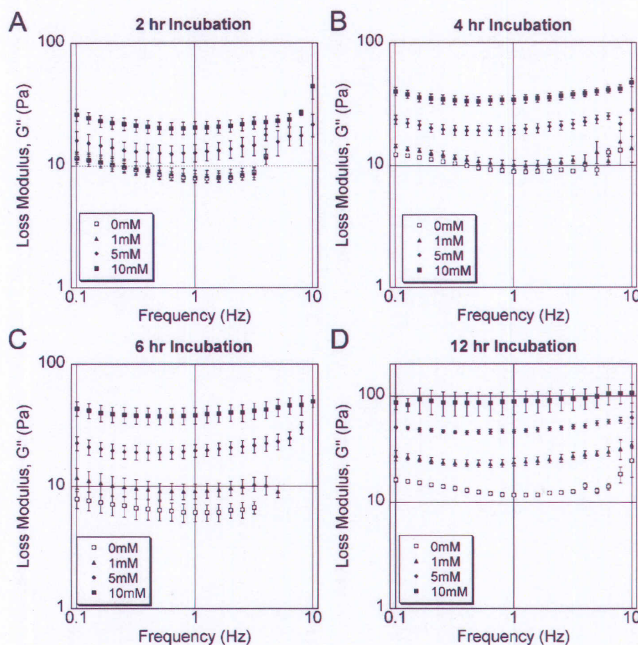
Figure 3. Loss moduli following parallel plate rheometry. A: 2-h incubation; (B) 4-h incubation; (C) 6-h incubation; (D) 12-h incubation. Results are average \pm std err. Loss modulus tended to decline with frequency and then rise concurrent with the decline in storage modulus at higher frequencies. Both genipin concentration and the duration of incubation significantly affected the storage modulus.
