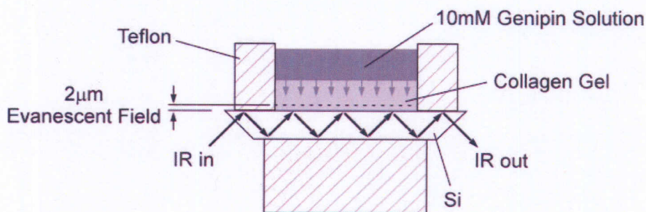
Figure 1. ATR setup showing genipin deposition for time-resolved study. Genipin solution (10 mM) is deposited on top of and diffuses through the collagen gel. A 2- \mu m region of the collagen gel is probed by the IR evanescent field during genipin-mediated crosslinking. The genipin solution (10 mM) and collagen crosslinked with genipin for 12 h are probed in a similar way.
