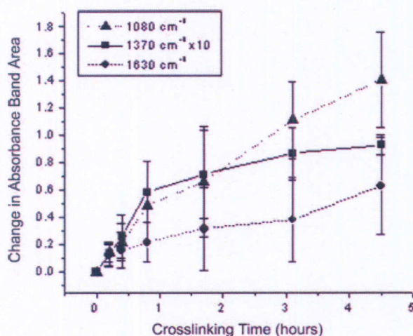
Figure 8. Changes in absorbance band areas versus crosslinking time for some of the highlighted bands in Figure 7: two genipin bands (triangle, 1080 \text{cm}^{-1} and circle, 1630 \text{cm}^{-1} ), and a new genipin-to-collagen crosslinking feature (square, 1370 \text{cm}^{-1} ). To allow all spectra to be viewed on a common plot, values of smaller band areas were scaled by a constant, as indicated in the inset. Crosslinking time began (at t = 0 ) when genipin reached the bottom of the collagen gel at the interface with silicon. Error bars combine two sources of errors: (1) baseline selection for area calculations, and (2) reproducibility of runs. End point area values of each band for different runs were normalized to a common value due to variation in absolute absorbance area possibly caused by variation in collagen density among samples.
