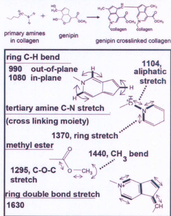
Figure 9. Description of the modes marked in the spectra of Figure 7.
