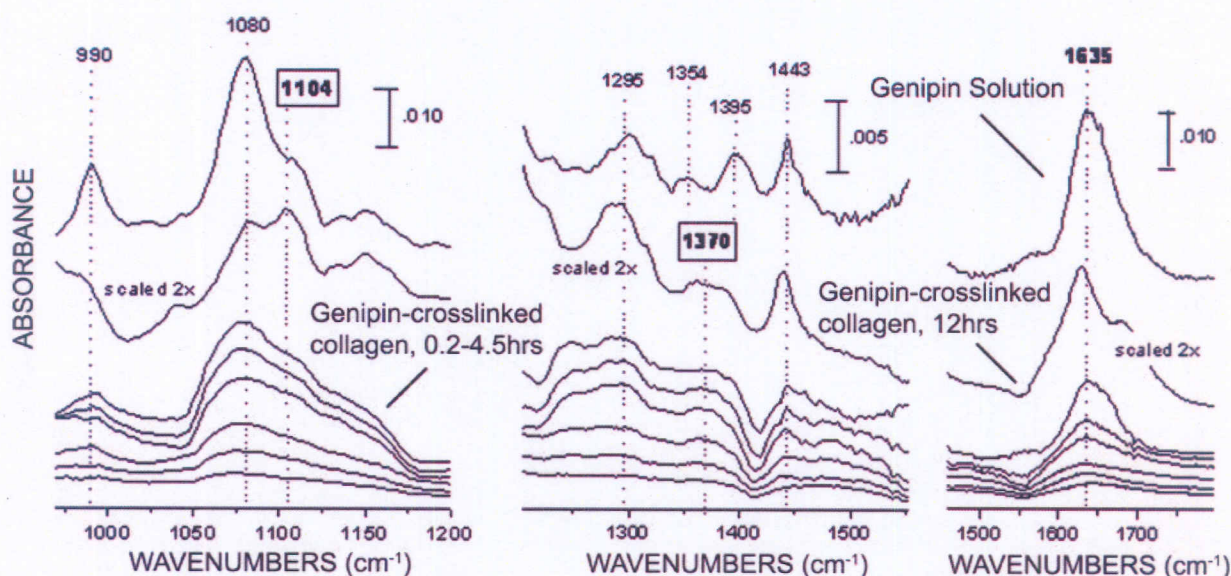
Figure 7. IR Absorbance spectra of 10 mM genipin referenced to a spectrum of pure water (top); collagen after 12 h of crosslinking with 10 mM genipin and extensive rinsing, referenced to a spectrum of uncrosslinked collagen (second from top, scaled 2 \times ) and collagen crosslinked with 10 mM genipin in situ , 0.2, 0.4, 0.8, 1.7, 3.1, and 4.5 h after adding genipin, referenced to the initially genipin-free collagen gel (bottom). Several spectral features that are present in the genipin solution alone, and/or the crosslinked and rinsed collagen are seen to evolve during the in situ crosslinking.
