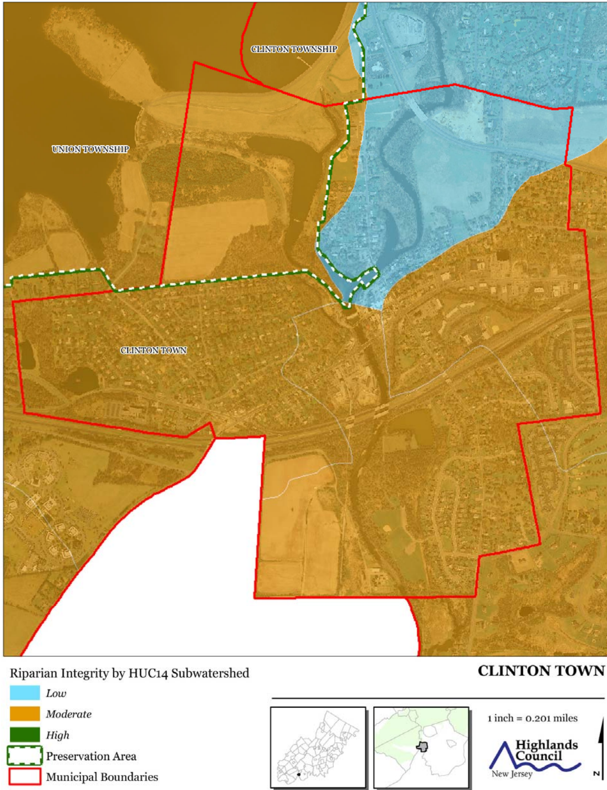
Figure 9. Riparian Integrity
