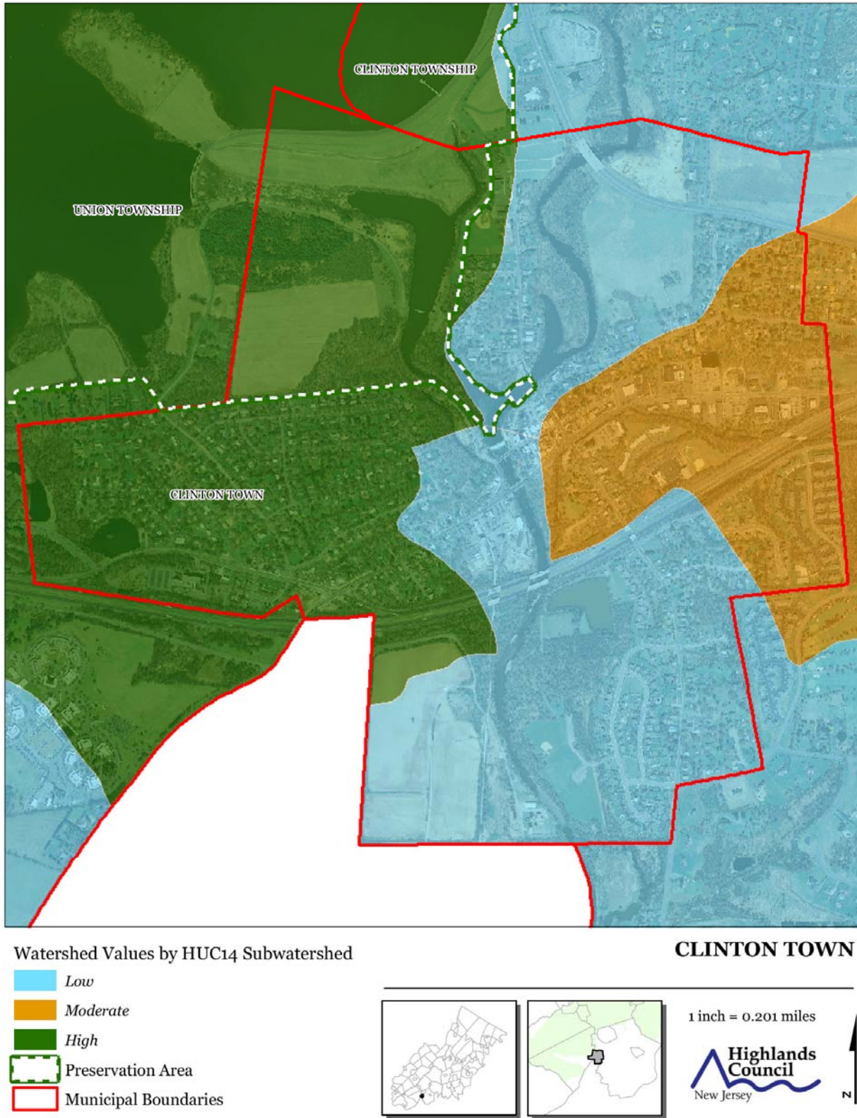
Figure 8. Watershed Values
