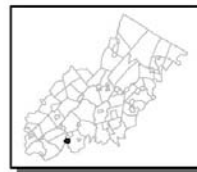
Figure 14. Carbonate Rock Areas
