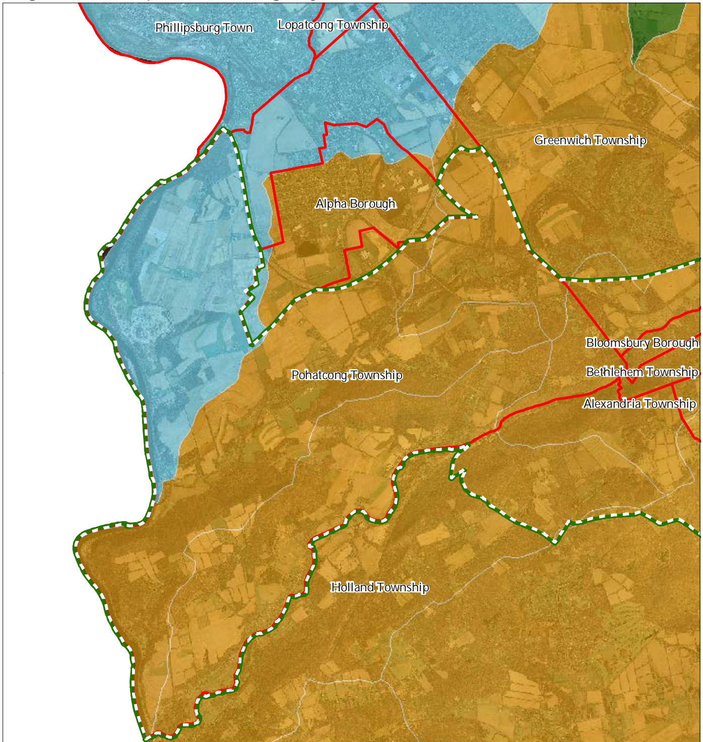
Figure 10: Riparian Integrity
