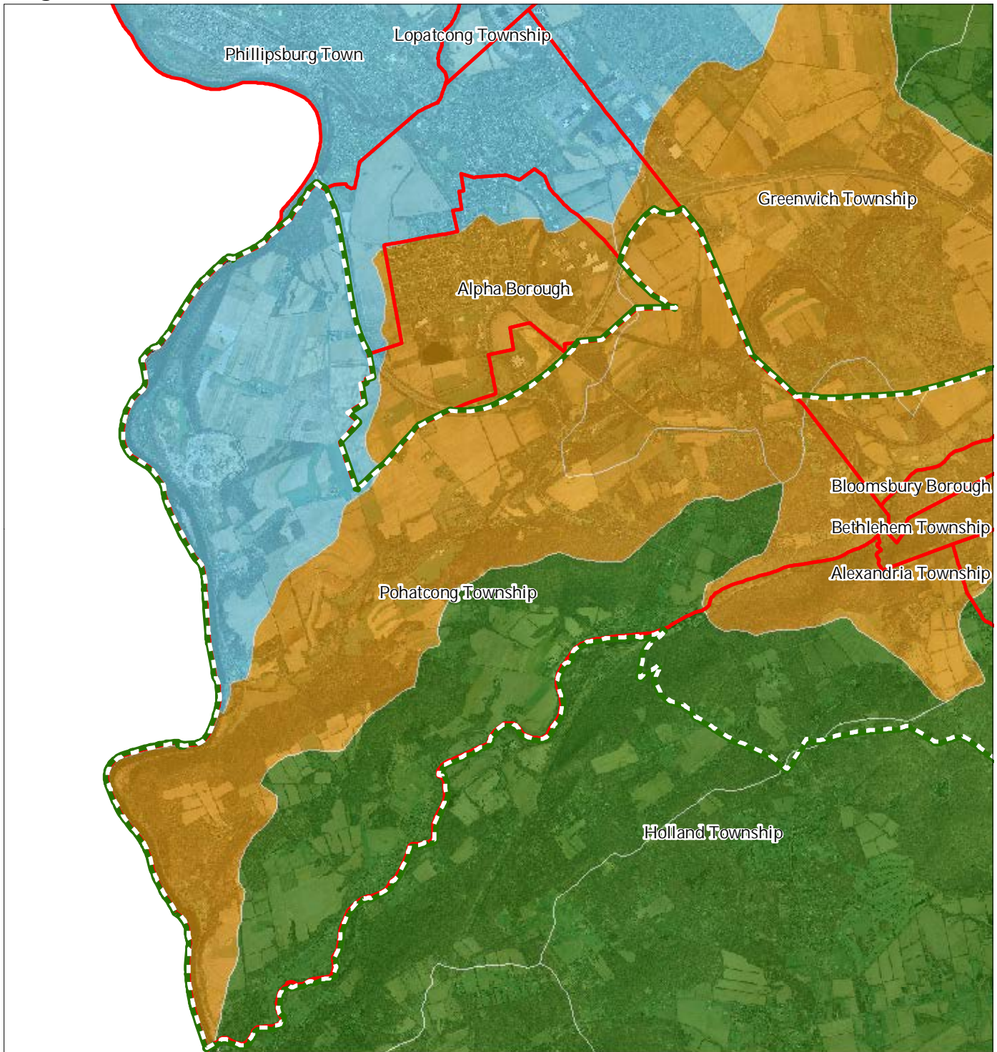
Figure 9: Watershed Values
