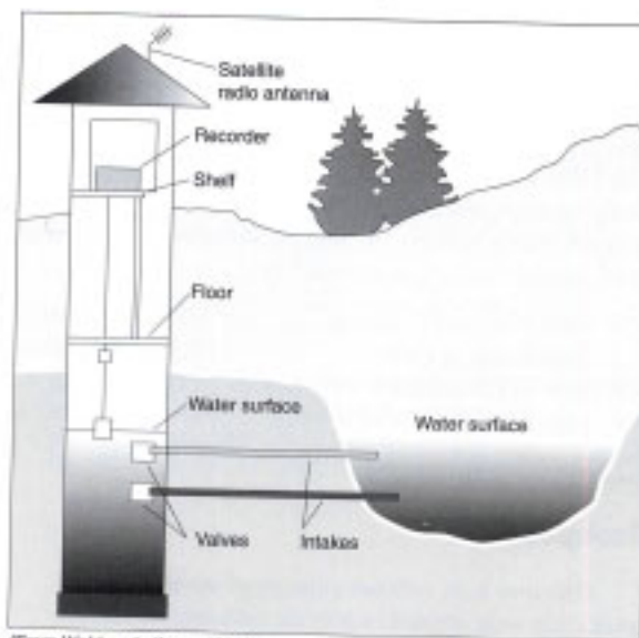
Figure 3. Schematic drawing of a stilling well and shelter at a stream-gaging station.
