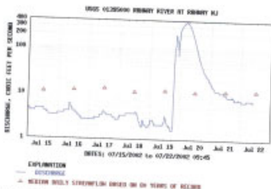
Figure 6. Example of an actual streamflow hydrograph that can be viewed and printed from the "real-time" network web page.
