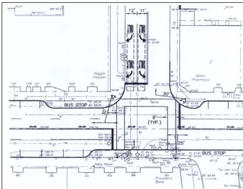
Figure 22 Cedar Lane and Garrison Avenue Bus Bulb.
