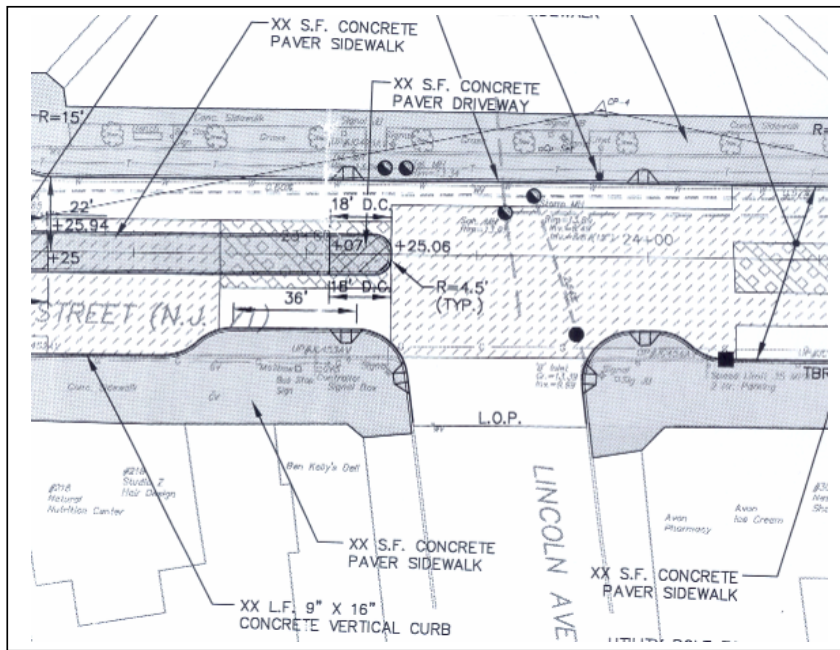
Figure 19. Main Street and Lincoln Avenue Bus Bulb.
