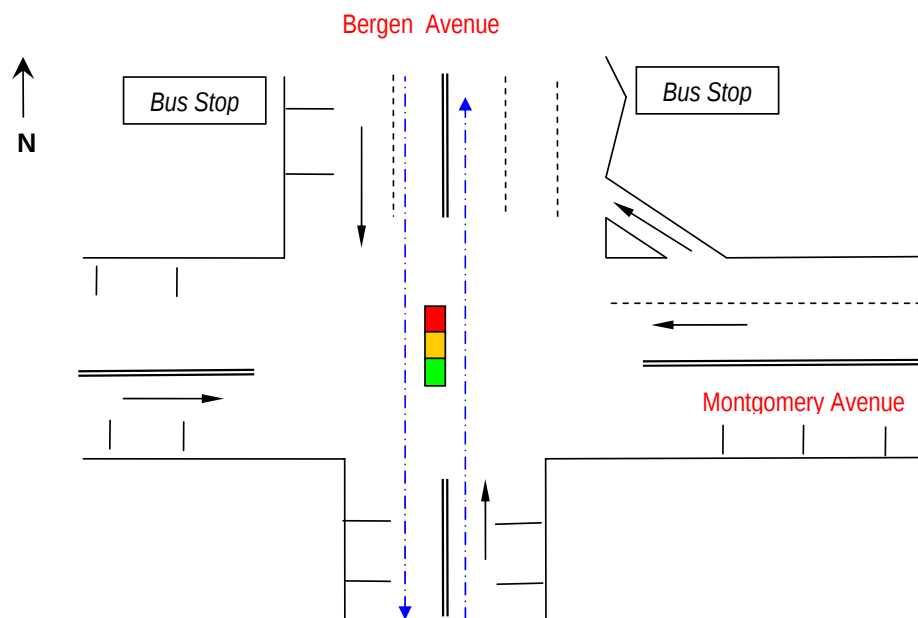
Figure 37. Bergen Avenue and Montgomery Avenue.
