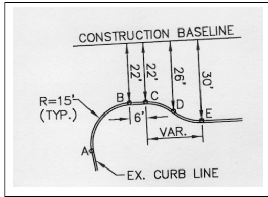
Figure 18. Typical Pedestrian Bulbout on Route 71.
