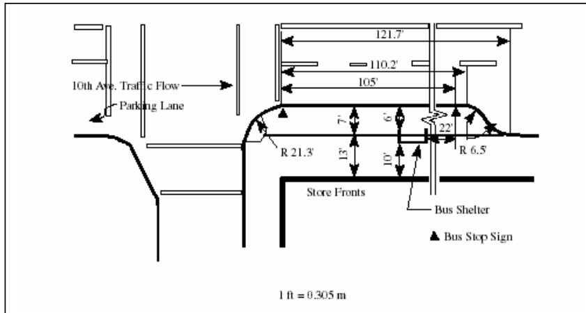
Figure 4. Farside Bus Bulb Location (Source: TCRP 65).
