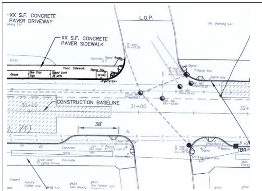
Figure 20. Main Street and Sylvania Avenue Bus Bulb.
