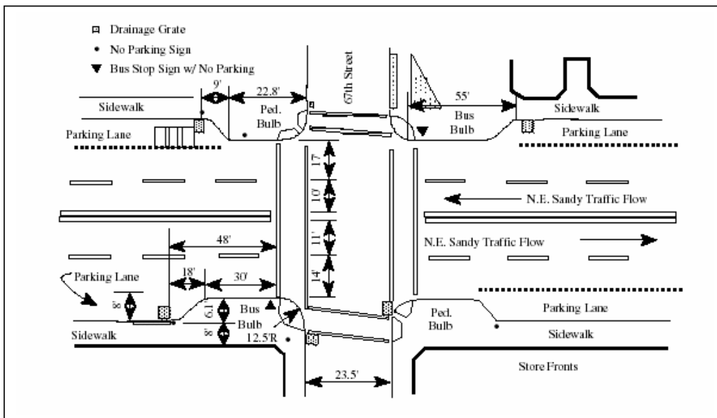
Figure 3. Nearside Bus Bulb Location (Source: TCRP 65).
