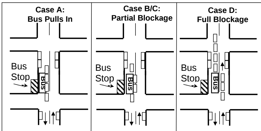
Figure 38. Re-Entry Delay Measurement Cases
