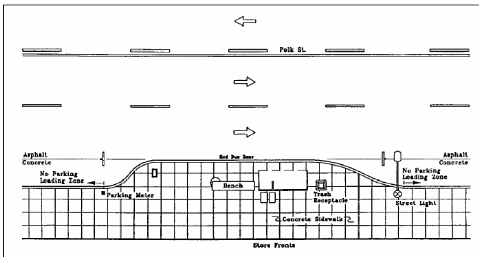
Figure 5. Midblock Bus Bulb Location (Source: TCRP 65).
