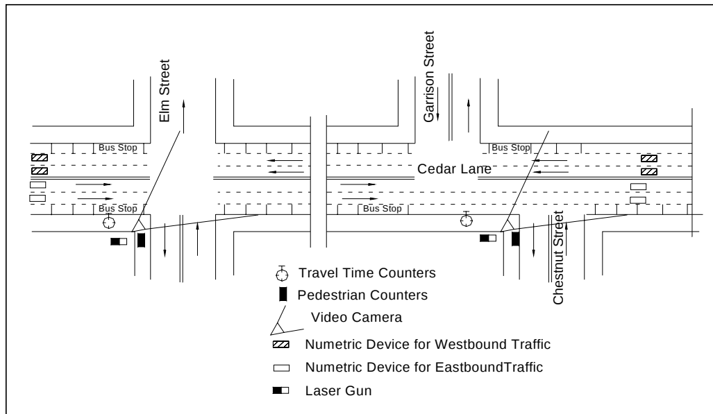
Figure 23. Layout of Field Work.
