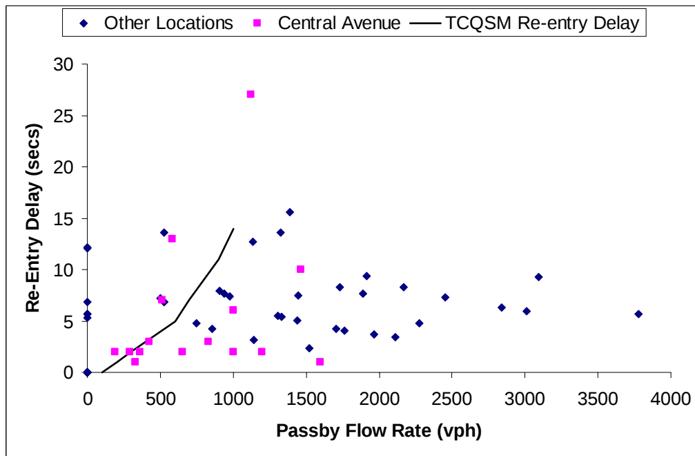
Figure 39. Re-Entry Delay vs. Passby Flow Rate.
