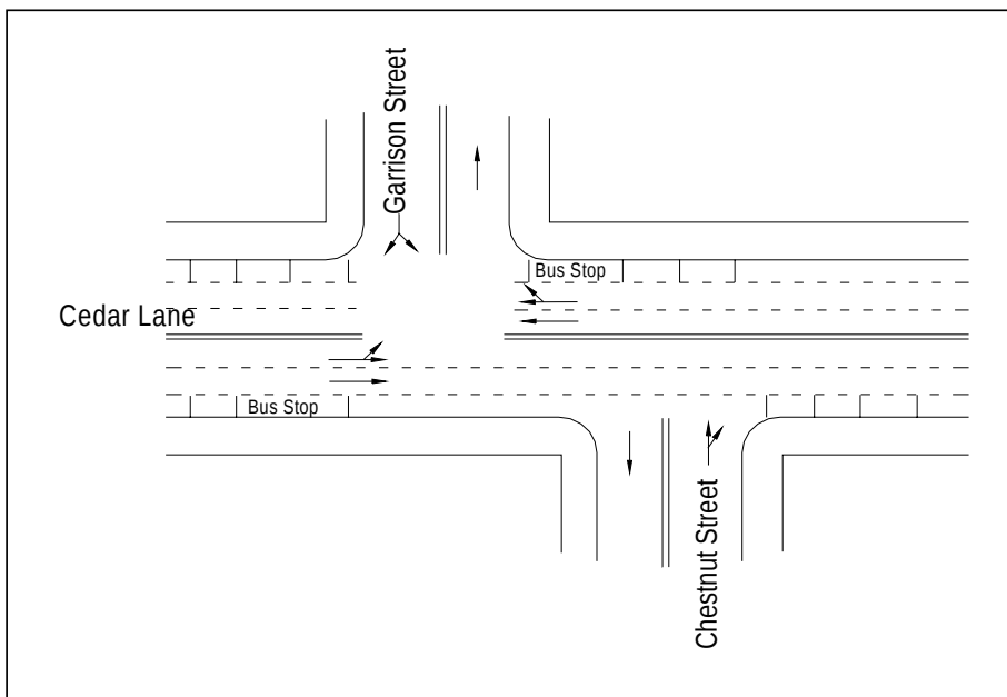
Figure 28. Geometry and Lane Configuration of Cedar Lane and Garrison Avenue.
