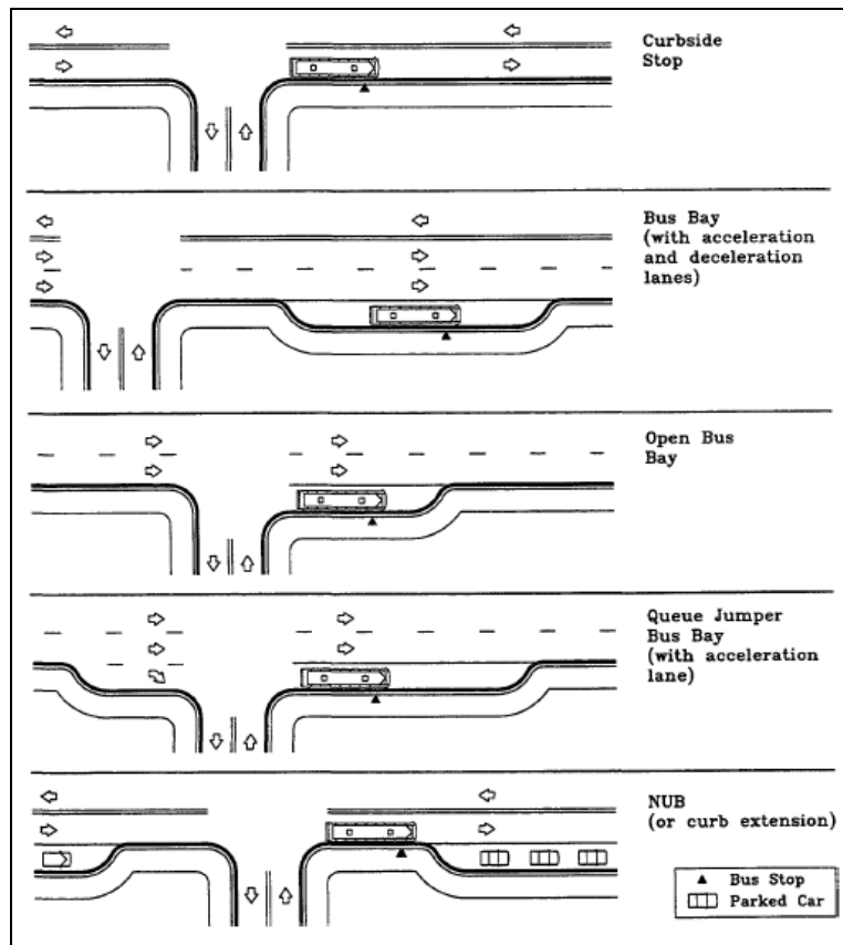
Figure 2. Alternative Bus Stop Design (Source: TCRP 65).
