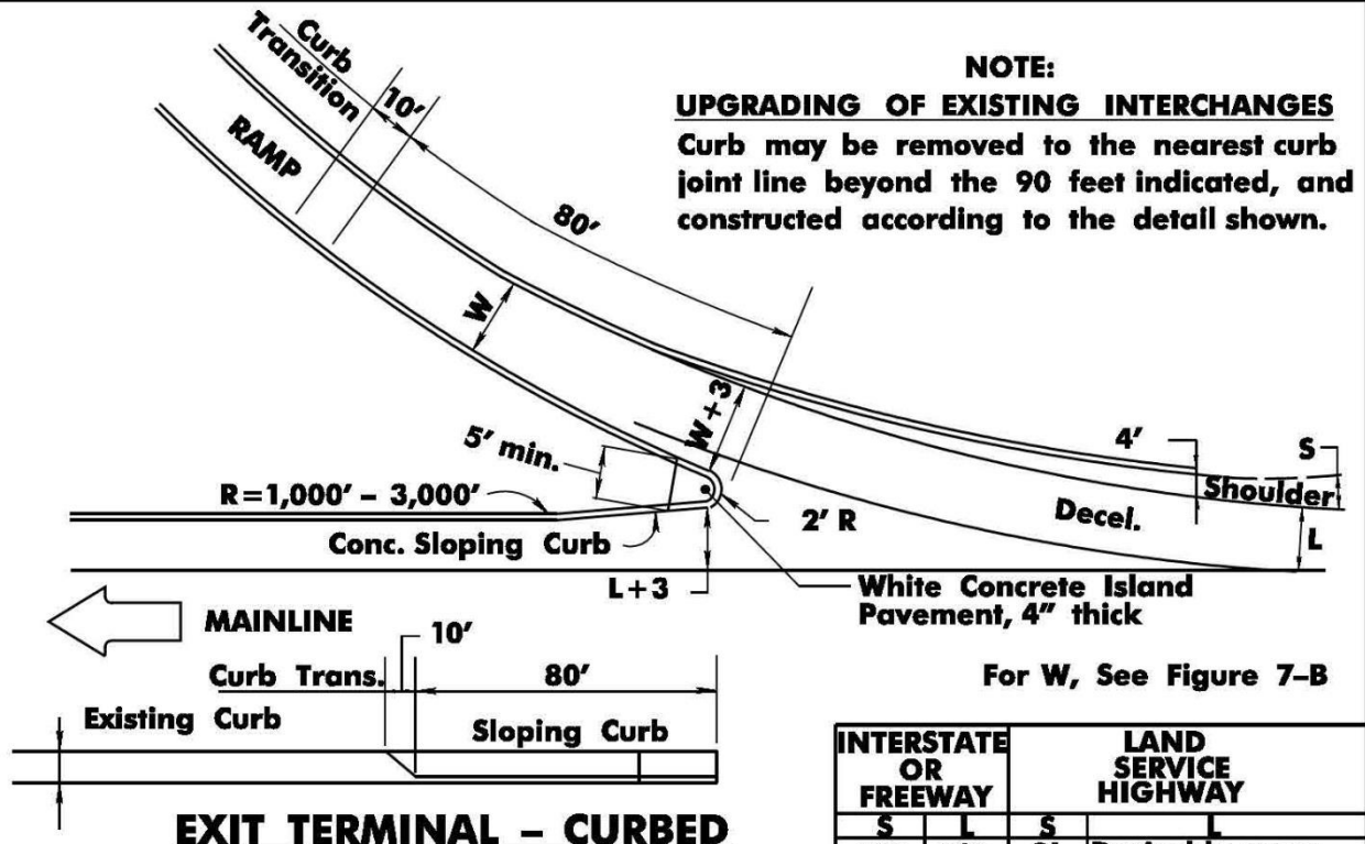
FIGURE 7-E: EXIT TERMINAL TREATMENT
