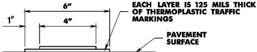
RUMBLE MARKING DETAIL
