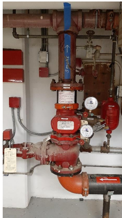
MOB Basement- Existing Backflow Preventor Valve
