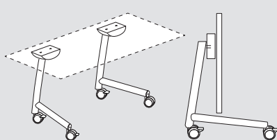
L-base with casters and Flip-Top mechanism
