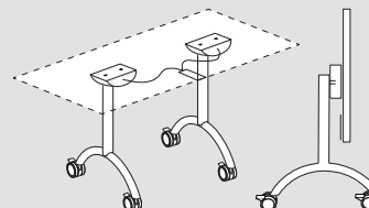
T-base with casters, Flip-Top mechanism and handle
