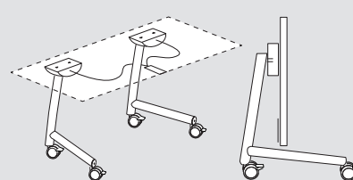
L-base with casters, Flip-Top mechanism and handle
